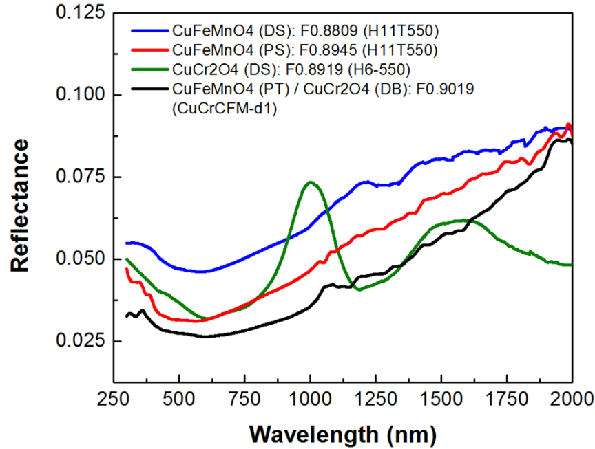
Fig. 16. Effect of porous layer structure and double layer on reflectance for SSC layers made of copper chromite particles and copper iron manganese particles. DS: dense single layer, PS: porous single layer, PT: porous top layer, and DB: dense bottom layer.
