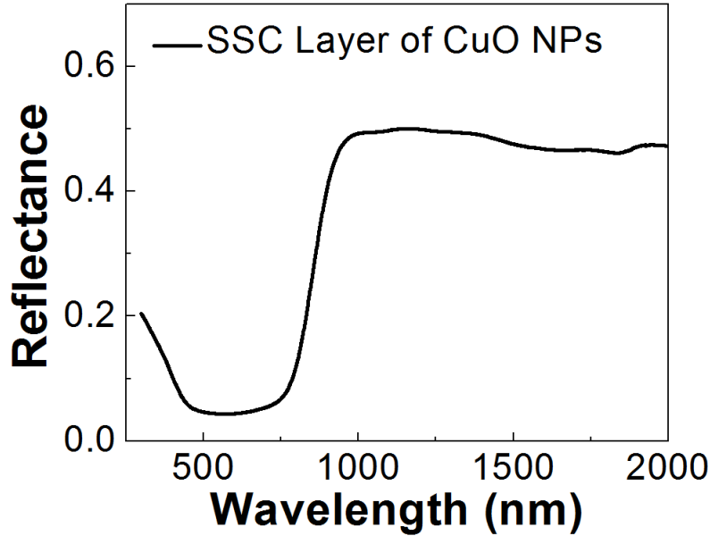
Fig. 27. Reflectance measured for SSC layer fabricated with CuO nanoparticles and annealed at 750°C/2h/air.
