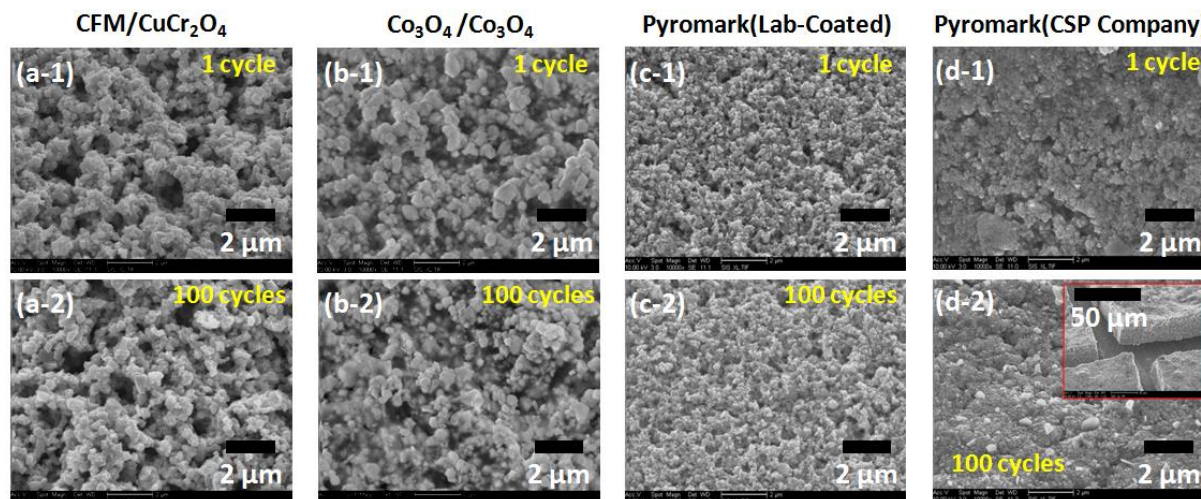
Fig. 25. SEM images showing surface morphologies of samples after 1 cycle and 100 cycles in thermal cycling (RT-750°C/air), and observed in tilted angle of 30 degree.
