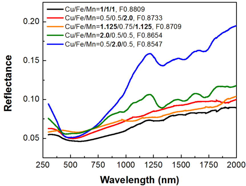
Fig. 8. Reflectance of SSC layers made of copper iron manganese particles with different atomic ratio (Cu/Fe/Mn). All samples had a dense single layer and were annealed with the condition of 750 °C/2h/air before reflectance measurement.
