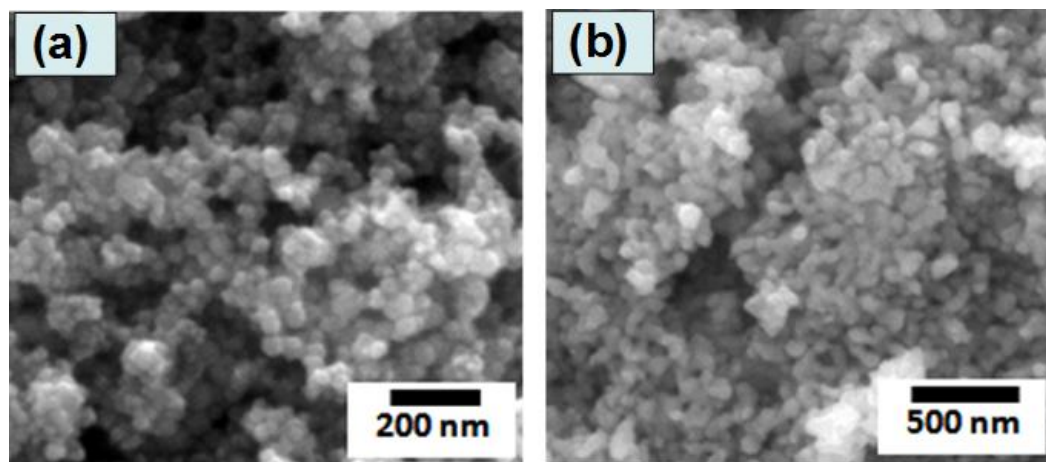
\text{Y}_2\text{O}_3 -coated \text{Fe}_3\text{O}_4 NPs
