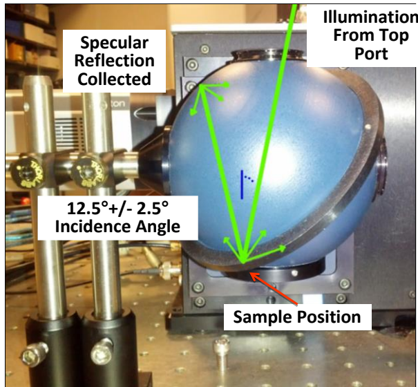
Fig. 17. Integration sphere configuration. Light is incident through top port onto sample resting at bottom port. Incidence is controlled to retain specular component of reflection.
