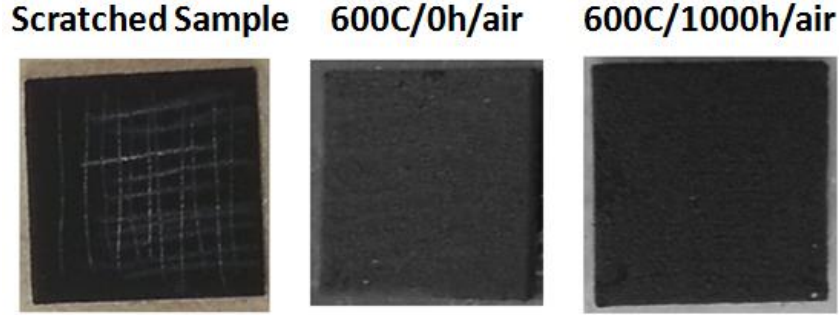
Fig. 30. Photos for (left) an impaired CuFeMnO 4 /CuCr 2 O 4 sample by scratching, (middle) a repaired sample by new spray coating on the scratched surface, and (right) a repaired sample after isothermal test.
