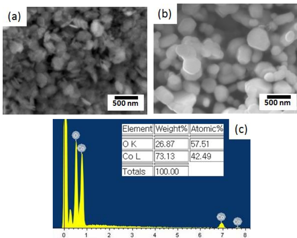
Fig.2. SEM images showing cobalt oxide nanoparticles (a) as-synthesized and (b) after annealing at 750 ^{\circ}\text{C} for 2 hr, and (c) EDX analysis results.
