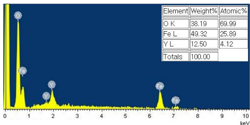
Fig. 11. EDX analysis result of \text{Fe}_3\text{O}_4 - \text{Y}_2\text{O}_3 core-shell nanoparticles.
