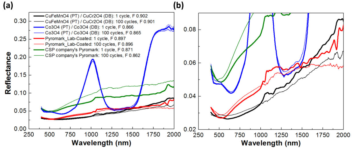
Fig. 23. Comparison of reflectance and FOM between 1-cycled samples and 100-cycled samples from RT to 750°C in air. (PT: porous top layer, DB: dense bottom layer)
