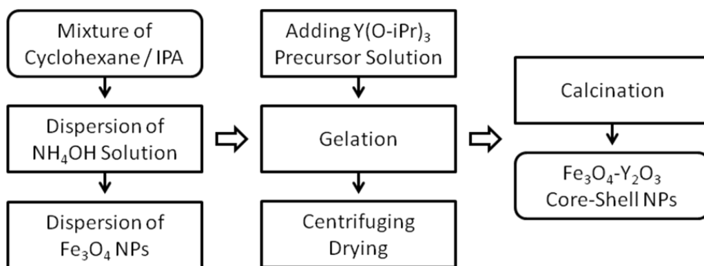
Fig. 9. The nano-shell synthesis procedure to make \text{Fe}_3\text{O}_4\text{-Y}_2\text{O}_3 core-shell NPs.
