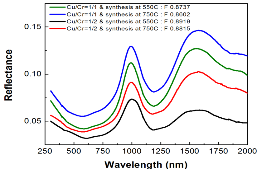
Fig.6. Reflectance change of SSC layers made of copper chromite nanoparticles with different atomic ratio (Cu/Cr) and crystallized at different temperatures. All coated samples were annealed with conditions of 750 °C/2h/air before reflectance measurement.
