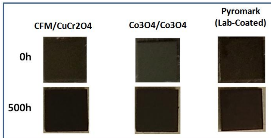
Fig. 29. Photos of samples taken before (0h) and after isothermal test (750°C/500h/air).
