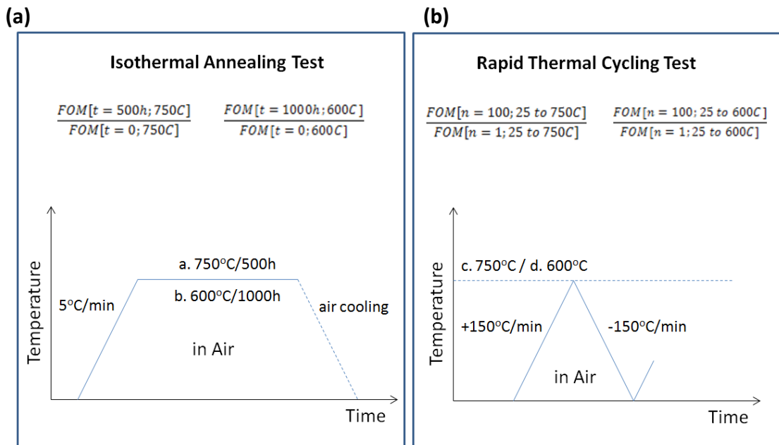
Fig. 19. Temperature profiles for (a) isothermal annealing test and (b) rapid thermal cycling test, and the equation to calculate FOM endurance.
