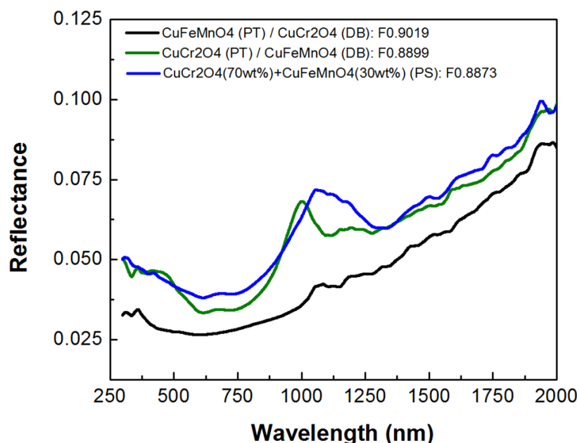
Fig. 15. Reflectance of double-layered sample and a single composite layered samples, fabricated with copper chromite and copper iron manganese oxide nanoparticles. All samples were annealed with the condition of 750 °C/2h/air before measuring. PT: porous top layer, DB: dense bottom layer, and PS: porous single layer.
