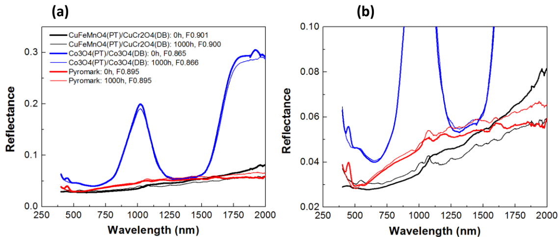
Fig. 21. Comparison of reflectance and FOM between as-prepared samples (0h) and samples annealed at 600°C/1000h/air. (PT: porous top layer, DB: dense bottom layer)
