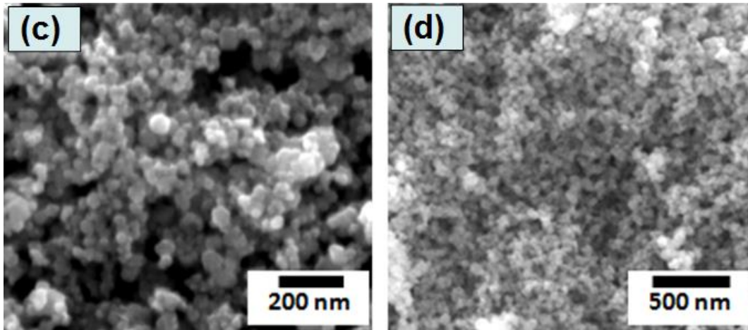
Fig. 12. SEM images showing the size change of bare \text{Fe}_3\text{O}_4 and \text{Y}_2\text{O}_3 -coated \text{Fe}_3\text{O}_4 NPs depending on the annealing temperature. (a)~(b) : \text{Fe}_3\text{O}_4 , (c)~(d) : \text{Y}_2\text{O}_3 -coated \text{Fe}_3\text{O}_4 , (a) and (c) : As-made, (b) and (d) : annealed at 750 °C for 2 hr.
