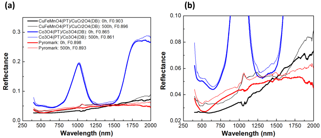
Fig. 26. Comparison of reflectance and FOM between as-prepared samples (0h) and samples annealed at 750°C/500h/air. (PT: porous top layer, DB: dense bottom layer)
