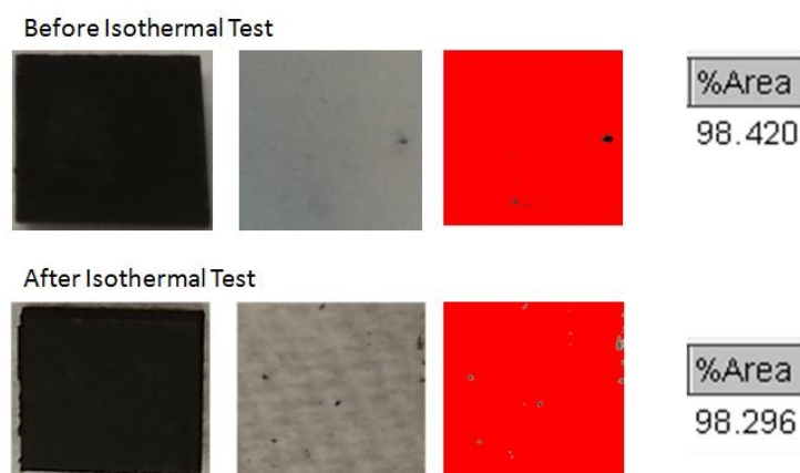
Fig. 33. Adhesion evaluations for repaired CuFeMnO 4 /CuCr 2 O 4 in the as-prepared state and after isothermal test (600°C/1000h/air). In each thermal test, The left is the sample image after removing tapes, the middle is the image of the detached tape, and the right is ImageJ-processed image which yields the retained area percentage.
