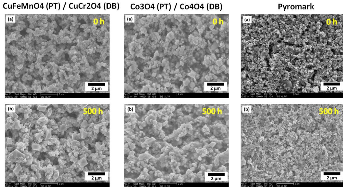
Fig. 28. SEM images showing surface morphologies of as-prepared samples (0h) and samples annealed at 750°C/500h/air, and observed in tilted angle of 30 degree.
