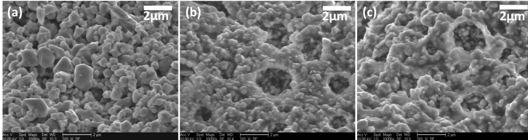
Fig. 14. SEM images of the porous Co 3 O 4 layers employing the polymer with the polymer beads of volume ratio 1:2 and 1:3 were shown in (a)-(c), respectively.
