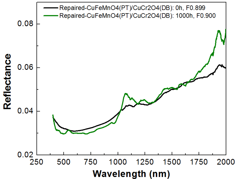
Fig. 31. Reflectance and FOM comparison between as-repaired CuFeMnO 4 /CuCr 2 O 4 (0h) and annealed one (600°C/1000h/air).
