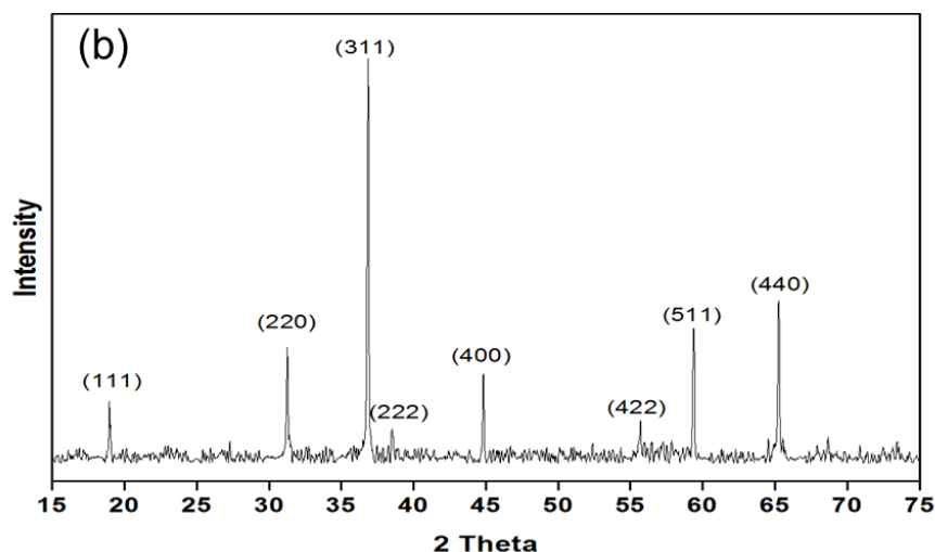
Fig. 3. X-ray diffraction pattern of Co oxide powders after stabilizing at 750°C for 2 hours, showing the \text{Co}_3\text{O}_4 phase.
