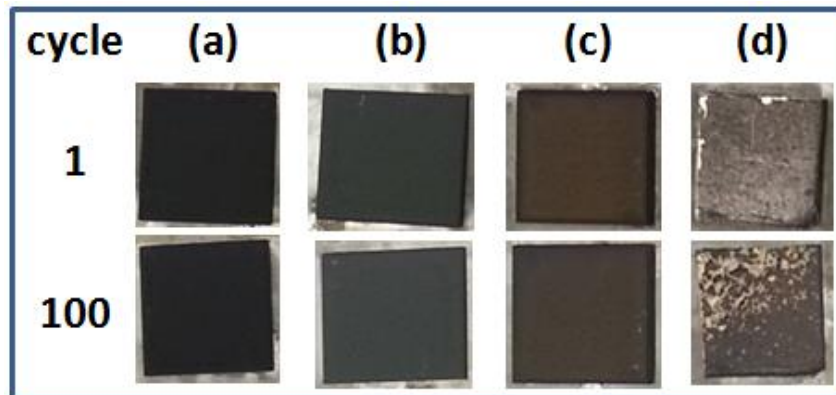
Fig. 24. Photo observation for 4 types of samples including CSP company-made Pyromark sample, taken after thermal cycling test (RT-750°C/100cycles/air).
