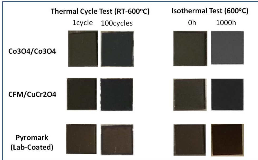
Fig.22. Photos of samples after thermal cycling (left two columns) and isothermal annealing (right two columns) at 600°C in air. Surface color of the images can be different from real colors because photos were not taken under the same environment.
