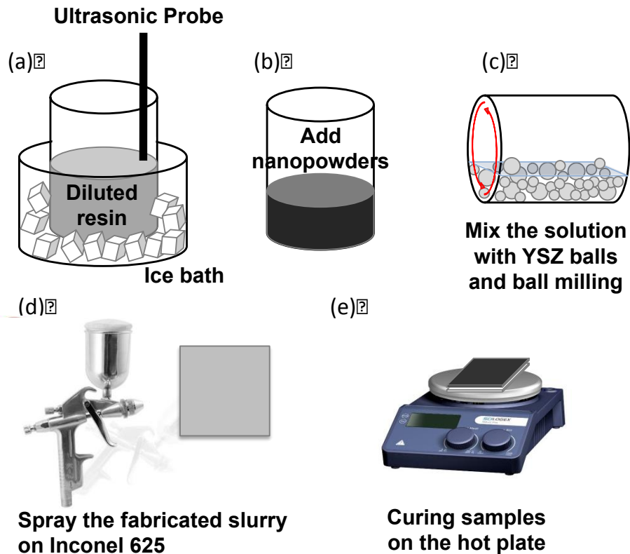
Fig 13. Fabrication procedure of light absorbing coating layers: (a) diluted resin with toluene(or xylene) and isobutanol (volume 3:1) thoroughly using an ultra-sonic probe, (b) added the synthesized nanopowders into the diluted resin, (c) ball milled the slurry with zirconia grinding balls for 24hours, (d) sprayed the slurry on Inconel metal substrates and (e) cured the samples at 250°C for 1hour
