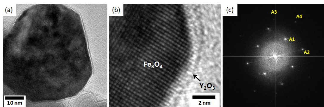
Fig. 10. (a) TEM images of \text{Fe}_3\text{O}_4\text{-Y}_2\text{O}_3 core-shell nanoparticles, (b) its magnified lattice image, and (c) its FFT patterns for the image (b).
