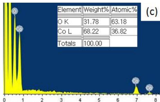
Fig.4. SEM images showing cobalt oxide ( \text{Co}_3\text{O}_4 ) nanorods ; (a) long nanorods with high aspect ratio and (b) short nanorods with low aspect ratio. And (c) EDX analysis result.
