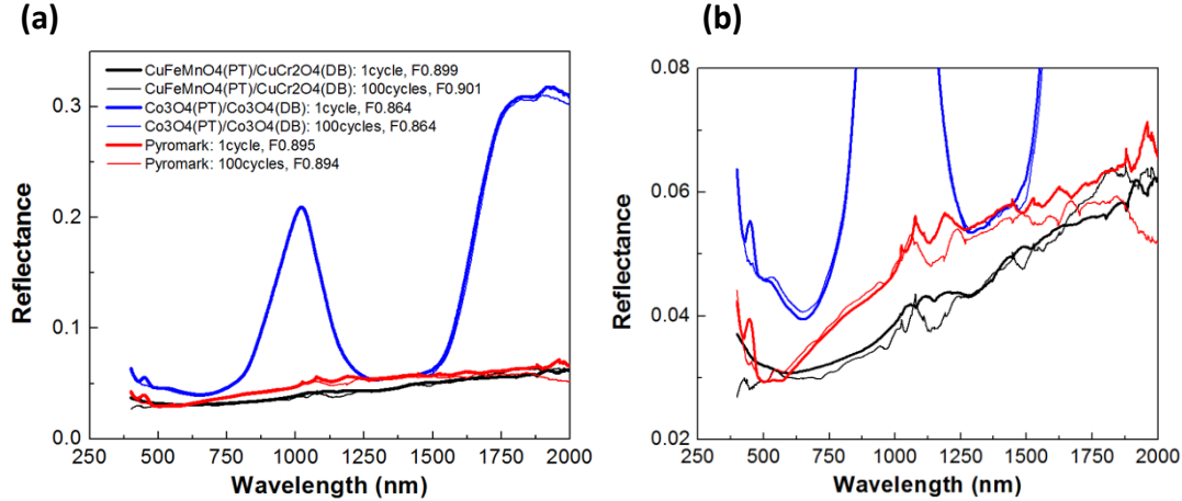
Fig. 20. Comparison of reflectance and FOM between 1-cycled samples and 100-cycled samples from RT to 600°C in air. (PT: porous top layer, DB: dense bottom layer)
