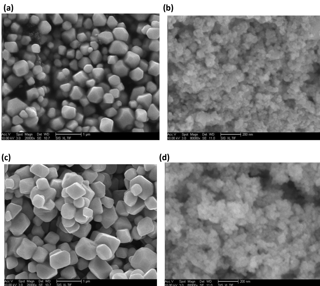
Fig. 5. Copper chromite particles synthesized with conditions of (a) Cu/Cr = 1/1 and crystallization at 750 °C/2h/air, (b) Cu/Cr = 1/1 and crystallization at 550 °C/5h/air, (c) Cu/Cr = 1/2 and crystallization at 750 °C/2h/air, and (d) Cu/Cr = 1/2 and crystallization at 550 °C/5h/air. Scale bar: 1 μm for (a) and (c), and 200 nm for (b) and (d).
