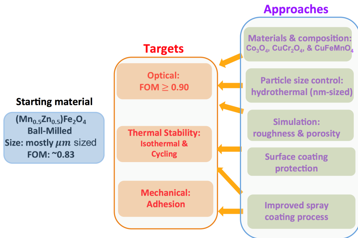
Fig. 1. Overview of research activities and technical approaches employed throughout this work. The developed SSC layers are expected to possess a combination of high performance merits, including high optical performance, measured by a figure of merit (FOM) greater than 0.90, excellent thermal durability and oxidation resistance, and excellent adhesion to the underlying substrates. To simultaneously meet these demanding and multi-facet requirements, multi-disciplinary approaches are pursued, including materials synthesis, optimization and processing, nanostructuring, optical and thermal measurements and modeling.
