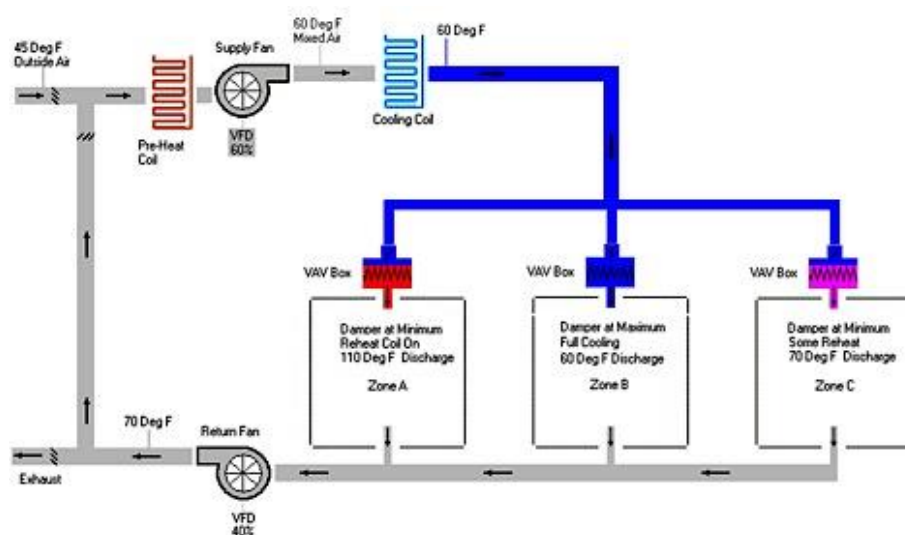
Figure A-1. Variable Air Volume with Reheat
