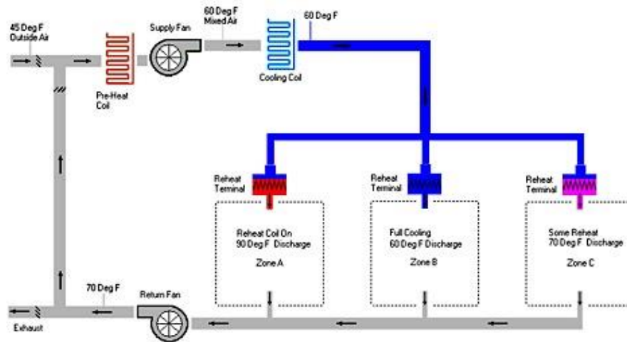
Figure A-2. Constant-Volume with Reheat
