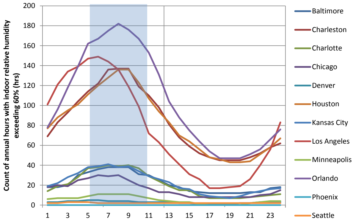
Figure 10 Hourly count of annual hours with indoor relative humidity exceeding 60% in a prototype 1.5 ACH 50 DOE Challenge Home with simple exhaust ventilation.
