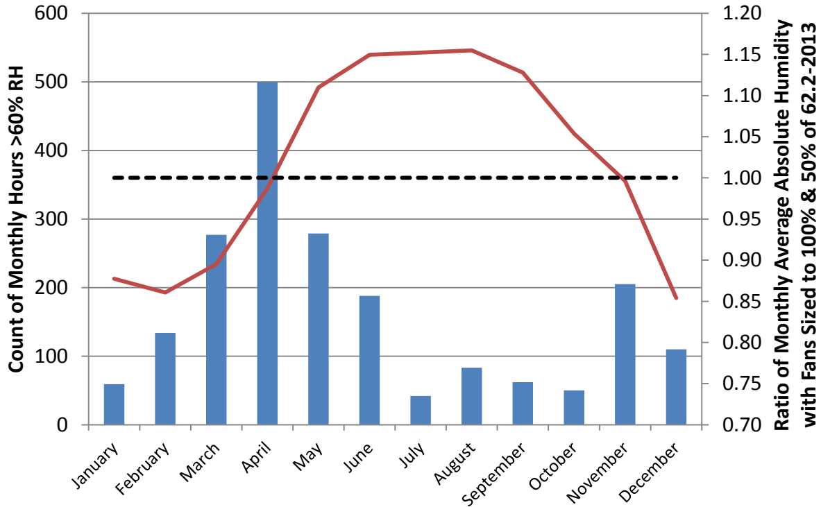
Figure 8 Monthly plot of hours exceeding 60% RH (blue bars) and ratios of indoor absolute humidity with ventilation fans sized to 100% and 50% of 62.2-2013 (solid red line). Houston, TX 1.5 ACH 50 home.
