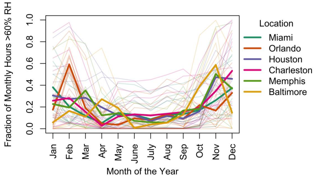
Figure 21 Average fraction of monthly hours above 60% RH, grouped by climate zone. Includes only homes with no dehumidification, where more than 5% of annual hours were >60% RH. The lighter, opaque lines represent individual simulations (colored by climate zone), while the bold lines represent the climate zone averages.
