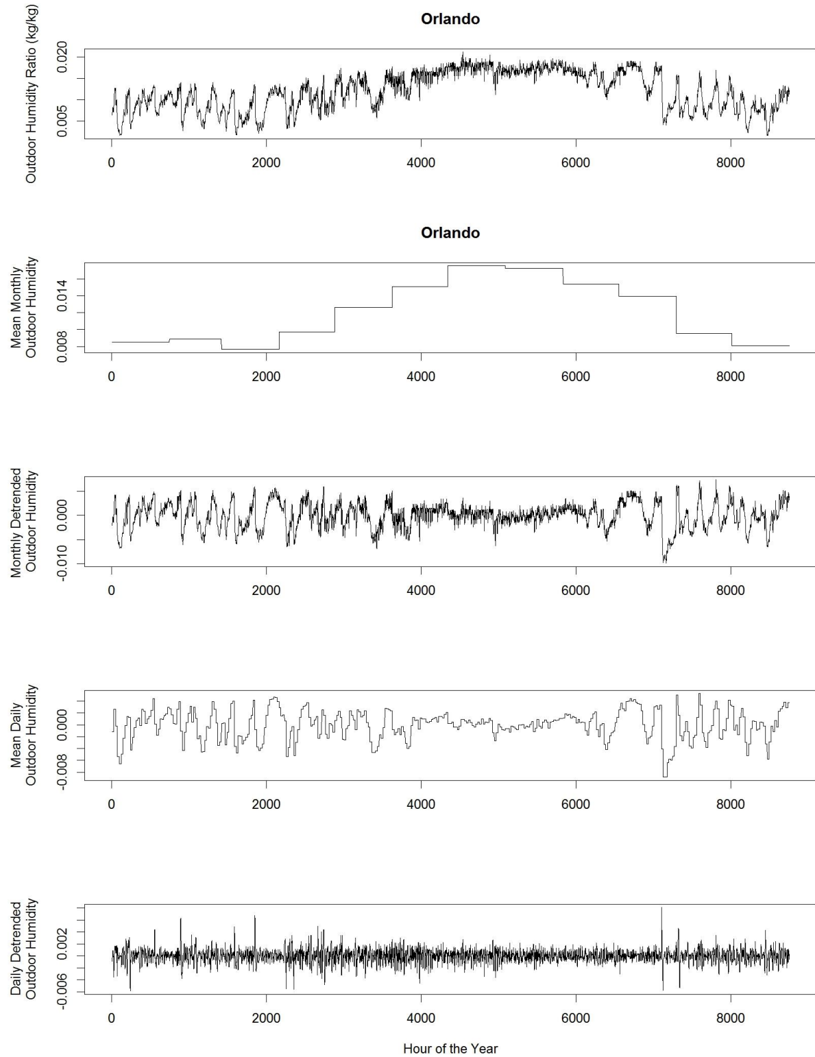
Figure 40 Time series decomposition plot for Orlando.
