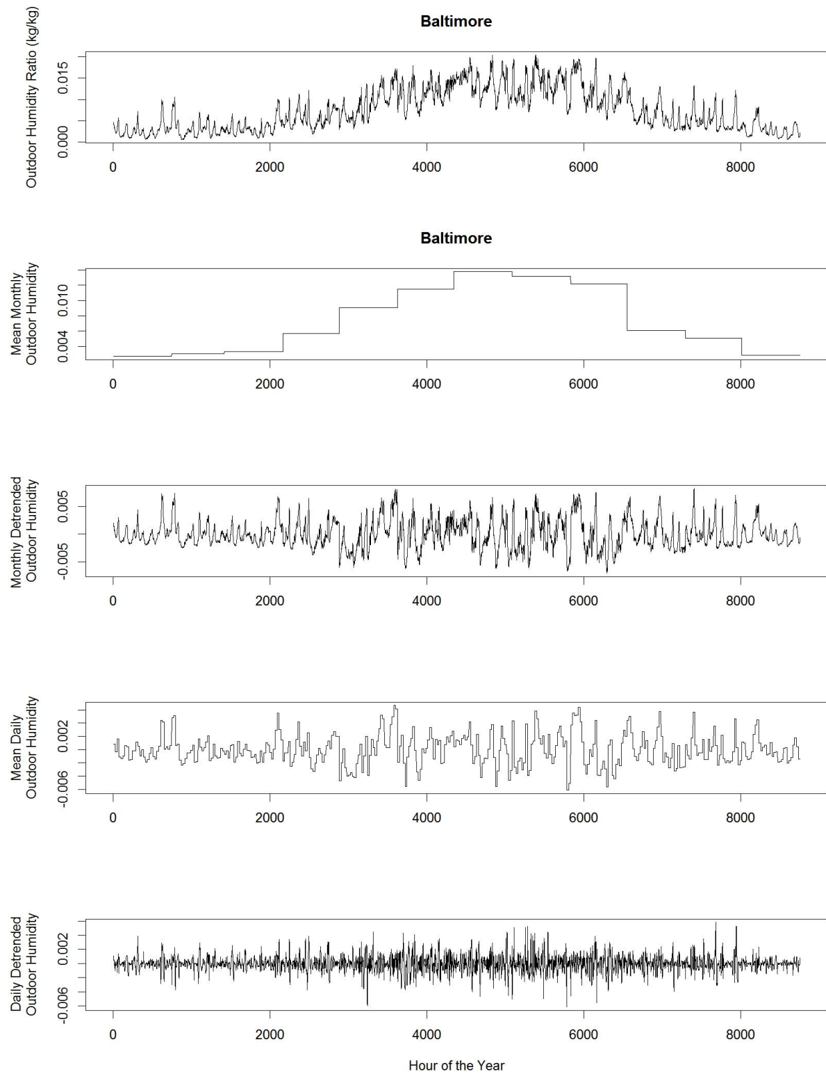
Figure 44 Time series decomposition plot for Baltimore.
