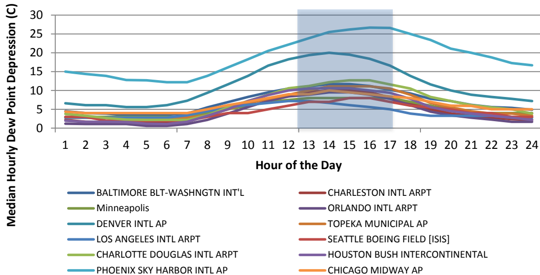
Figure 7 Hourly profiles of the median dew point depression in varying climate zones. The peak is quite consistent across climates, with the hours of 12pm to 6pm having the largest values, indicative of greater dehumidification potential in mechanically cooled spaces.
