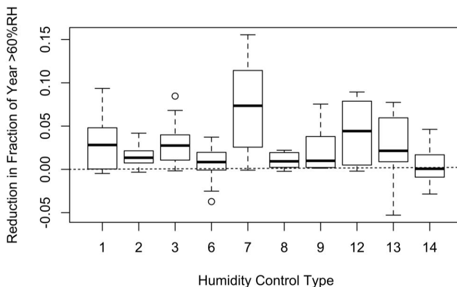
Figure 31 Distributions of the reduction in the fraction of the year >60% RH by each smart control strategy. Includes only cases without dehumidification. Reductions are absolute, not relative, in that 0.10 means that 10% of hours were shifted from above to below the 60% RH threshold.
