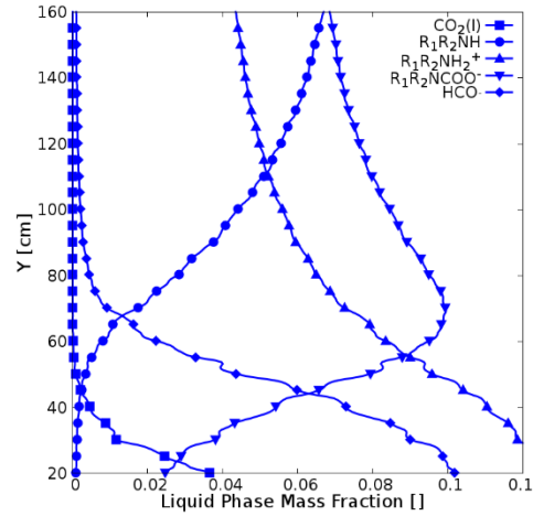
(c) Liquid-phase mass fractions
