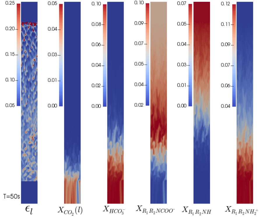
(a) Instantaneous contours of liquid fraction ( \epsilon_l ) and liquid species mass fraction ( X_i )
