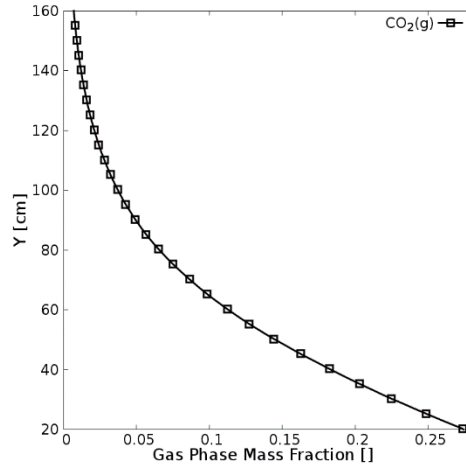
(b) Gas-phase CO_2 mass fraction
