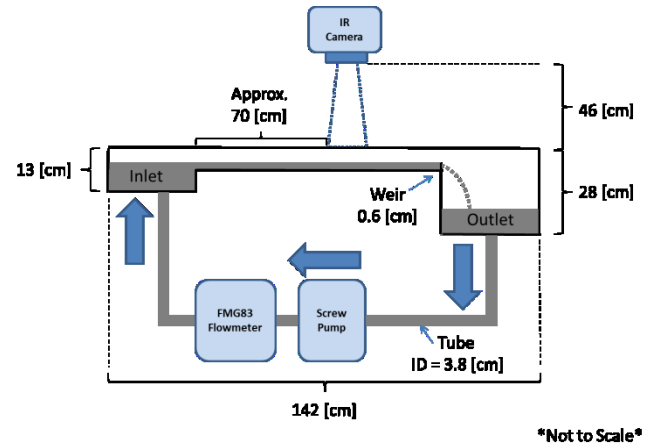
FIG. 1. (Color online). A simple depiction of the LMX flow path and instrumentation layout. The width of the channel ( w ) was a constant 10.9 [cm].
