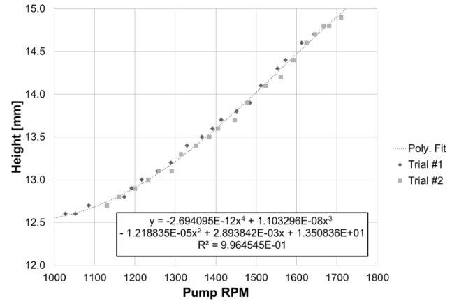
FIG. 4. The height of the flowing galinstan surface as a function of pump RPM. Data was collected using the electrical contact method. Above 1000 RPM the galinstan began to flow over the weir and circulate through the system. The surface of the galinstan rises above the weir before beginning to flow due to surface tension effects ( \gamma = 0.533 [N/m]) 6,7 .
