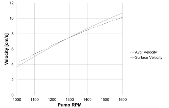
FIG. 7. A comparison of the average and surface velocities. The values shown above were calculated using the linear and polynomial fits given in FIG. 2, FIG. 4, and FIG. 6.
