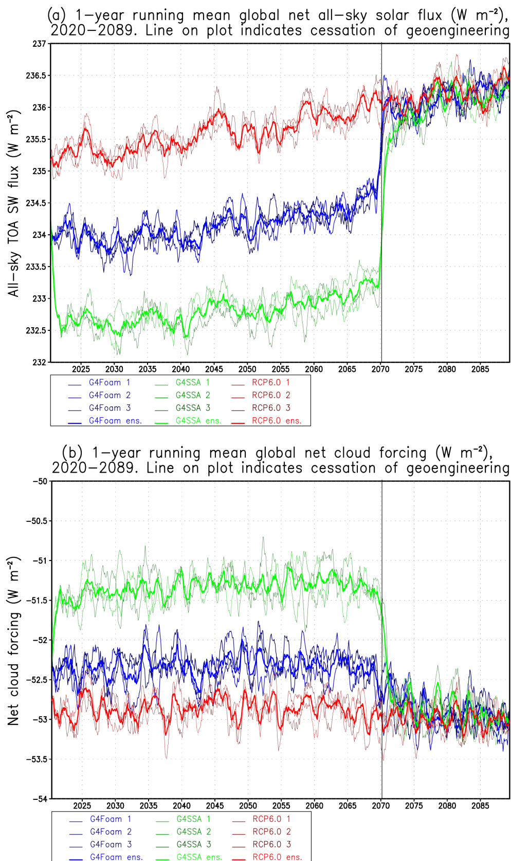
Figure 2. (a) Net all-sky SW flux at top of atmosphere and (b) time series of global mean net cloud forcing. Each ensemble member and the ensemble mean are shown for each forcing.
