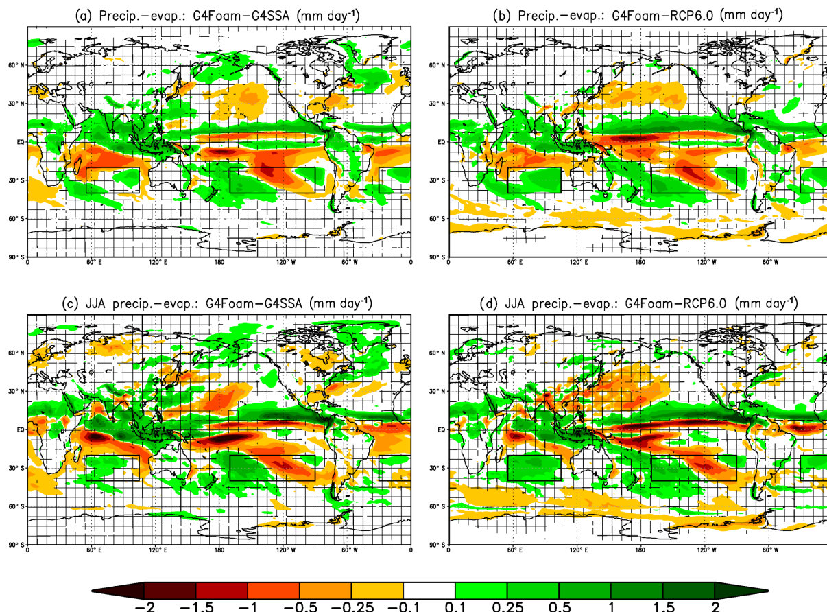
Figure 8. 2030–2069 precipitation minus evaporation difference (mm day -1 ) between G4Foam and (a) G4SSA, (b) RCP6.0, (c) G4SSA during JJA, and (d) RCP6.0 during JJA. Hatched regions are areas with p > 0.05 (where changes are not statistically significant based on a paired t test). Black boxes enclose foamed regions.
