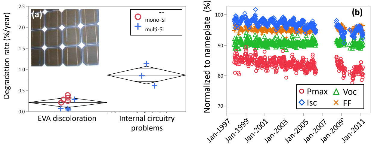
Fig. 6. Encapsulant discoloration is the most noticeable degradation mode. In a side-by-side comparison, encapsulant discoloration had significantly less effect on power than modules that showed internal circuitry problems associated with series resistance increase (a). The decline is I_{sc} dominated and appears fairly consistent during more than 10 years of field exposure (b).
