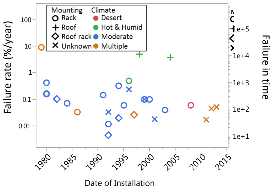
Fig. 1. Failure rate in %/year (left axis) and FIT (right axis) of PV modules and systems during the last 35 years color coded by climate and symbol coded by mounting configuration. Failure in
