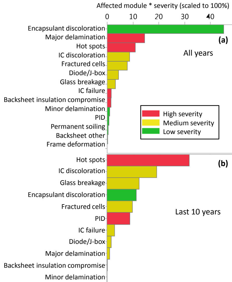
Fig. 3. Pareto chart of the most significant degradation modes for all years (a) and systems installed in the last 10 years (b). The bars are color coded by severity.
