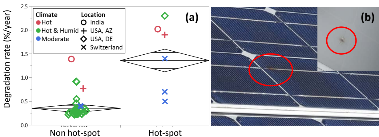
Fig. 4. In side-by-side comparison, modules affected by hot spots show consistently higher degradation than modules without hot spots (a). The studies from Arizona and India used the nameplate rating, which may have influenced the absolute value. Hot spots can easily be
