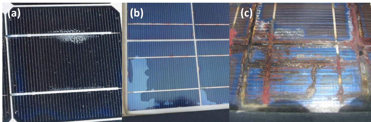
Fig. 5. Encapsulant delamination can occur at the encapsulant-silicon interface and typically starts to appear along the cell busbar (a), or at the glass-encapsulant interface (b). Depending on the field exposure duration and severity, delamination can be accompanied by internal circuitry discoloration (c).
