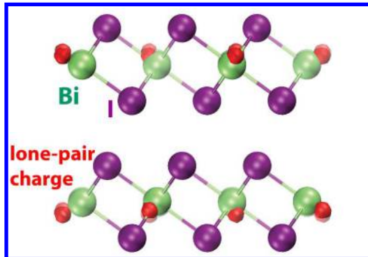
Figure 11. Layered crystal structure of BiI 3 (space group 148) depicting the localized Bi cation 6s lone pair by the red spheres (0.06 e Å 3 with respect to the superposed atomic densities).
