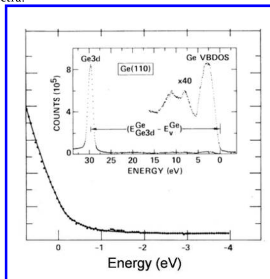
Figure 5. Least-squares fit of instrumentally-broadened valence band density of states to the leading edge of Ge measured by XPS. Core levels and valence band density of states (VB DOS) shown inset. Reproduced with permission from Ref. 171.
