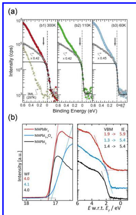
Figure 6. (a) UPS measurements of pentacene on chloroaluminium phthalocyanin performed at 300 K (b1), 110 K (b2) and 60 K (b3). Reproduced from with permission from Ref. 172. (b) UPS measurement of hybrid organic-inorganic lead-halide perovskite layers with secondary electron cut-off (left) and valence band onset (right, semilogarithmic representation). Reproduced from with permission from Ref. 163.
