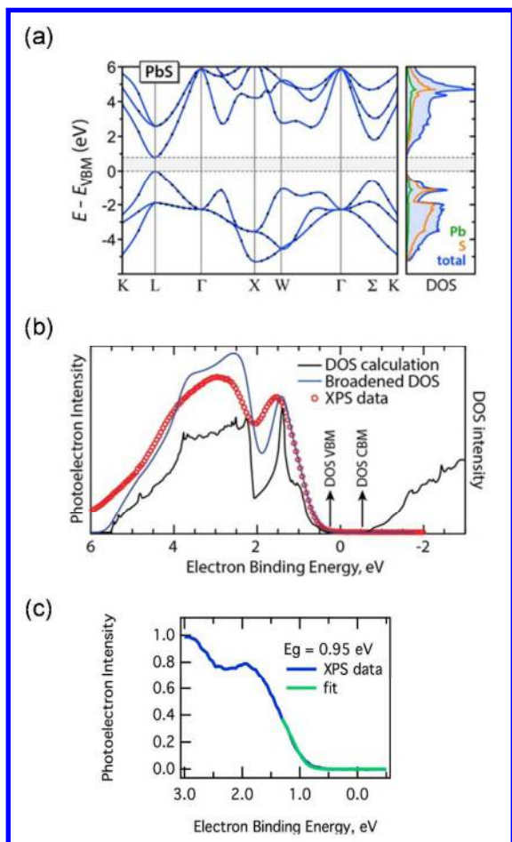
Figure 7. (a) Electronic band structure and density of states of bulk PbS calculated with the GW approximation. (b) Comparing the GW-calculated density of states, fitted instrument-broadened valence band density of states and XPS spectrum of bulk PbS. (c) Comparison of the XPS measurement of 0.95 eV bandgap PbS quantum dots and the fitted parabolic density of states model. Reproduced with permission from Ref. 164. Copyright 2016 American Chemical Society.
