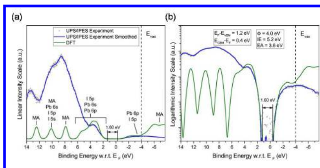
Figure 8. UPS and IPES spectra of MAPbI 3 in (a) linear and (b) semilogarithmic plots. These spectra are compared to the density of states calculated by DFT. Reproduced with permission from Ref. 177.
