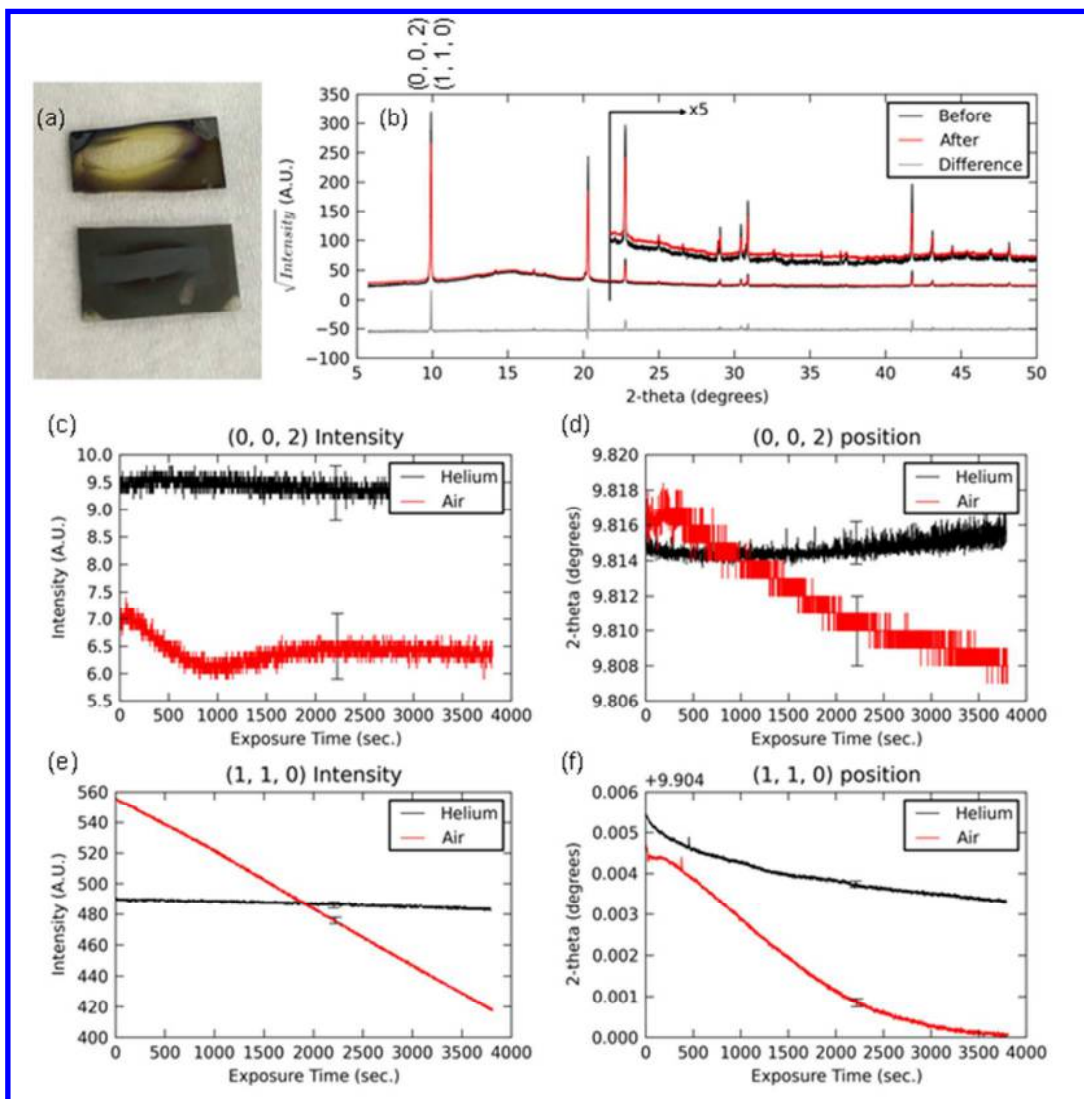
Figure 1. Beam damage study of MAPbI 3 films at room temperature taken by the authors. (a) Image of MAPbI 3 films after approximately 24 h of X-ray exposure in air (top) and in helium (bottom). (b) Full powder XRD patterns both before and after 1 h of X-ray exposure in air. The difference between the two patterns is plotted below, showing significant differences due to beam damage. The fitted intensities and positions of the (0, 0, 2) and (1, 1, 0) peaks are shown as a function of X-ray exposure time in panels (c-f), with error bars plotted at representative points. The error bars for the (1, 1, 0) peak intensity are multiplied by a factor of 10 for clarity. We note that the (0, 0, 2) and (1, 1, 0) peak positions are at different 2\theta values to lab-standard diffraction patterns because these measurements were taken using a 10.995 keV X-ray beam, rather than a 8.049 keV Cu K \alpha X-ray beam. The raw data is available as Supporting Information.
