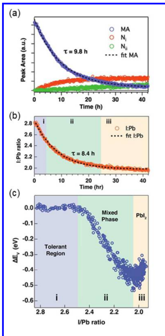
Figure 10. Degradation of MAPbI 3 under extended X-ray exposure. (a) Change in areas of peaks fit to N 1s peak in XPS measurements over time of X-ray exposure. The N species are attributed to methylammonium (MA) and nitrogen-rich reaction products (N i and N ii ). (b) Ratio of I to Pb and (c) shift in valence band relative to Fermi level during X-ray exposure. Reproduced with permission from Ref. 187. Copyright 2016 American Chemical Society.
