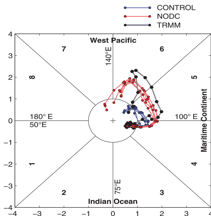
Figure 3. Large-scale precipitation tracking (LPT) phase diagram for 24 November to 22 December 2011 for TRMM (black), the CONTROL simulations (blue), and the NODC simulations (red). The circle markers are for daily mean LPT longitude and amplitude. Diamonds indicate the LPT initiation points. LPT phase is determined by the longitude of the centroid of convection with breakpoints indicated on the diagram. Amplitude is the effective radius divided by 600 km. Only the longest lasting LPTs within the model simulation domain for TRMM and for each simulation are drawn.
