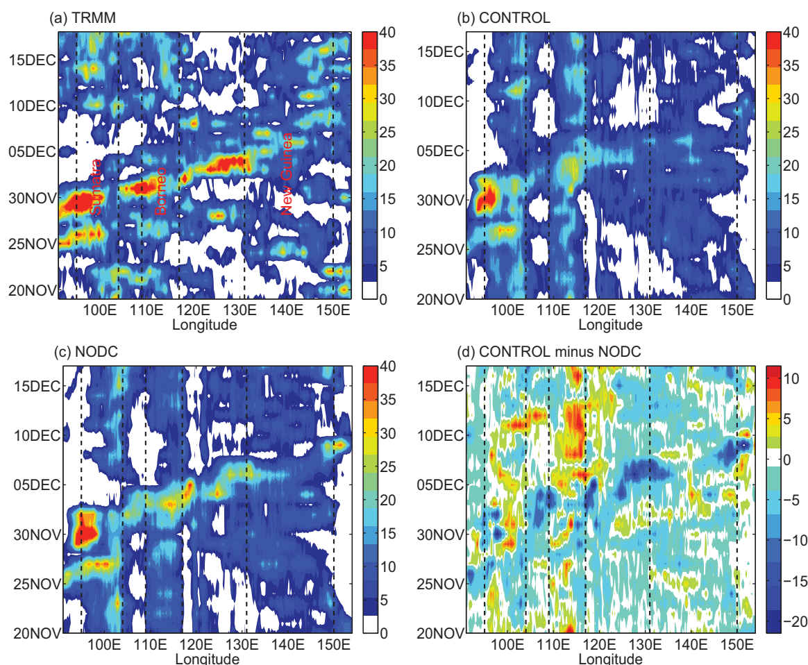
Figure 2. Hovmöller diagrams of precipitation ( \text{mm d}^{-1} ) averaged between 5^{\circ}\text{S} and 5^{\circ}\text{N} from (a) TRMM, (b) CONTROL, (c) NODC, and (d) the difference between CONTROL and NODC. The vertical dashed lines mark the boundaries of the islands of Sumatra, Borneo, and New Guinea.
