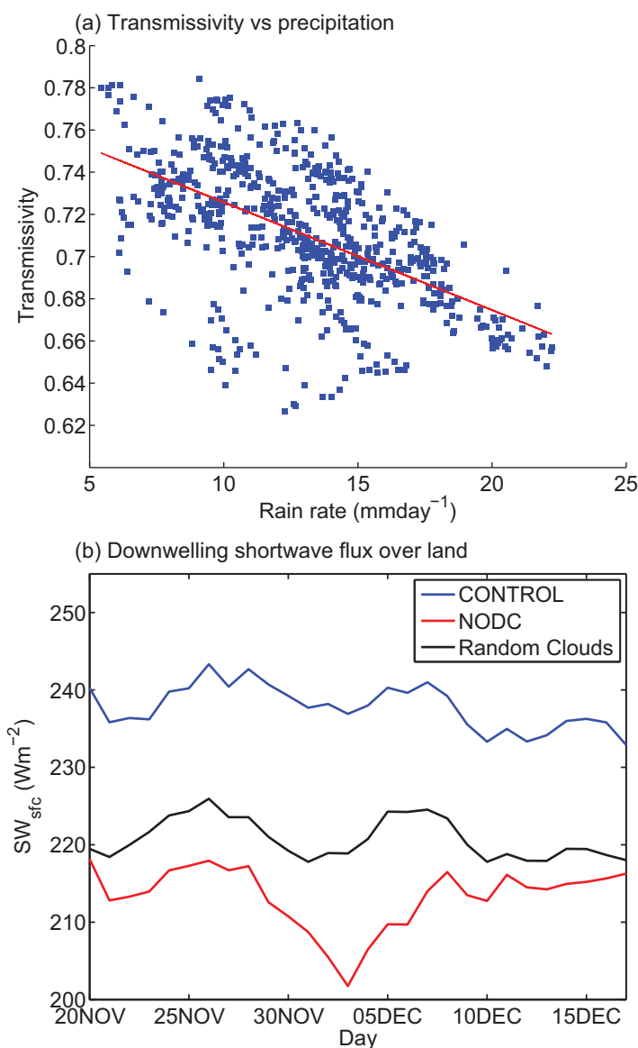
Figure 6. (a) Relationship between rain rate and transmissivity from the CONTROL simulation. The correlation is -0.58 , (b) as in Figure 4a, but including diurnal mean surface downwelling shortwave radiation using the hypothetical random diurnal distribution of cloudiness.
