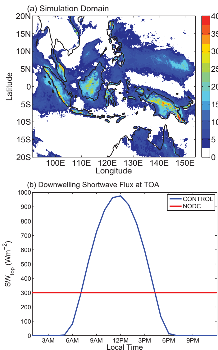
Figure 1. (a) Simulation domain and monthly mean precipitation from the model ( \text{mm d}^{-1} ). (b) Top of the atmosphere (TOA) downwelling shortwave radiation ( \text{W m}^{-2} ) for the CONTROL and NODC simulations averaged over the simulation period. The daily mean values are equal for the two simulations.
