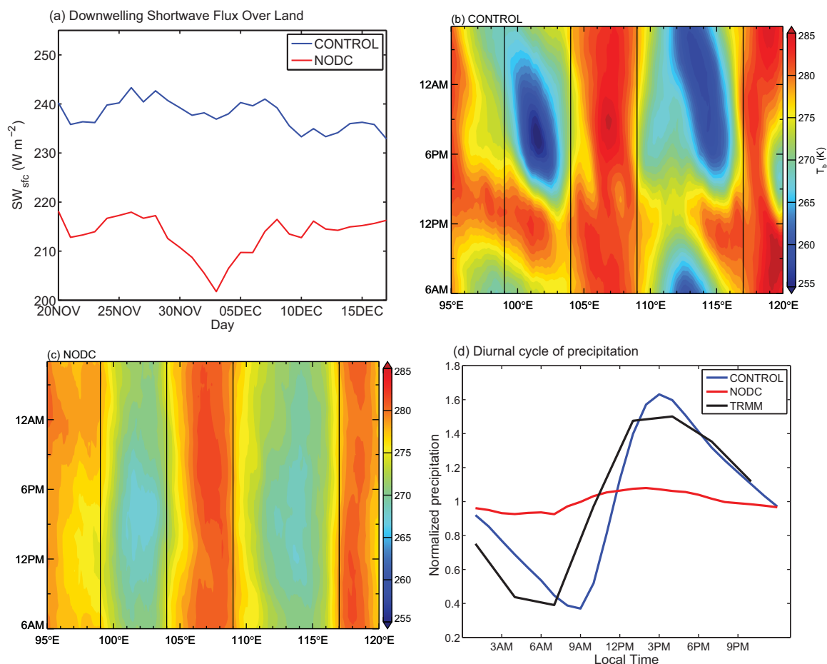
Figure 5. (a) Diurnal mean surface downwelling shortwave radiation (SW sfc ) averaged over the islands of Sumatra and Borneo and smoothed by a 5-point moving average, Hovmöller diagram of diurnal cycle of outgoing infrared brightness temperature (T b ) from (b) CONTROL and (c) NODC averaged between 5°S and 5°N. (d) Diurnal cycle of precipitation averaged over Sumatra and Borneo, normalized by the daily mean.
