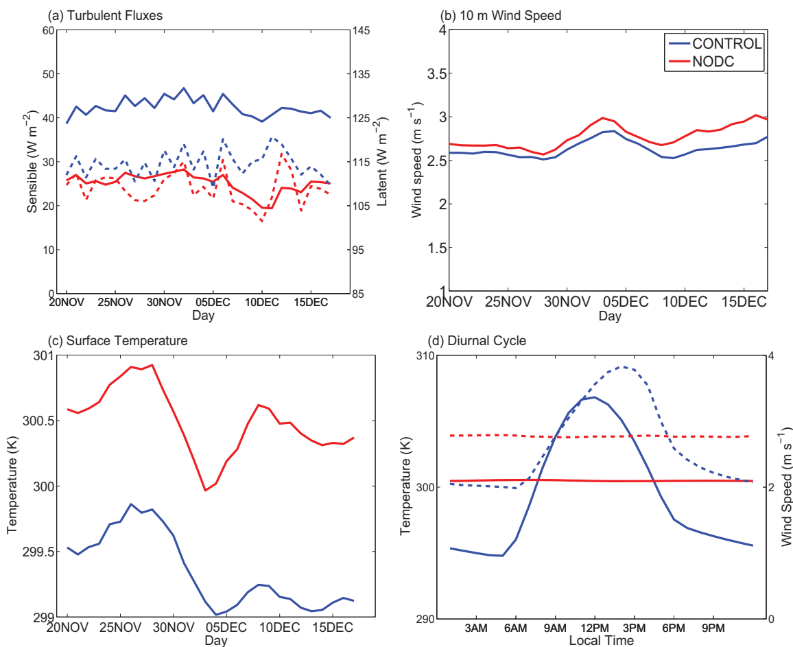
Figure 8. Time series of diurnal mean surface sensible (solid) and latent (dashed) heat flux, (b) 10 m wind speed, (c) land surface temperature, and (d) monthly mean diurnal cycles of surface skin temperature (solid) and 10 m wind speed (dashed). CONTROL ensemble mean is in blue and NODC ensemble mean is in red. All are averaged over the Islands of Sumatra and Borneo and the time series in Figures 8a–8c are smoothed by a 5-point moving average.
