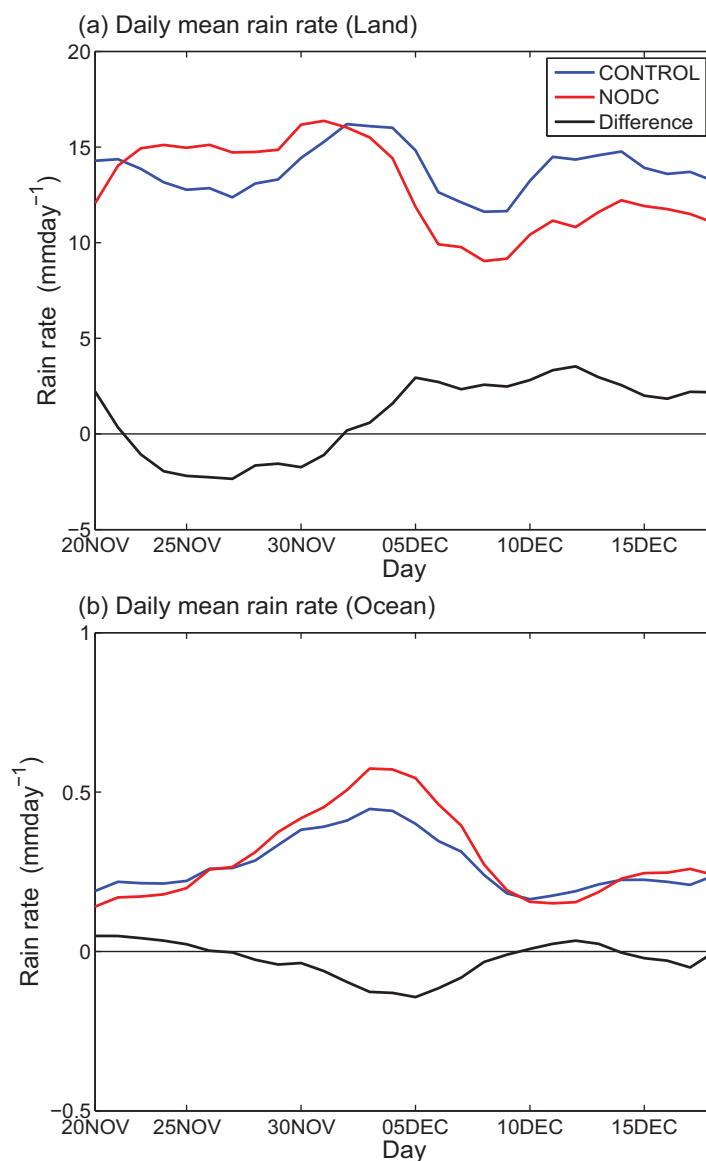
Figure 4. Daily mean rain rate averaged over (a) the islands of Sumatra and Borneo and (b) the adjacent waters. The averaging areas are 95°E–120°E and 5°S–5°N and the time series are smoothed by a 5-point moving average.
