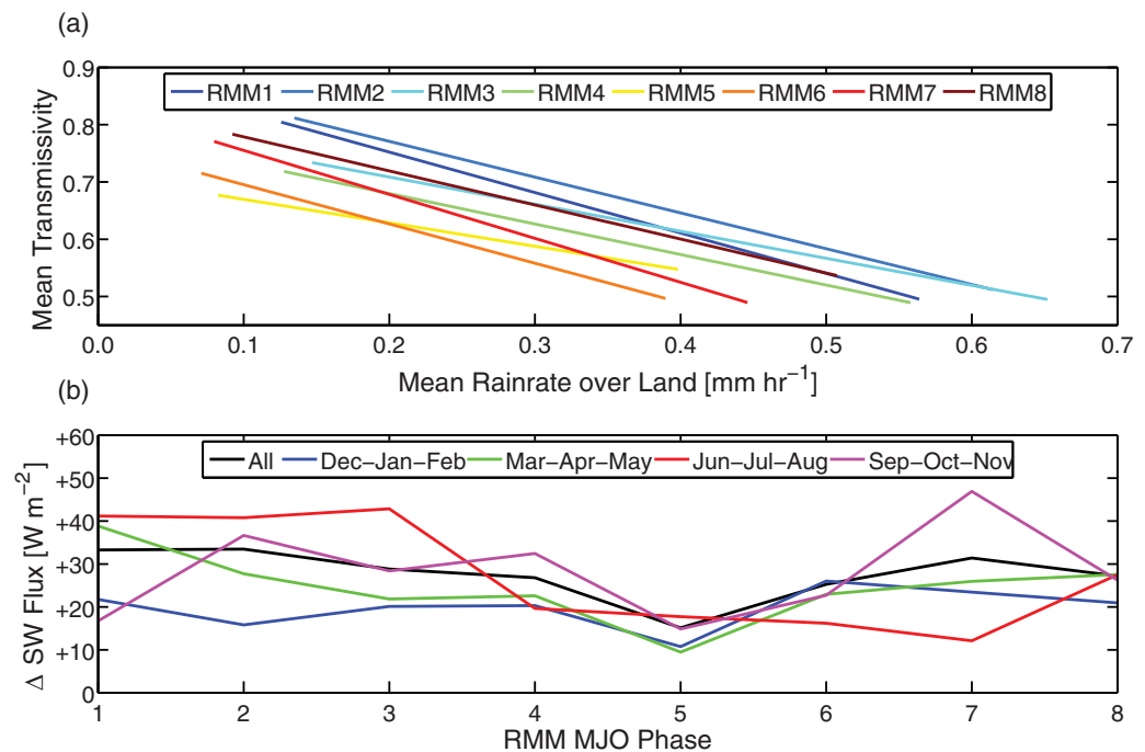
Figure 9. (a) Linear-regression relationship between the mean rain rate over land in the MC and the mean SW transmissivity (the ratio of cloudy to clear-sky SW flux at the surface) at the Manus DOE ARM site. (b) Change in the total SW flux reaching the surface that would occur if the observed clouds were randomly distributed across the diurnal cycle. The regressions and change in SW flux are both derived for each RMM MJO phase. Black is for all year and the colors are for different seasons.
