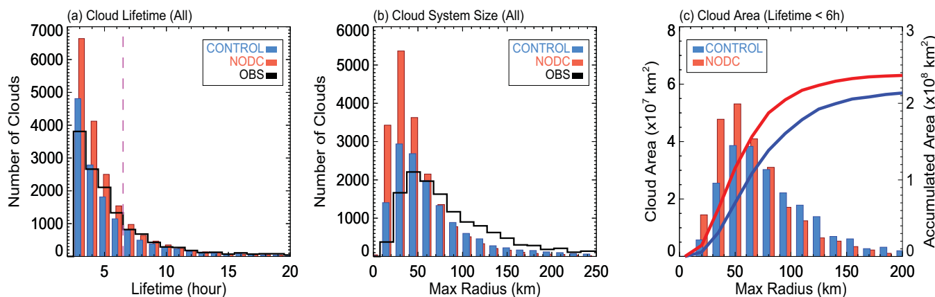
Figure 7. Statistics of convective cloud systems initiated over land: (a) lifetime of clouds, (b) maximum equivalent radii of clouds during their lifetime, and (c) total integrated maximum cloud area for each radius bin (number of cloud systems in each radius bin \times radius value). Cloud systems include all clouds with infrared brightness temperature lower than 260 K. The vertical dashed line in Figure 7a marks lifetime of 6 h.
