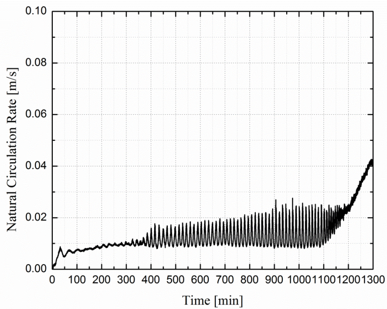
Figure 5-39 Natural Circulation Rate for Very Slow Startup Transient
