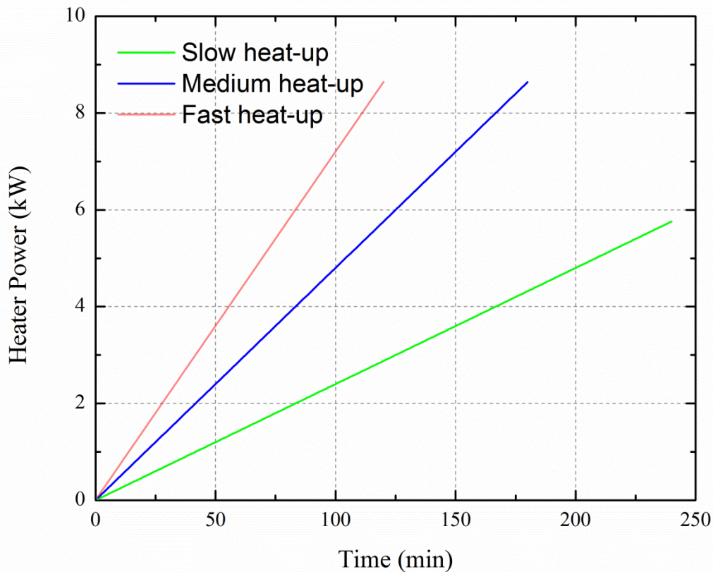
Figure 6-1 Power Curves for Pressurized Startup Transients
