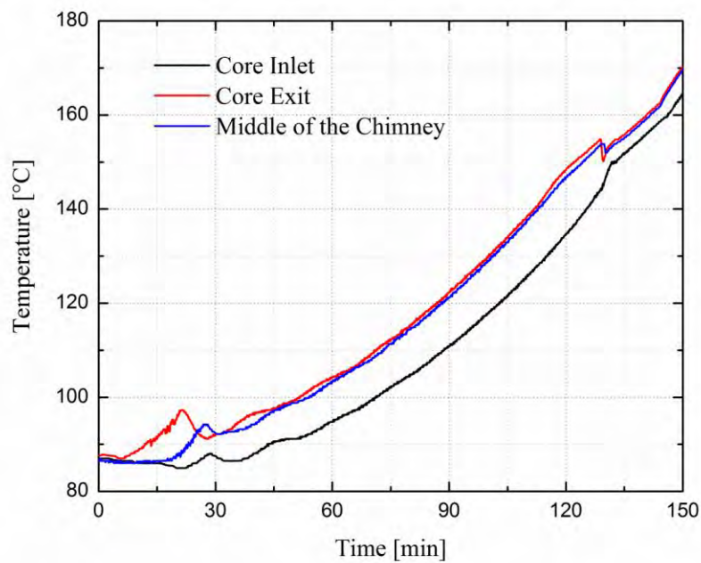
Figure 6-10 Temperatures for Pressurized Medium Startup Transient
