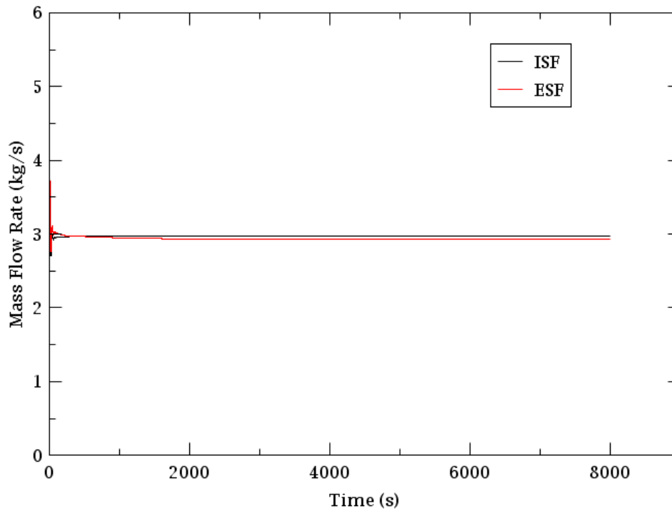
Figure 11-10 Steady State Mass Flow Rate Comparison of the ISF and the ESF by RELAP5
