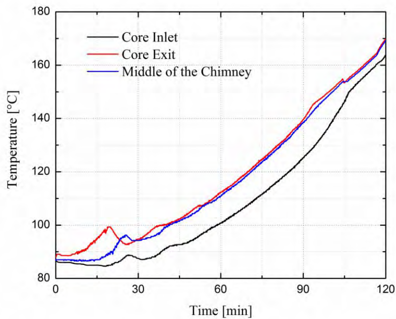
Figure 6-16 Temperatures for Pressurized Fast Startup Transient
