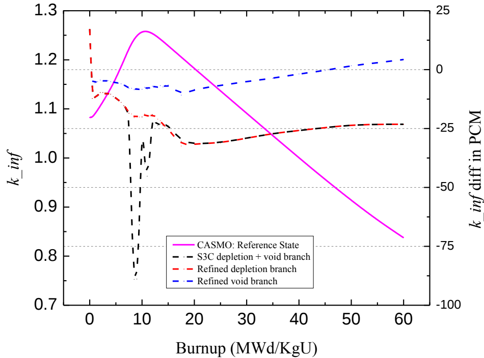
Figure 2-3 k_{inf} vs. burnup results for case problem with the high moderator density
