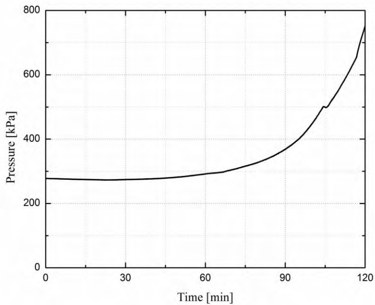
Figure 6-15 Steam Dome Pressure for Pressurized Fast Startup Transient
