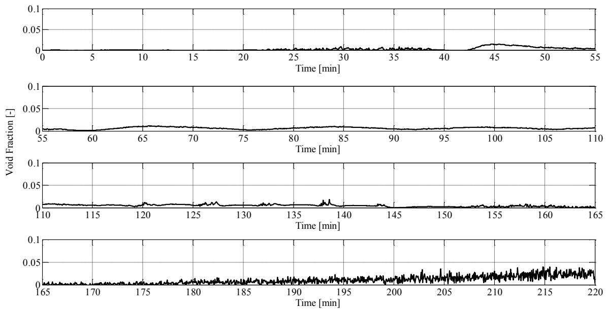
Figure 5-26 Void Fraction at the Chimney Inlet (IMP04) for the Slow Startup with Void Reactivity Feedback
