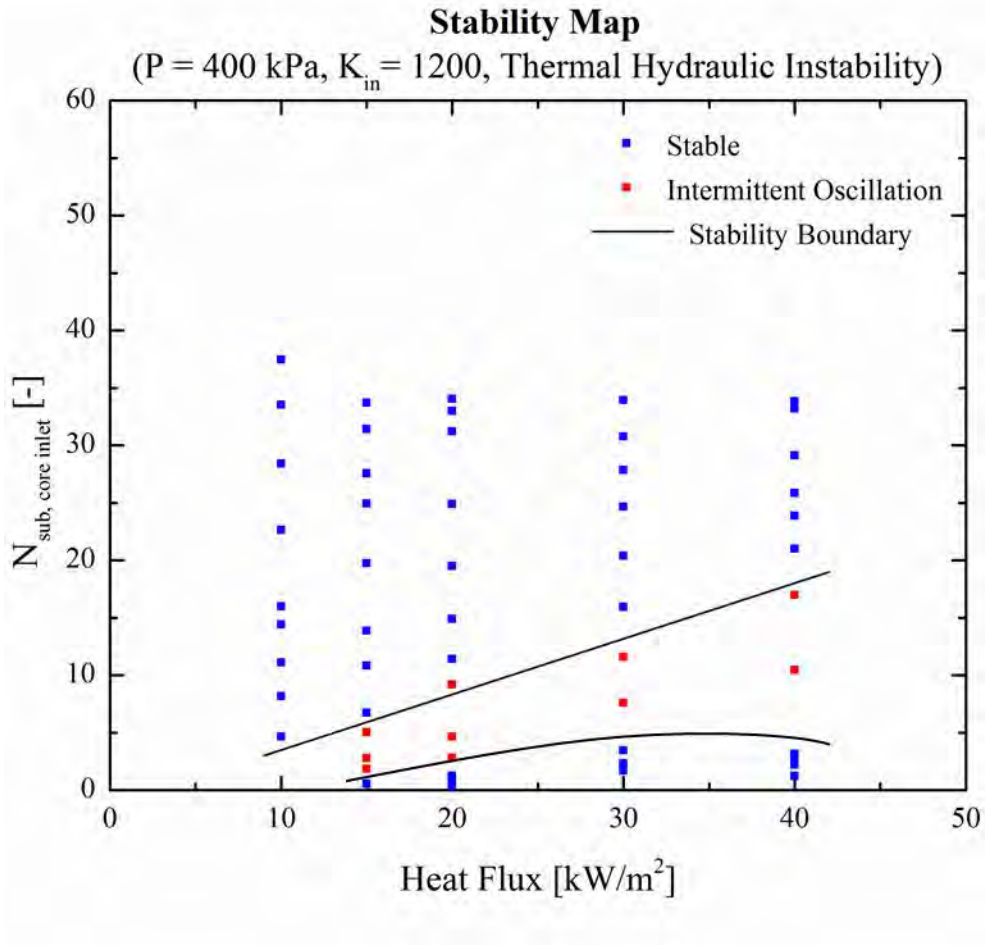
Figure 7-5 Stability Map at 400 kPa
