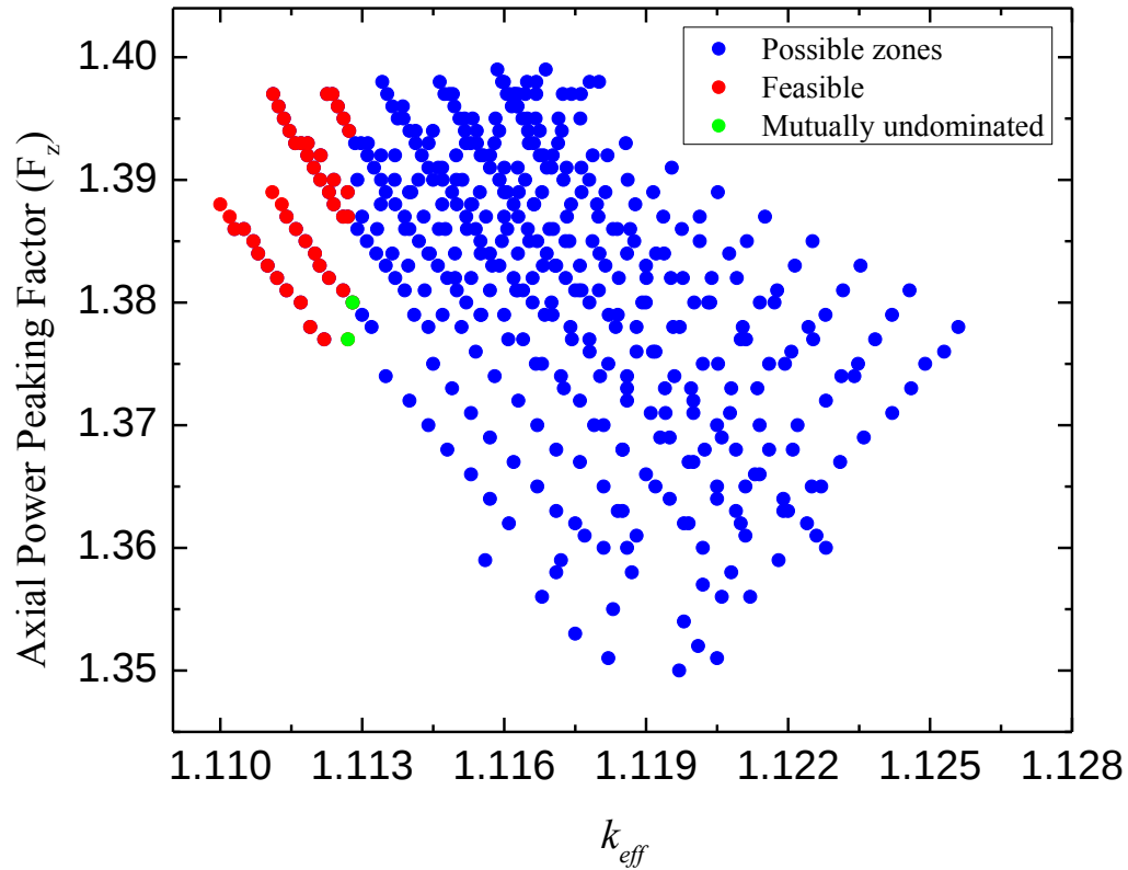
Figure 2-9 Axial power peaking factor versus k_{eff}
