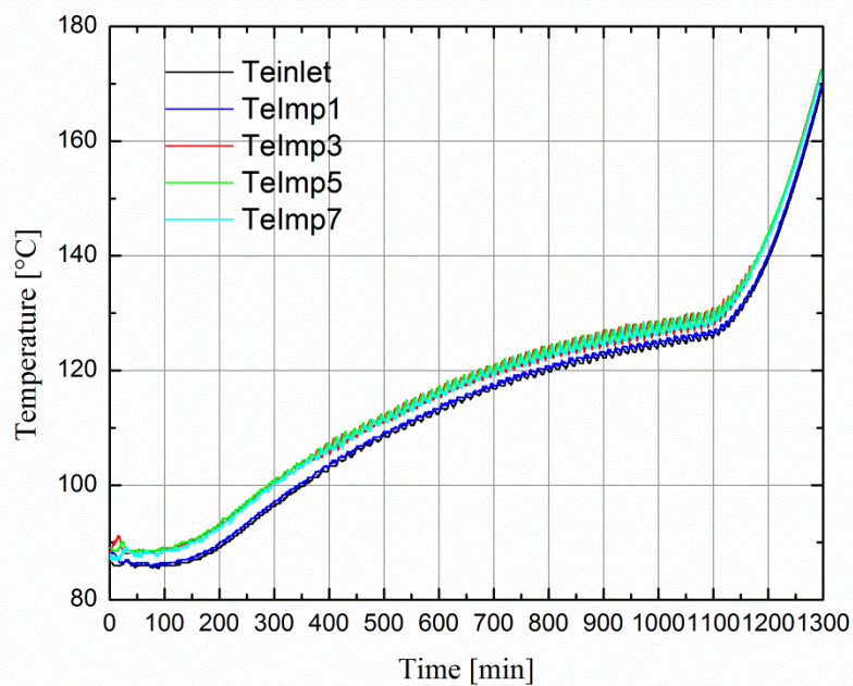
Figure 5-37 Temperatures for Very Slow Startup Transient
