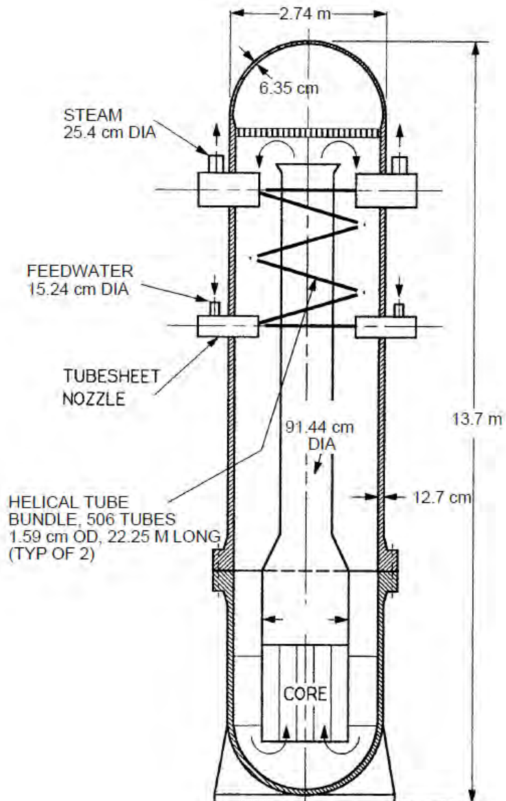
Figure 9-3 Schematic Design of NuScale (MASLWR) RPV [46]
