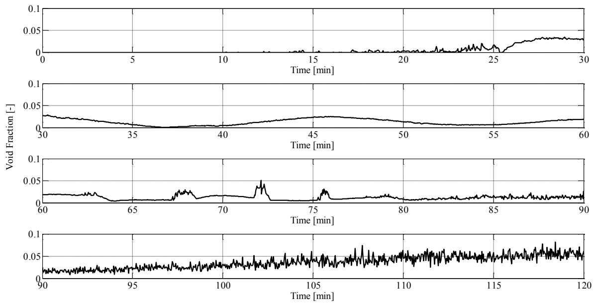
Figure 5-16 Void Fraction at the Chimney Inlet (IMP04) for the Fast Startup Transient
