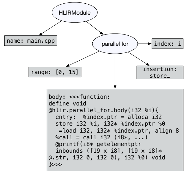
Figure 1: A portion of an HLIR module containing a simple parallel for.
