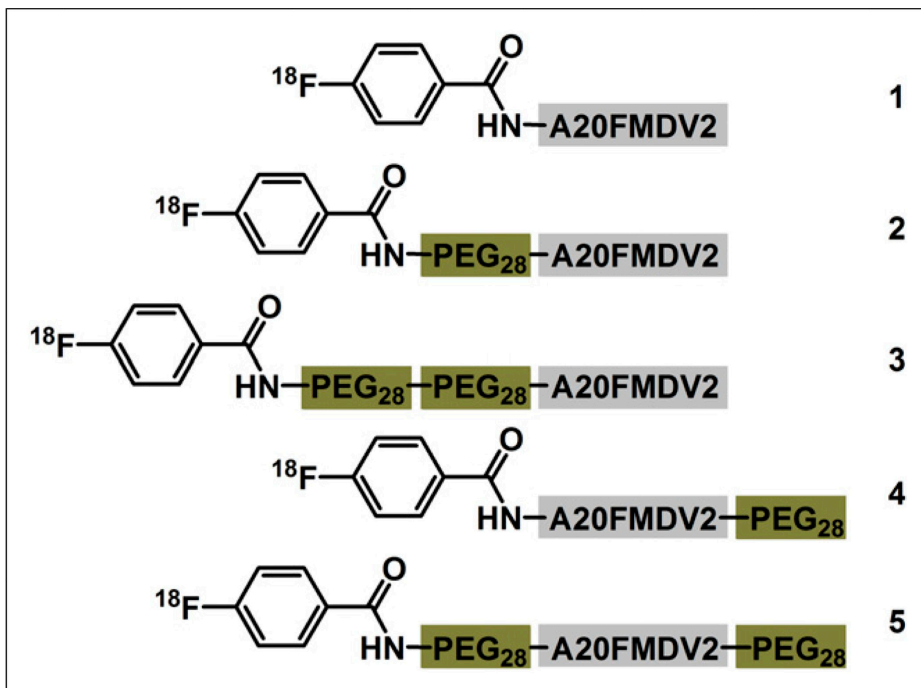
Figure 1. Structures of radiotracers evaluated.
