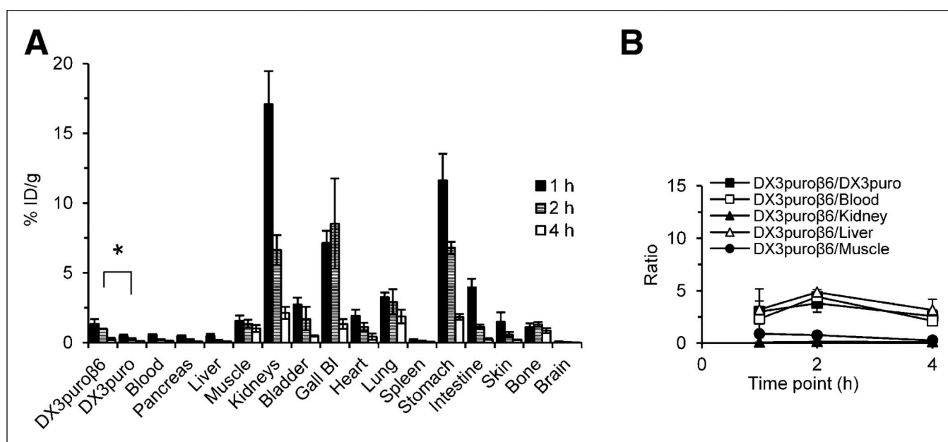
Figure 3. Biodistribution data of ^{18}\text{F} -FBA-A20FMDV2-PEG 28 ( 4 ) in mice bearing paired \alpha_v\beta_6 -expressing DX3puro \beta_6 and non- \alpha_v\beta_6 -expressing DX3puro xenograft tumors. (A) Organ uptake (%ID/g; bars = SD; n = 3 /time point). * P = 0.02 for corresponding time points. (B) Uptake ratios of 4 for tumors and selected organs (bars = SD). Bl = bladder.
