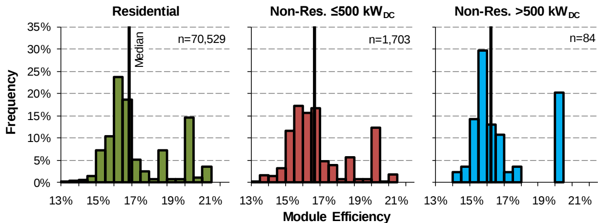
Figure 27. Module Efficiency Distributions for Systems Installed in 2015
