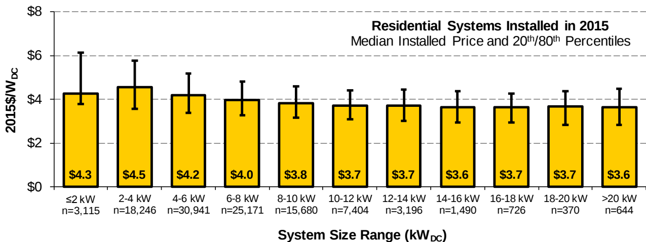
Figure 16. Installed Price of 2015 Residential Systems by Size
