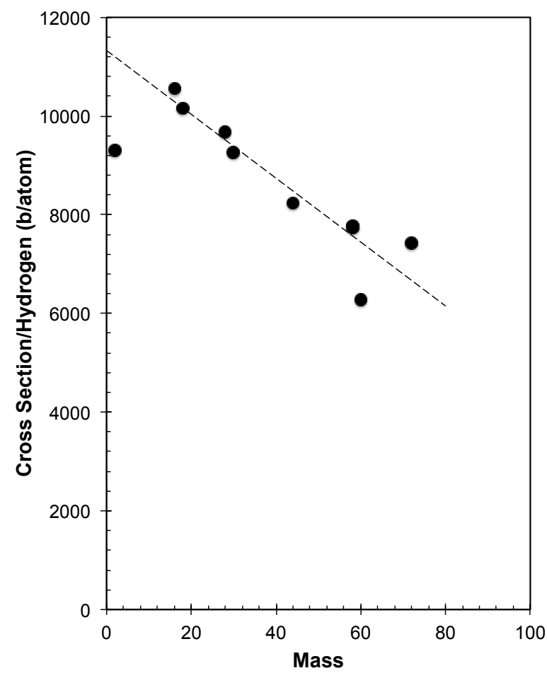
Figure 5: Cross section per Hydrogen atom as a function of molecular mass calculated from our data.
