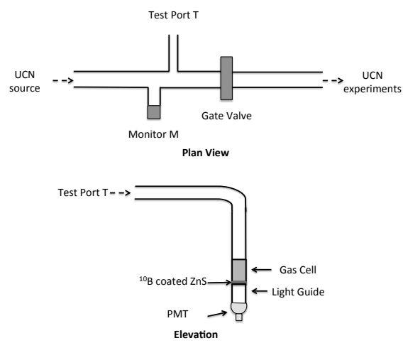
Figure 1: Experimental layout.
