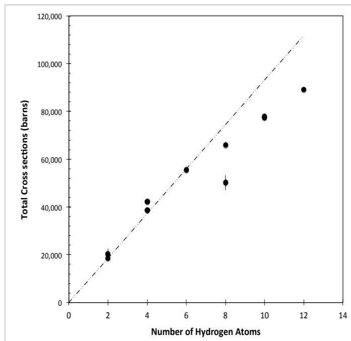
Figure 4: Total cross section as a function of number of hydrogen atoms. The line to guide the eye was chosen to go through the origin and the cross section for hydrogen.
