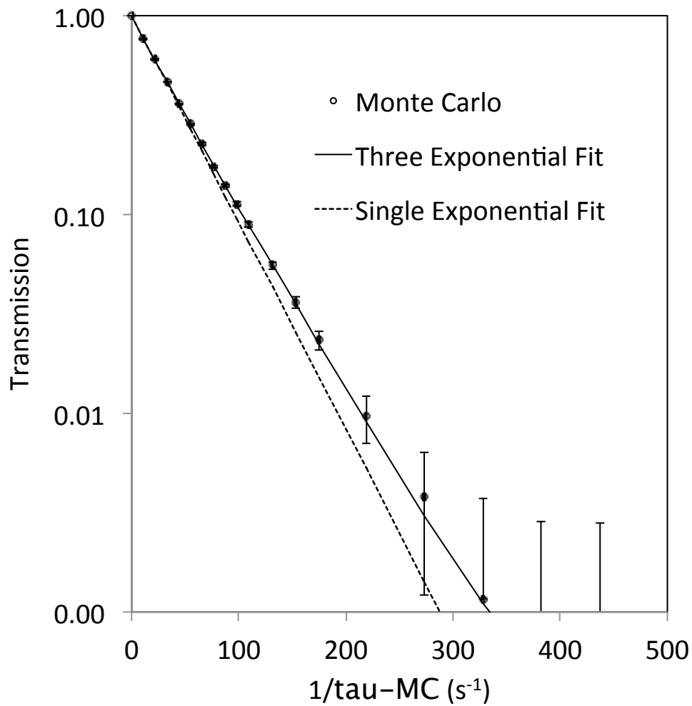
Figure 2: Fits to the Monte Carlo data where the points are for different UCN lifetimes in the gas cell using a simple exponential (dotted line) and a triple exponential function (solid line).
