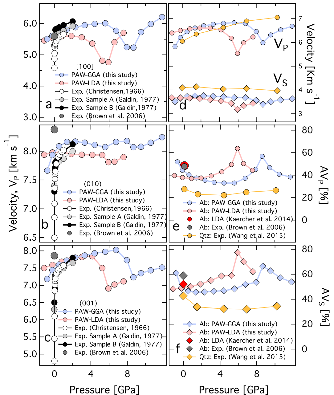
Figure 5. Seismic velocity and elastic anisotropy at high pressure. Compressional wave, V_p propagation directions (a) [100], (b) \perp (010), (c) \perp (001). LDA and GGA results are represented by filled red and blue symbols. Experimentally measured V_p as a function of pressure for albite (An5–8) 38 (open white symbols) and oligoclase (An 10–30) 39 (filled black symbols) to 1 and 2 GPa respectively. The recent experimental results 20 are represented by filled grey symbol. The experimentally measured velocities 38,39 are softer compared to the recent experiments 20 for \perp (010) and \perp (001). (d) Bulk compressional wave V_p and shear V_s velocity as a function of pressure. For comparison, velocities for quartz 51 , a silicate framework mineral is also shown. (e) AV_p and (f) AV_s as a function of pressure. Also shown are the experimentally determined elastic anisotropy for albite 20 and quartz 47 .
