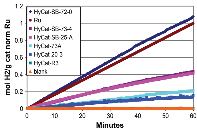
FIGURE 2. Selected NaBH_4 Hydrolysis Microreactor Screening Results
