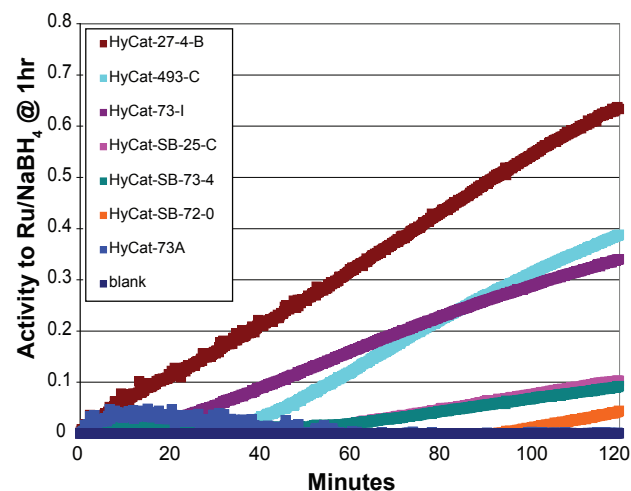
FIGURE 3. Selected NH_3BH_3 Dehydrogenation Screening Results
