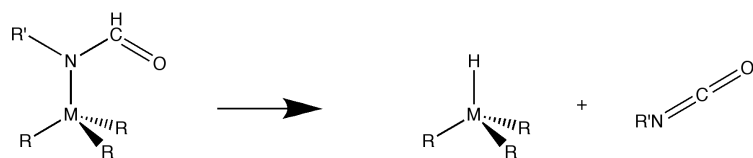
Figure 11: Strategy to replace CO 2 with isocyanate RNCO in tin hydride generation; M = Sn.
