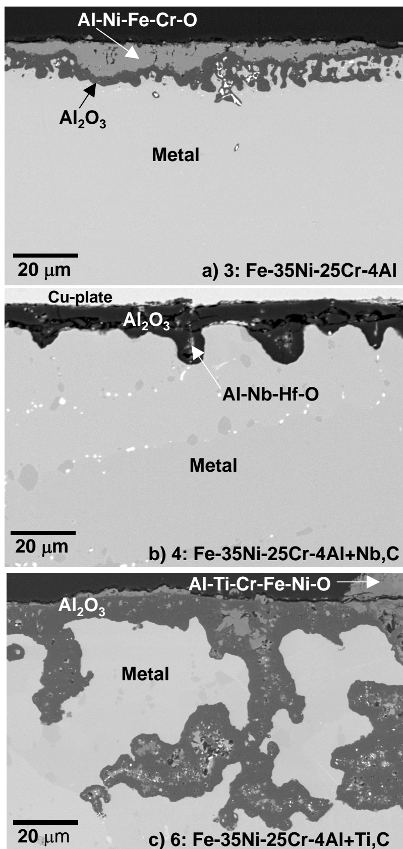
Fig. 2- SEM backscatter mode cross-sections of as-cast Fe-Ni-Cr-Al based alloys after 1000 h (a,c) and 1200 h (b) at 1100°C in air with 10% H 2 O (100 h cycles).
