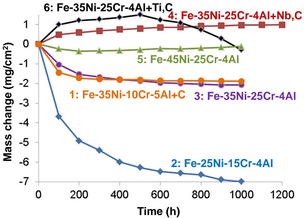
Fig. 1- Mass change at 1100°C in air with 10% H 2 O vs. time (100 h cycles) for as-cast Fe-(35,45)Ni-(10,15,25)Cr-(4,5)Al based alloys with and without C, Nb, Ti additions.
