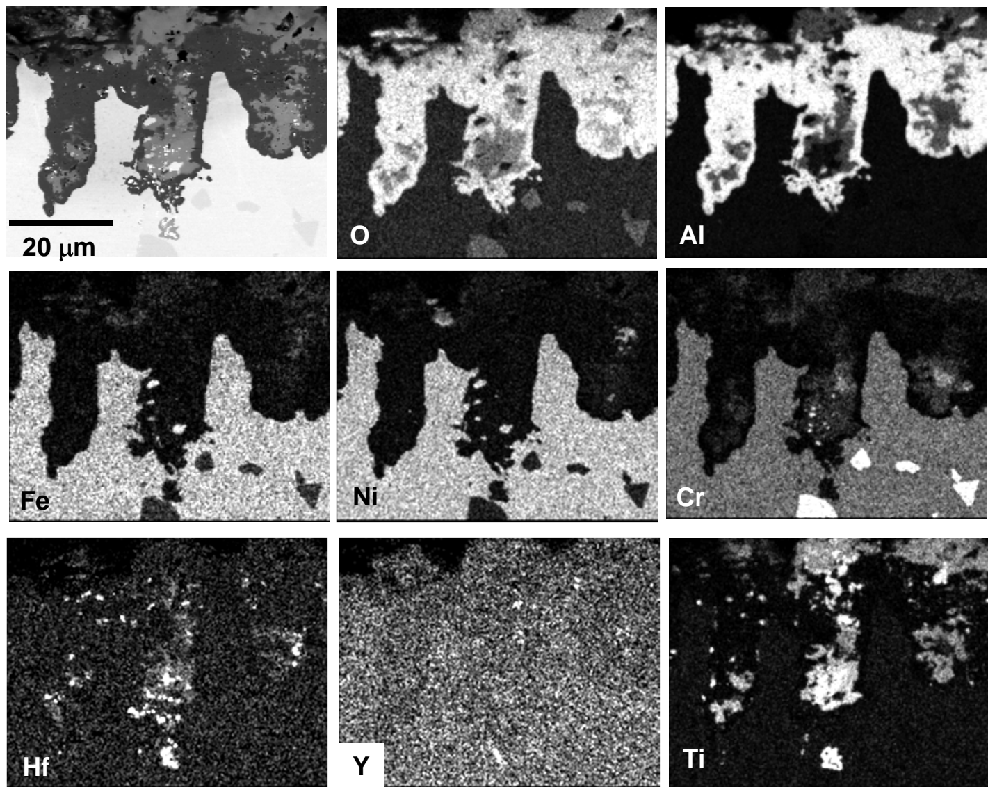
Fig. 4- SEM backscatter mode cross-section and elemental maps of oxide scale formed on as-cast Fe-Ni-Cr-Al based alloy 6: Fe-35Ni-25Cr-4Al+Ti, C after 1000 h at 1100°C in air with 10% H 2 O (100 h cycles).
