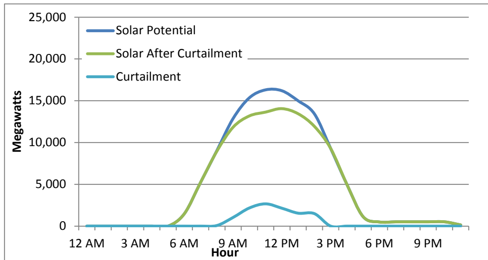
Figure 4. Used and curtailed solar in California on March 29 in a scenario with 11% annual wind and 11% annual solar in a system with limited grid flexibility
