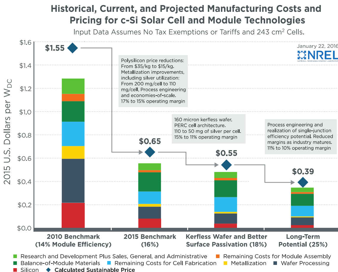
Figure 10. Historical, current, and possible roadmap scenarios for crystalline-silicon module manufacturing cost reductions
