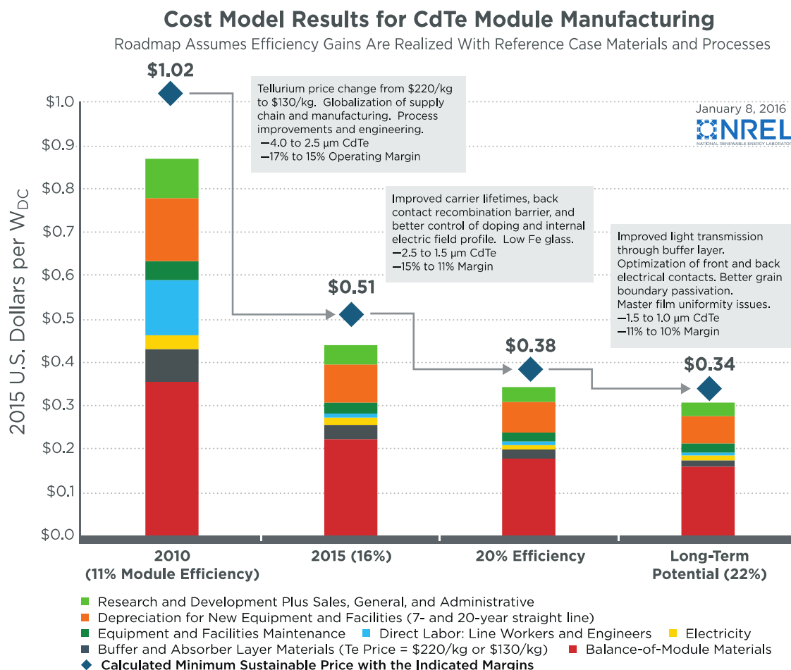
Figure ES-3. Historical, current, and two possible roadmap scenarios for CdTe module manufacturing cost reductions
