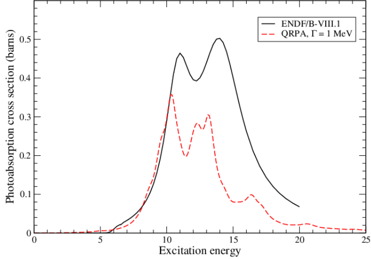
Figure 1. Photoabsorption cross section on the ^{240}\text{Pu} ground state calculated using the QRPA and compared to the ENDF/B-VIII.1 evaluation.
