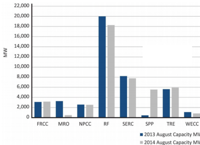
Figure 6.18. Registered demand response capacity (in MW) for all product service types by NERC region 620
