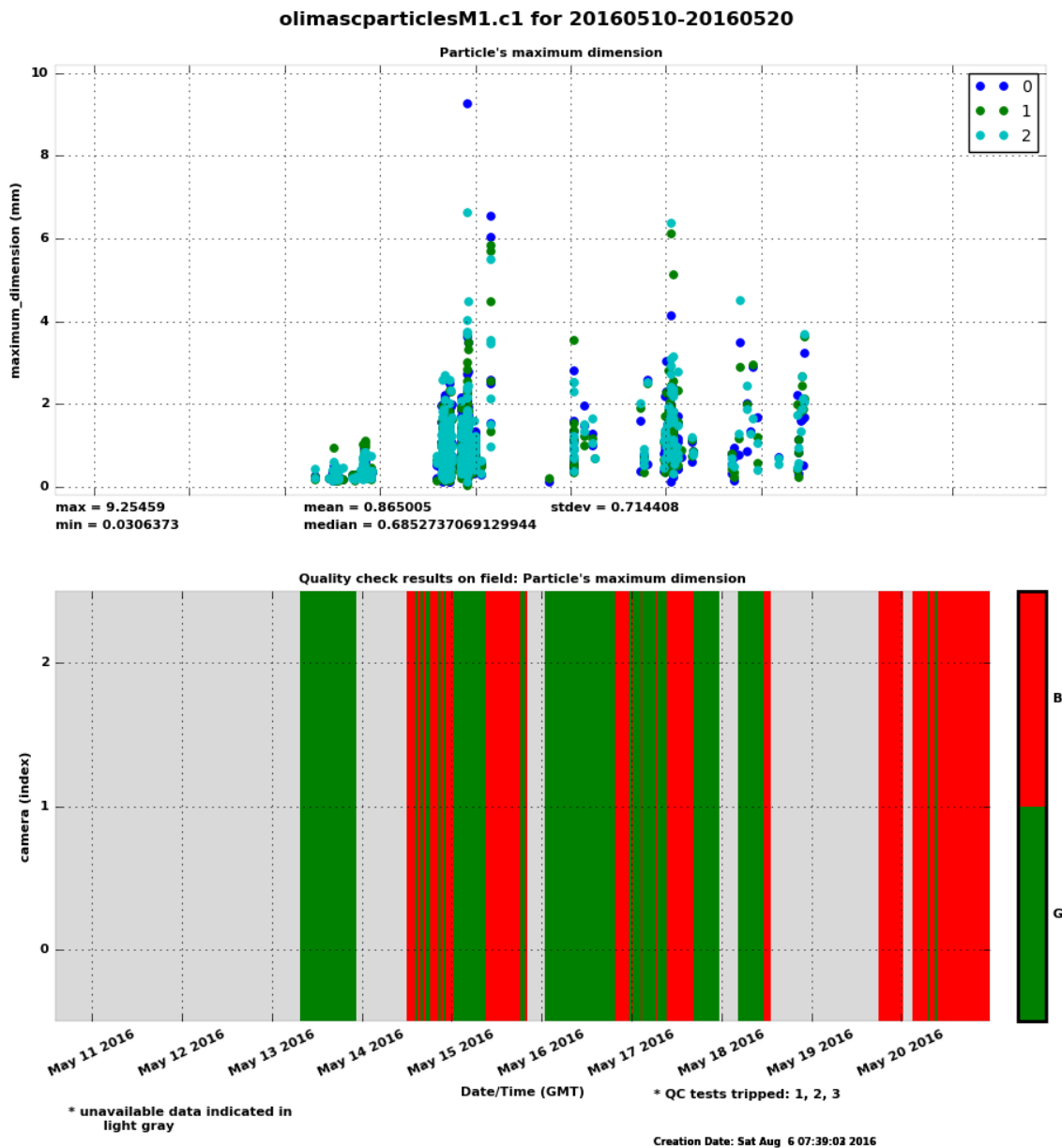
Figure 8. Retrieved maximum dimension for each of the three images for every captured particle (top). Numbers denote camera id. All average quantities are derived from per-image data like this. Quality bits (bottom) for data captured between May 10 and May 20, 2016. See Section 6.0 for description of colors.
