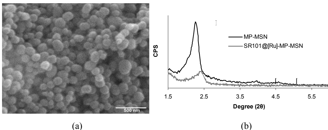
Figure 4. Scanning electron micrograph (SEM) of Sr101@[Ru]-MP-MSN (a) and low angle X-ray diffractograms of MP-MSN and Sr101@[Ru]-MP-MSN (b)
