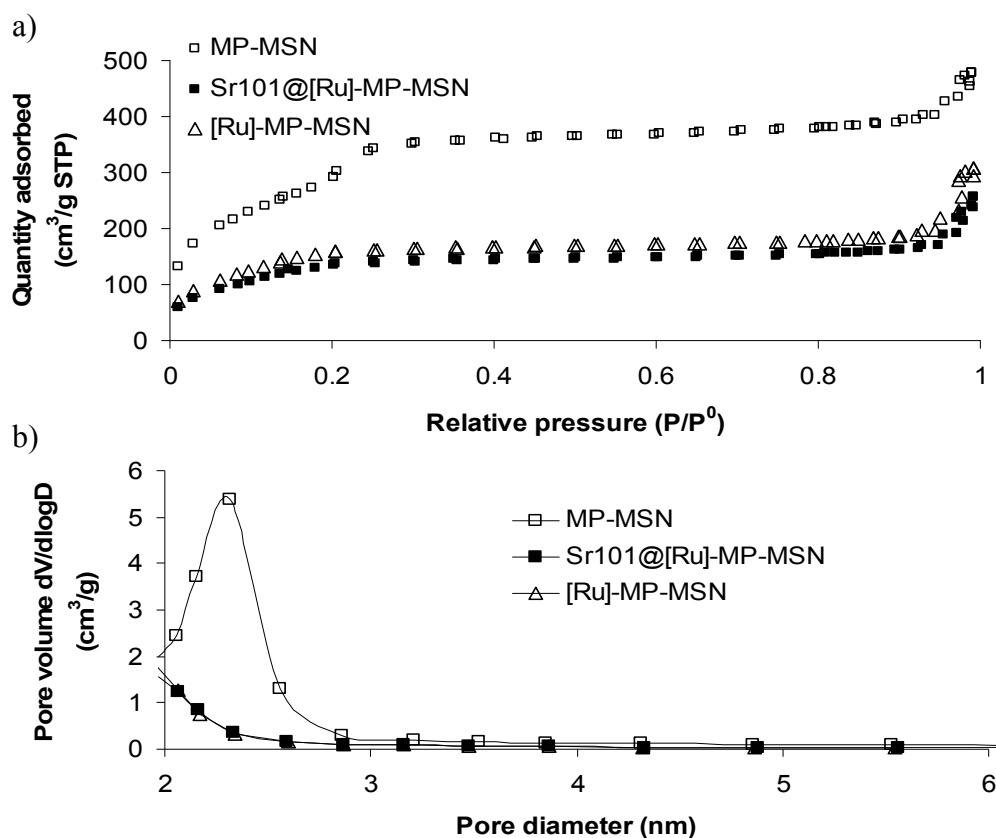
Figure 3. a) BET nitrogen adsorption/desorption isotherms and b) BJH average pore diameters for MP-MSN, \text{Sr101}@\text{[Ru]-MP-MSN} and \text{[Ru]-MP-MSN}
