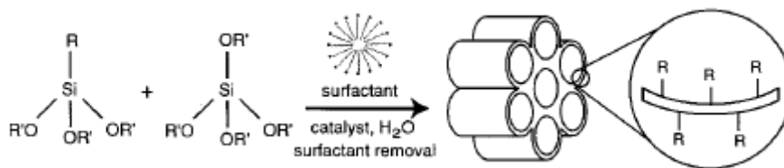
Figure 3. Organic functionalization of MSN by co-condensation
