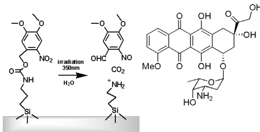
Scheme 1. a) Structural representation of NVCAP-MSN and UV light triggered deprotection of amine groups; b) molecular structure of doxorubicin.
