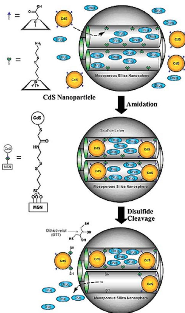
Figure 4. Schematic representation of the CdS nanoparticle-capped MSN-based drug delivery system. 27
