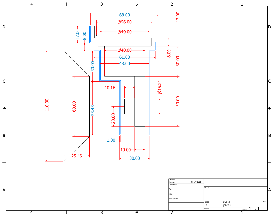
Figure 3.9 Sectional view of the sample holder at the bottom of the cold finger. The trapezoid on the left side is projection of the lens of the electron analyzer. Blue lines are the shielding for the holder.
