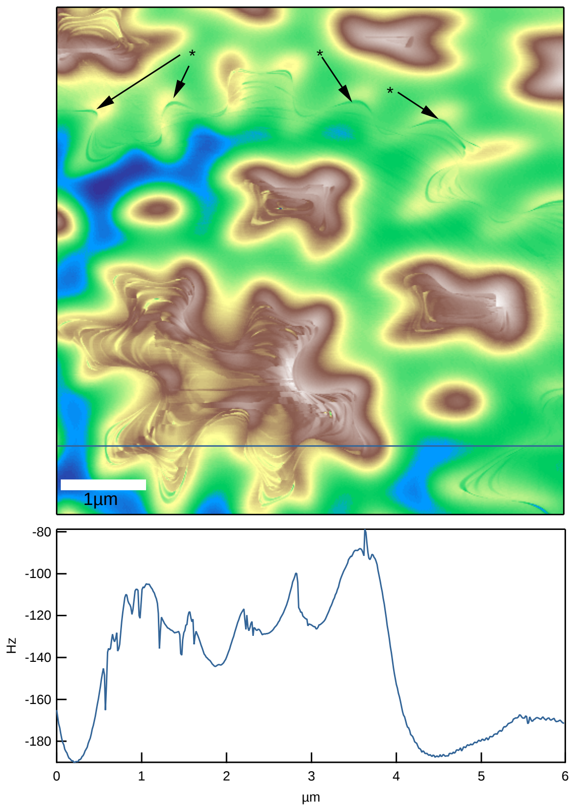
Figure 4.7 (color online). Top: A 6\ \mu\text{m} \times 6\ \mu\text{m} magnetic frequency shift image of the surface of \text{Nd}_2\text{Fe}_{14}\text{B} . Bottom: The z-profile of the blue line in the top graph. Scan height: 300 nm.
