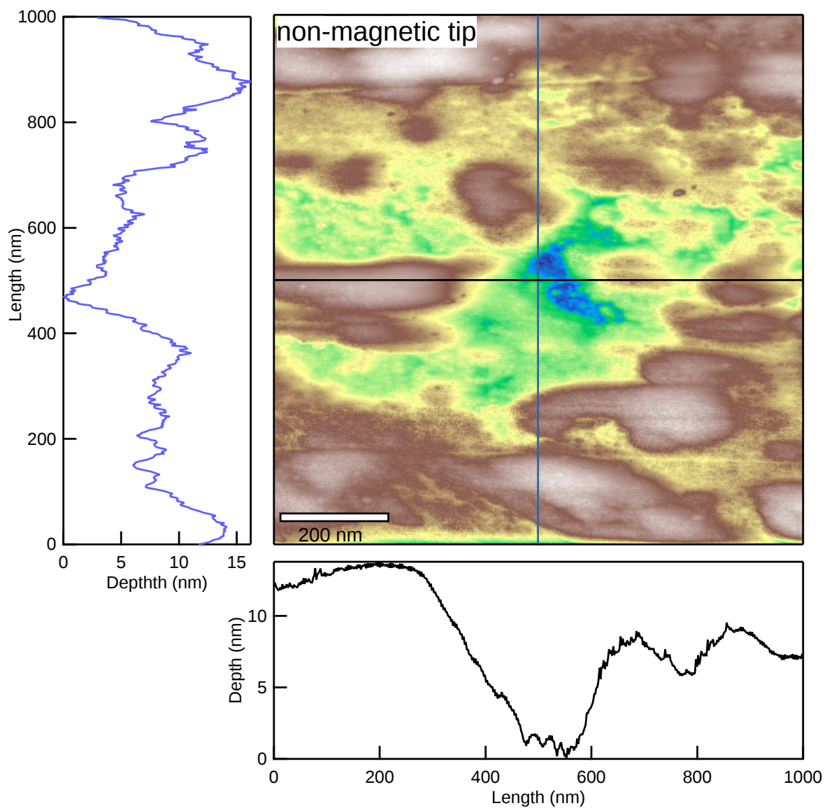
Figure 4.6 (color online). Main: The surface topographic image of \text{Nd}_2\text{Fe}_{14}\text{B} , non-magnetic signal scanned by the AFM Non-contact-tip, z mode. 1\ \mu\text{m} \times 1\ \mu\text{m} scan, the z range is 18 nm. Left: The z-profile along the vertical line in main. Bottom: The z-profile along the horizontal line in main.
