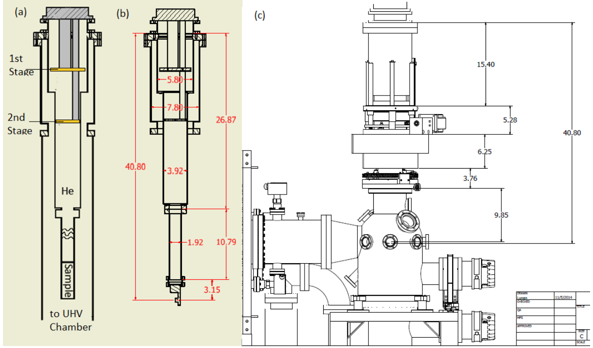
Figure 3.5 Cold finger design. (a) A schematic drawing of the cold finger. (b) A detailed drawing with main dimensions marked. (c) A schematic drawing of the cold finger installed on the ARPES system. The units in (b) and (c) are inches.
