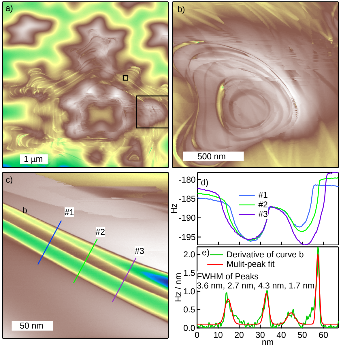
Figure 4.11 (color online). (a) A frequency shift image ( 6\ \mu\text{m} \times 5.5\ \mu\text{m} ) measured using magnetic tip 300 nm above the surface of \text{Nd}_2\text{Fe}_{14}\text{B} . (b) A zoom-in from the larger box area marked in (a) (scanned area 1.37\ \mu\text{m} \times 1.37\ \mu\text{m} ). (c) A zoom-in from the smaller box area marked in (a) (scanned area 200\ \text{nm} \times 200\ \text{nm} ). (d) The z-profile along the three cuts indicated in (c). (e) The derivative of the curve #2 in graph (d) and multi-peak fit.
