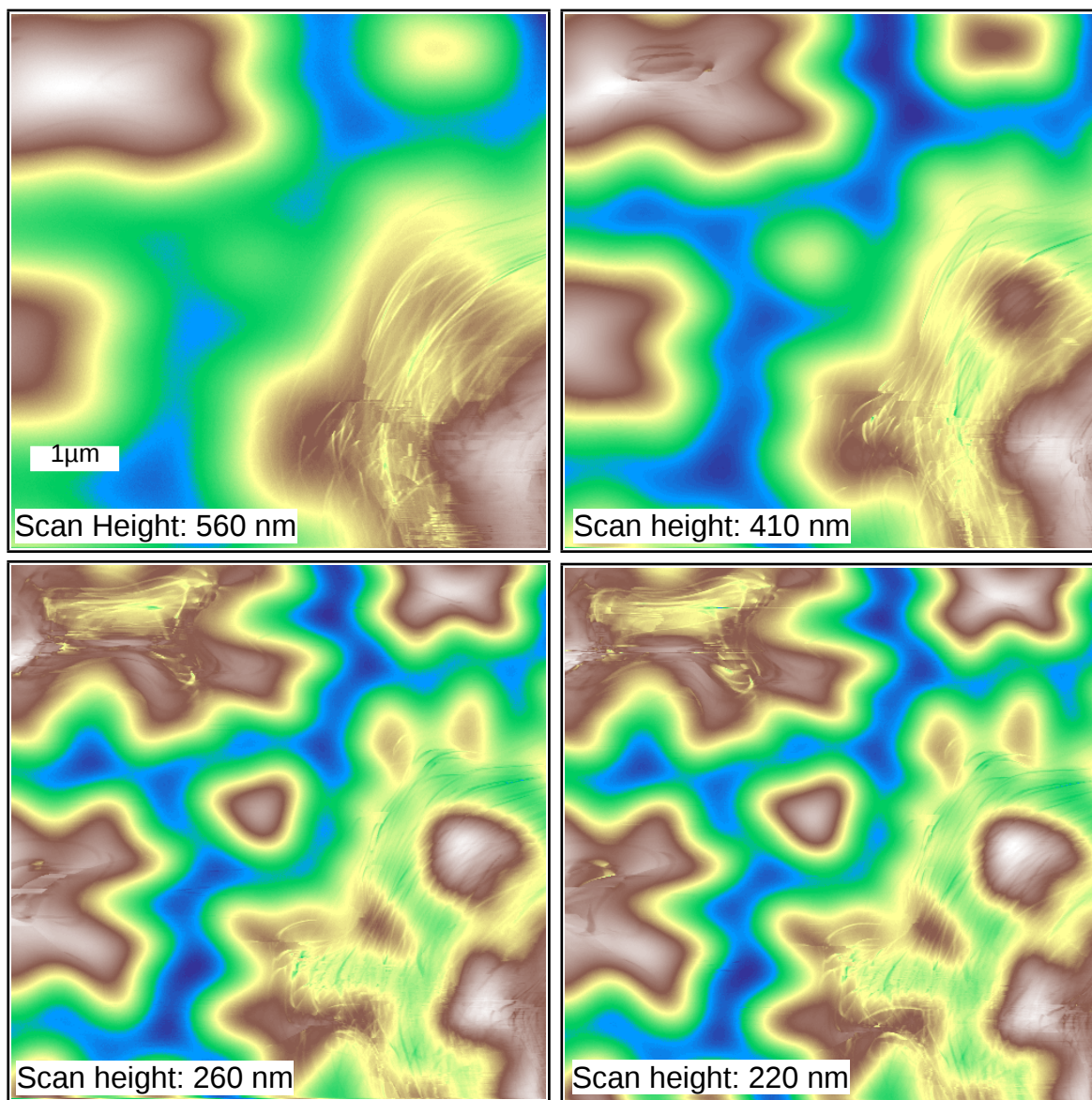
Figure 4.8 (color online). The same position on the sample is scanned at different tip-sample distances ( 6\ \mu\text{m} \times 6\ \mu\text{m} ; And scan heights are (From left top to right bottom) 560 nm, 410 nm, 260 nm and 220 nm, respectively).
