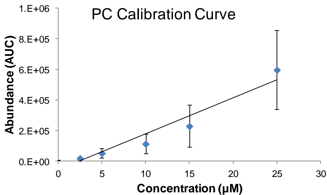
Figure 2C. Phosphorylcholine calibration curve. Calibration curve for phosphorylcholine using standards ranging in concentration from 2.5 \mu\text{M} to 25 \mu\text{M} .
