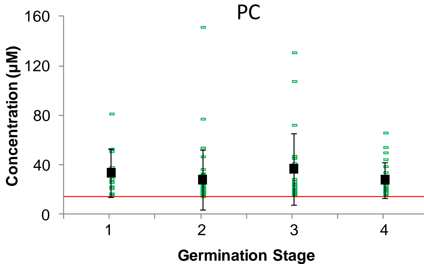
Figure 5C. Abundance of phosphorylcholine in seed exudates. Individual data points are shown in green, the average value is in black, and the LOQ is shown as a red line.
