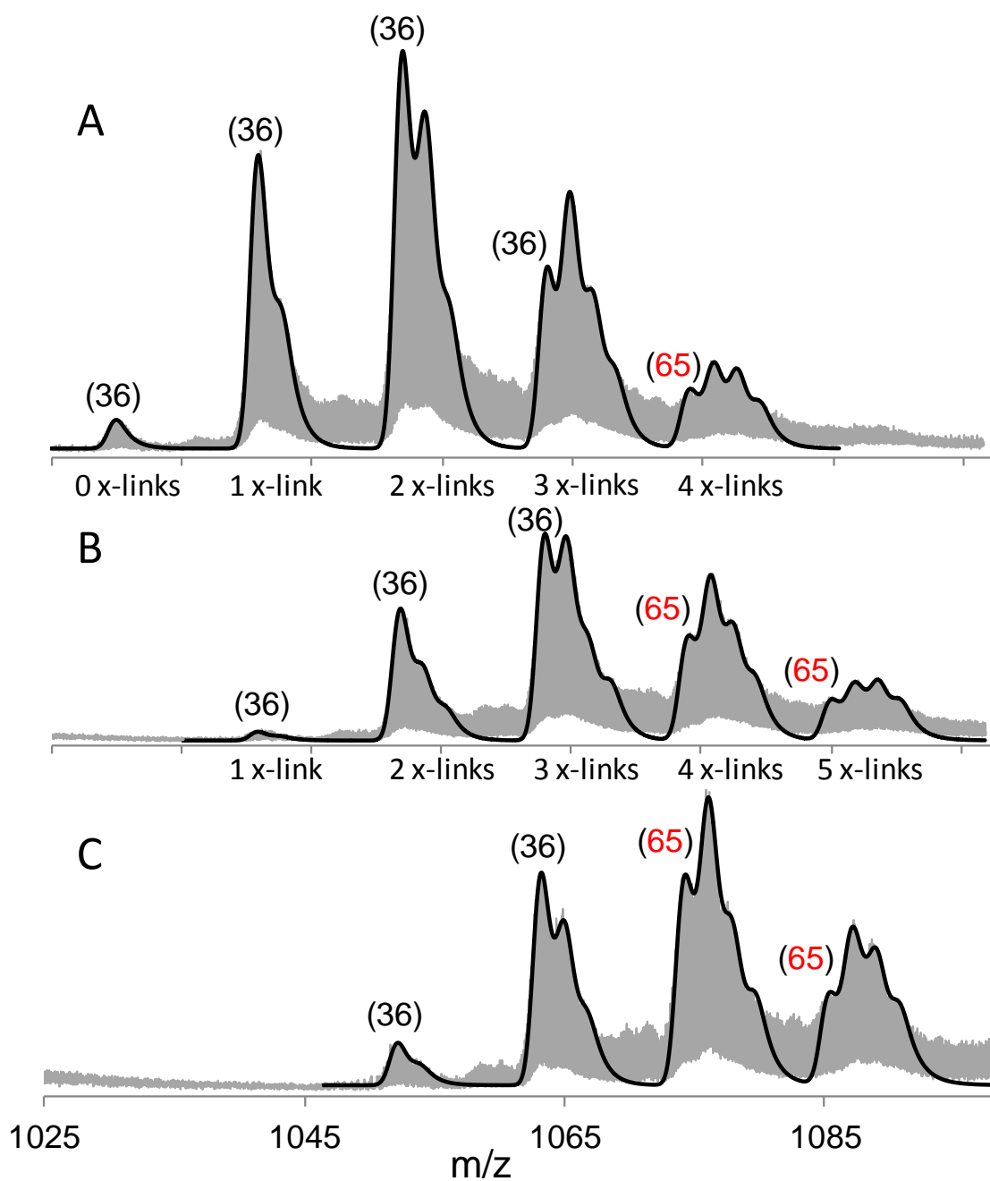
Figure 2. HDX/MS of cross-linked cytochrome c. The 12+ series of HD exchanged cytochrome c (gray line) after cross-linked with DSS (100:1 molar ratio) for (A) 10 minutes, (B) 30 minutes, and (C) 60 minutes compared with the best fitted EMG (solid line). Best fitting tau values are shown in parentheses.
