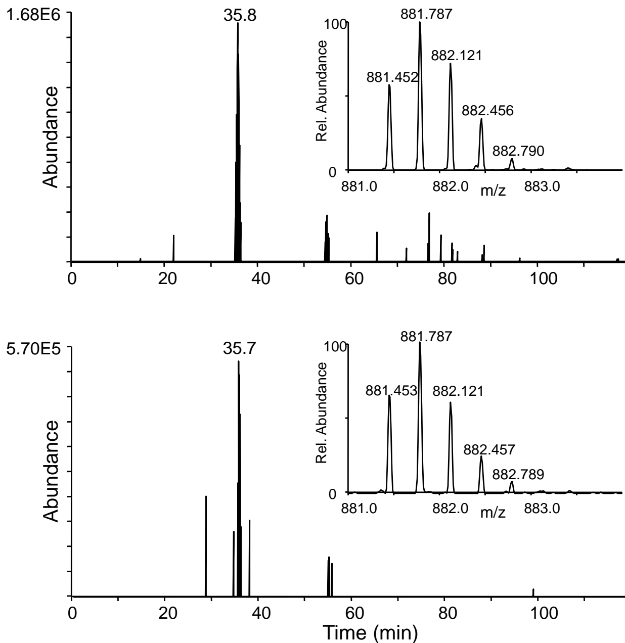
Figure 3. Extracted ion chromatogram of m/z 881.4535. XIC of m/z 881.4535 ([TGQAPGFSYTDANKNK-KYIPGTK + 3H] 3+ ) for the data set at (A) 45°C/100:1 and (B) 25°C/20:1 reaction conditions. Mass tolerance of 0.004 Da was used for XIC generation. Zoomed-in inset precursor mass spectra were obtained averaging over the retention time of 35-36min.
