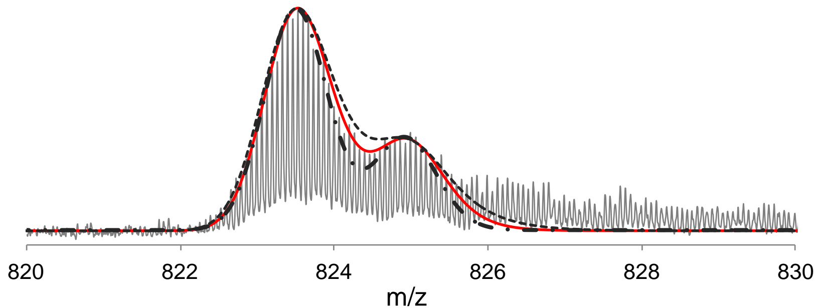
Figure S2. EMG fitting. The mass spectrum for the 15+ ion of cytochrome c (gray line) compared with best fitting EMG profile ( \tau=12 , red line) and EMG profiles with 10% narrower ( \tau=4.5 , dot-line) and 10% broader FWHM ( \tau=19.5 , dashed line).
