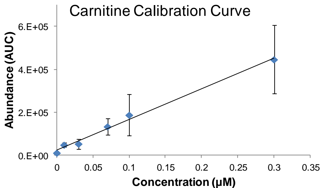
Figure 2B. Carnitine calibration curve. Calibration curve for carnitine using standards ranging in concentration from 0.01 \mu\text{M} to 0.3 \mu\text{M} .
