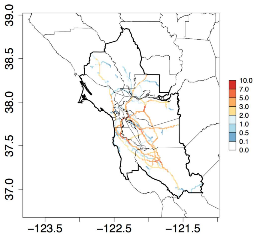
Figure 19. On-road \text{CH}_4 emissions (nmol/m 2 /s) on the 1-km BAAQMD grid.
