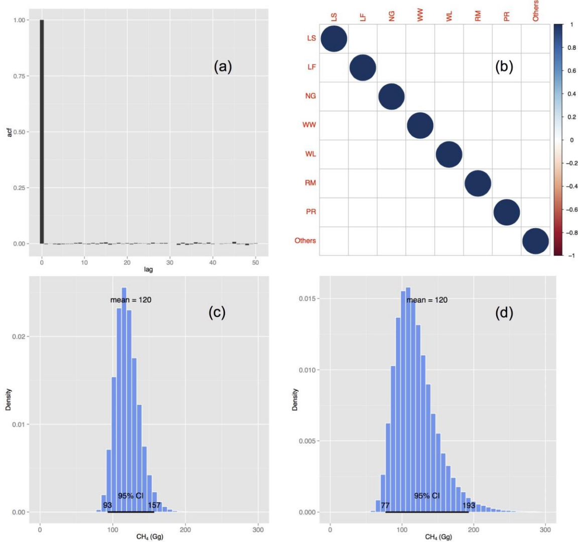
Figure 26. (a) autocorrelation function for the combined total \text{CH}_4 samples, (b) cross-correlation between different sectors (white color indicates no correlation), (c) histogram for the combined total \text{CH}_4 using 1 sd error from the US EPA uncertainty, and (d) histogram for the combined total \text{CH}_4 using 2 sd error from the US EPA uncertainty.
