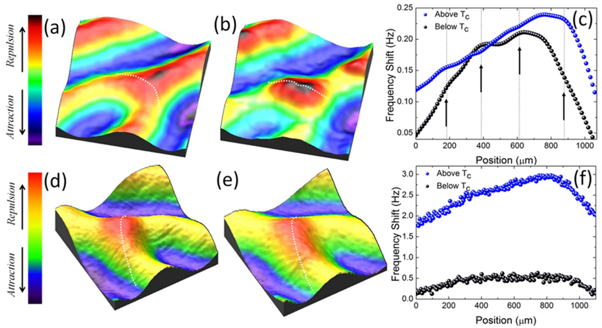
Figure 2. Magnetic contrast at magnetic stripe bifurcation. (a)–(b) 3D zoom-in of MFM maps acquired at T = 13 K and T = 6 K on Nb(200 nm)/Py(1 \mu m), focusing on the stripe bifurcation; (c) magnetic profile taken along white dotted lines of (a) and (b). Blue and black dots show the profiles above and below T_c , respectively. Arrows point at possible vortex position inside the cluster. (d)–(e) 3D zoom-in of MFM maps acquired at T = 13 K and T = 6 K on Nb(100 nm)/Py(1 \mu m), focusing on the bifurcation; (f) magnetic profile taken along white dotted lines of (d) and (e). Blue and black dots draw the profiles above and below T_c , respectively. Each map is 2 \mu\text{m} \times 2 \mu\text{m} in size.
