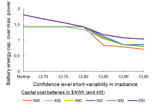
Fig. 6 Energy capacity over rated output of installed batteries
