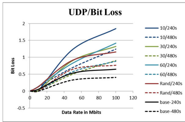
Figure 1. UDP Bit Loss Measurements
