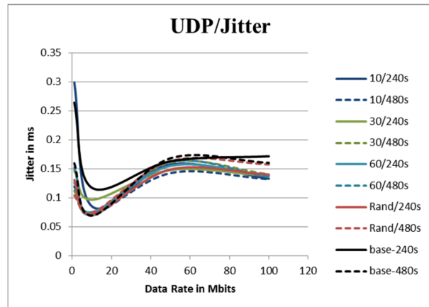
Figure 2. UDP Jitter Measurements
