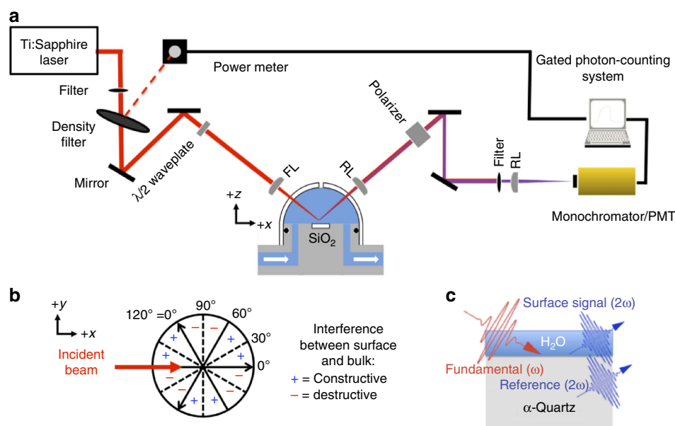
Figure 1 | Experimental setup. (a) Depiction of the external reflection geometry and the flow cell enabling this work. FL, focal lens; RL, recollimating lens. (b) Top view of right-handed z-cut \alpha -quartz as placed across the plane of incidence and depiction of the sign of the interference between surface and bulk signals. (c) Depiction of the phase-referencing process used to unveil the newly identified term i\chi^{(3)} \times \Phi(0) .
