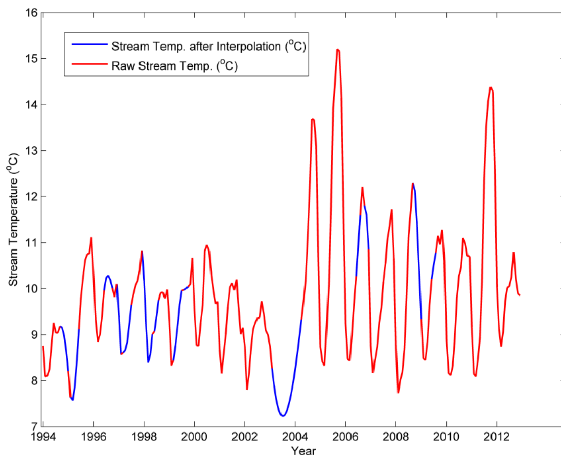
Figure 2.9 Time series of historical stream temperature data after filling missing values at a station Lees Ferry on the Colorado River in the state of Arizona
