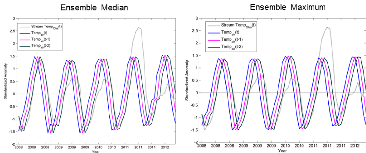
Figure 2.11 Observed stream temperature, current and lagged air temperatures during validation phase for the Lee's ferry station on the Colorado River
