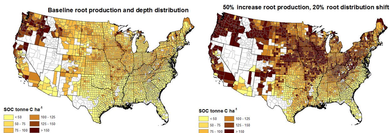
Fig. 6. Geographic distribution of steady-state soil organic C stocks (0-200 cm) on cropland and pasture/hay land under baseline (i.e. current) conditions and under a scenario for 50% increased root C inputs and moderately deeper root distributions.
