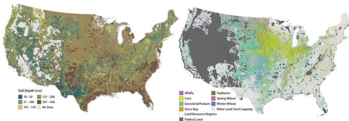
Fig. 4. Soil depth for potential rooting (derived from SSURGO) and distribution of major crop types (derived from CDL) used in the analysis.
