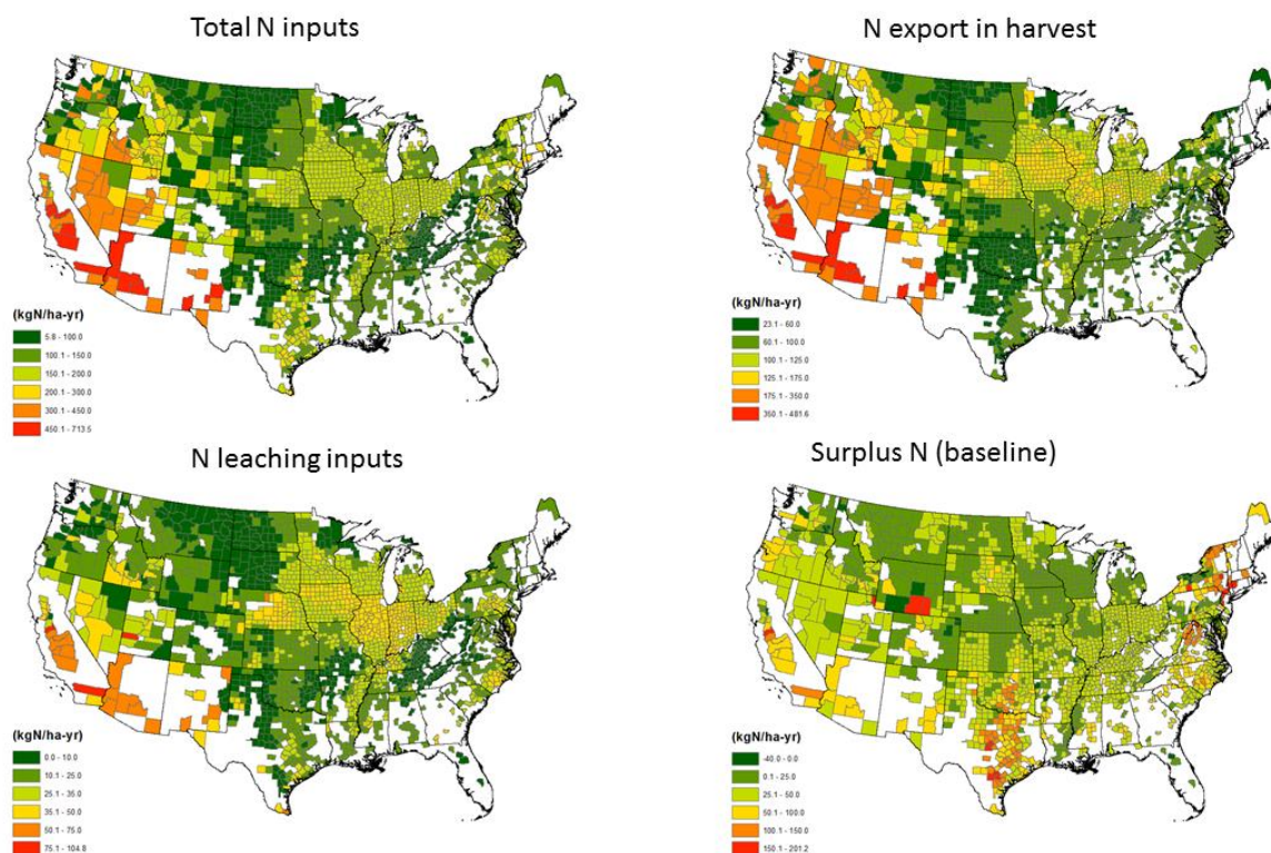
Fig. 9. Nitrogen balance components, showing average annual N flux rates for cropland included in the analysis. Values are in kg N ha -1 yr -1 for cropland in counties containing more than 10,000 acres in a county.
