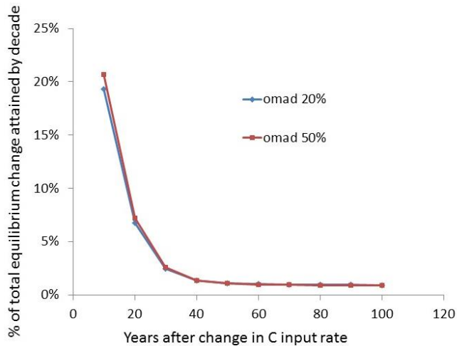
Fig. 7. Change in the relative rate of SOC accumulation (as a percentage of the difference between equilibrium soil C stocks) for the transition to a new equilibrium following a change in C input rates (+20% and +50% above baseline, respectively) for the Wooster, OH site. Simulations were run for 5000 yr – only the first 100 year period is shown here.
