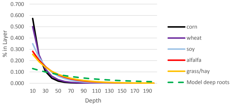
Fig.2. Baseline root distributions for all plant types included in this analysis, using parameter values from Table 2.
