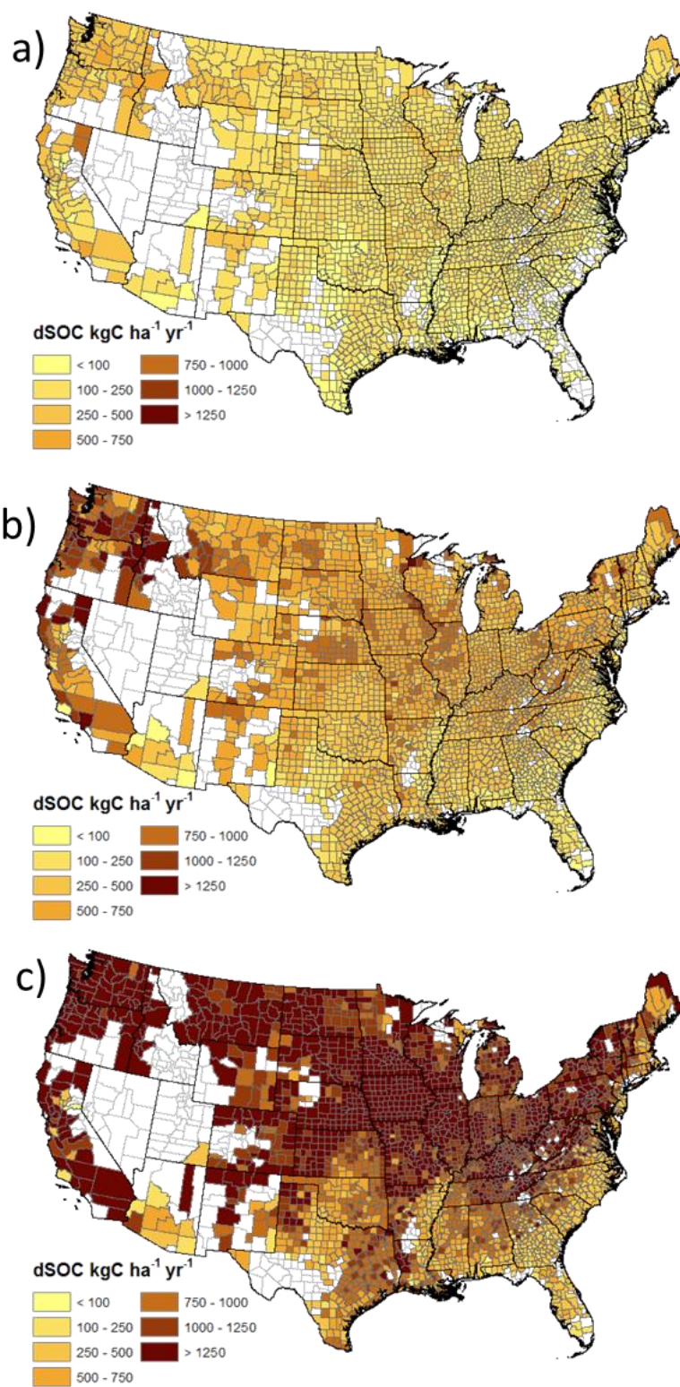
Fig. 8. Annual delta SOC (kg C ha -1 yr -1 ) over the 30 year projection period for: a) 25% production increase, no shift, b) 50% production increase, 20% shift, c) 100% production increase, strong shift.
