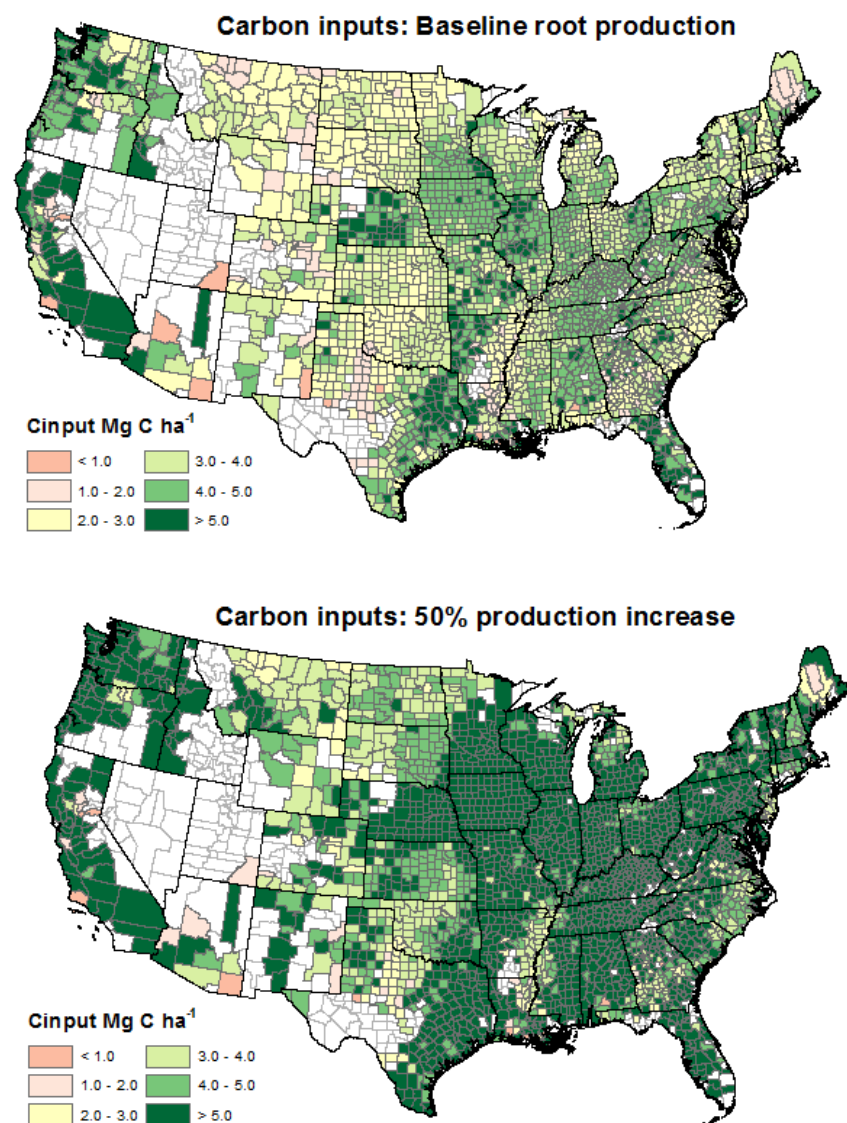
Fig. 5. Baseline average annual residue C inputs (top) based on CDL reported crop histories (2010 – 2015) and residue C under the 50% increased root production scenario (bottom).
