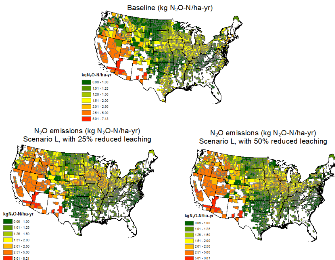
Figure 11. N 2 O emissions under baseline (current) conditions vs N 2 O emissions projected for the scenario with 50% increase in root C inputs and a 20% downward shift in root distribution, including with a 25% decrease (bottom left) or a 50% decrease (bottom right) in N leaching.
