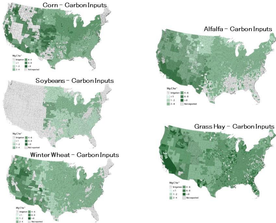
Fig. 1. Average county-scale baseline plant C inputs (above-ground + below ground) for each major crop type.
