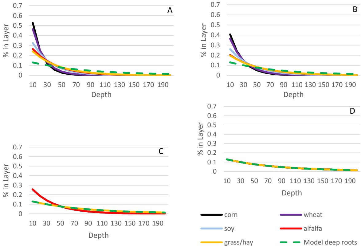
Fig. 3. Root distributions for scenario 1 (A), scenario 2 (B), scenario 3 (C) and scenario 4 (D), showing percentage allocation of root biomass in each layer to 200cm.
