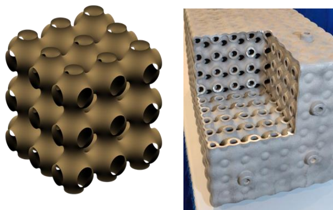
Figure 1. The Schwarz P-surface structure of the REL conformable tank, shown schematically and in cross section on a demonstration tank
