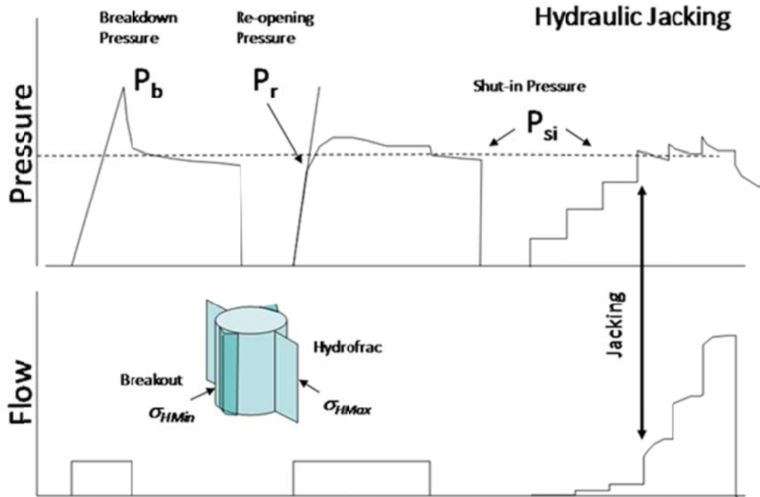
Figure 5.13. Idealized hydraulic fracturing pressure-time record. Inset shows location of triangular prismatic borehole breakouts relative to horizontal stress directions.
