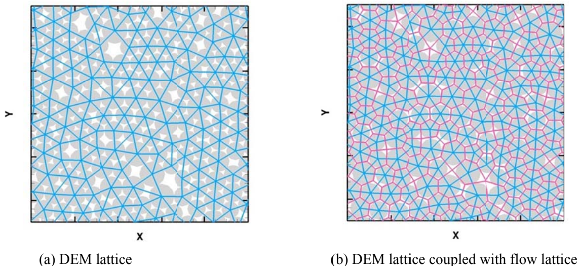
Figure 4.1. The concept and construction of the dual lattice system. In both figures, the grey circles represent randomly distributed DEM particles. The blue lines (elastic beams) connecting DEM particles represent the DEM lattice. The red lines in (b) are the conjugate flow lattice.
