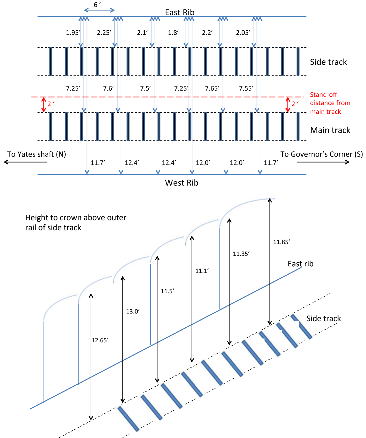
Figure 2.9. Dimensions of site (in decimal ft) on the West Access Drift of 4850L selected for kISMET.
