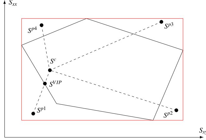
Fig. 2 A simplified 2D schematic of the VIP algorithm for tensors with unlimited reconstructed values in cell nodes S^{p1} \dots S^{p4} , cell-centered average value S^c and the closest limited value S^{VIP} , compared with component-wise limiting set (red).
