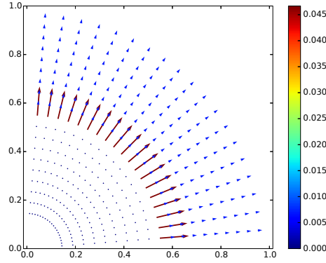
Fig. 4 Initial elastic force distribution shown in the internal nodes of the 20 \times 20 mesh, force vectors are colored according to magnitude.
