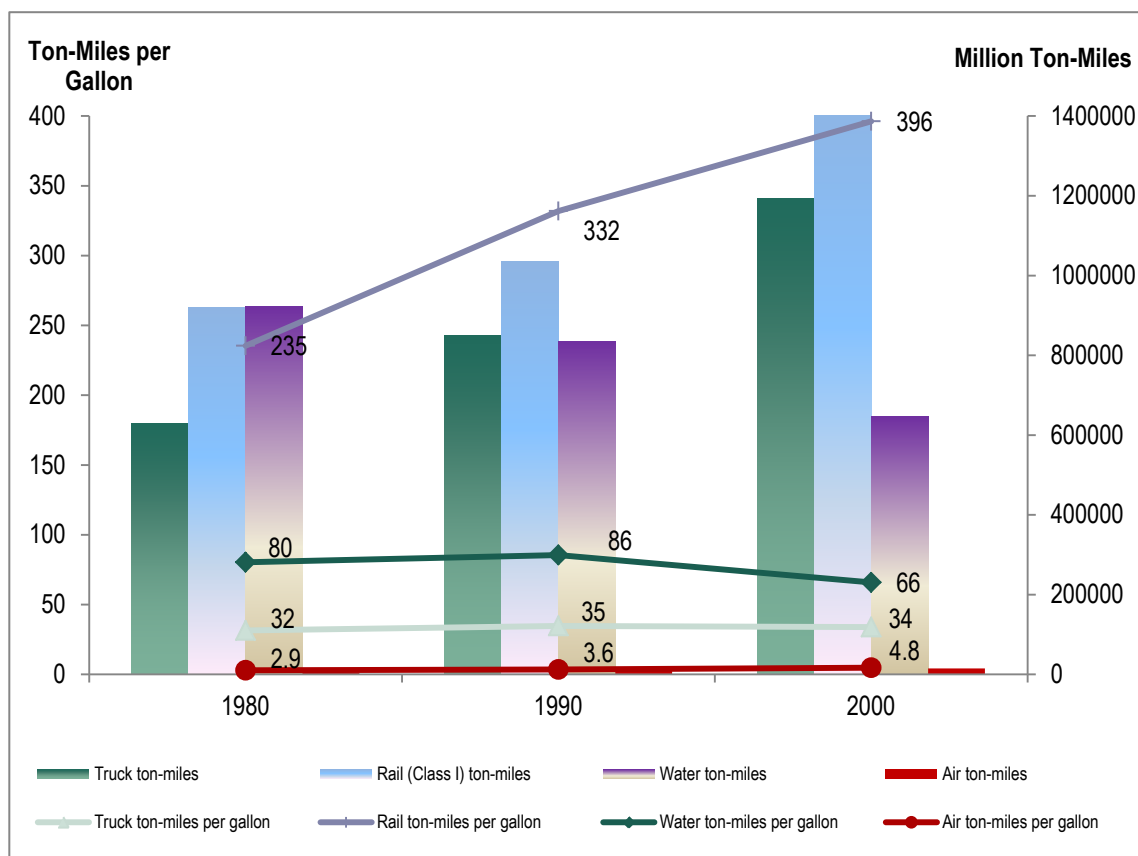
Figure 3.2. Freight ton-miles per gallon and ton-miles traveled, 1980 to 2000
