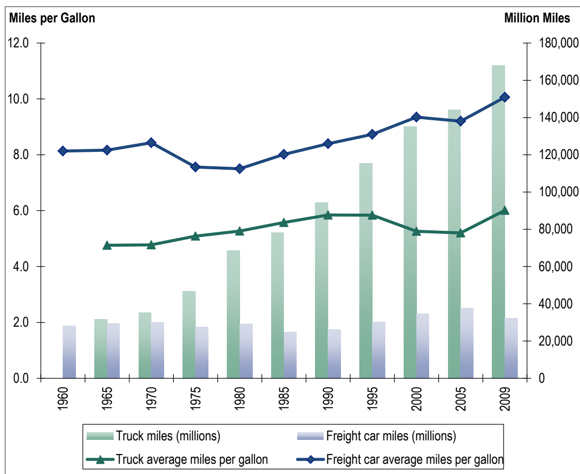
Figure 3.1. Freight truck and rail miles per gallon and miles traveled, 1960 to 2009
