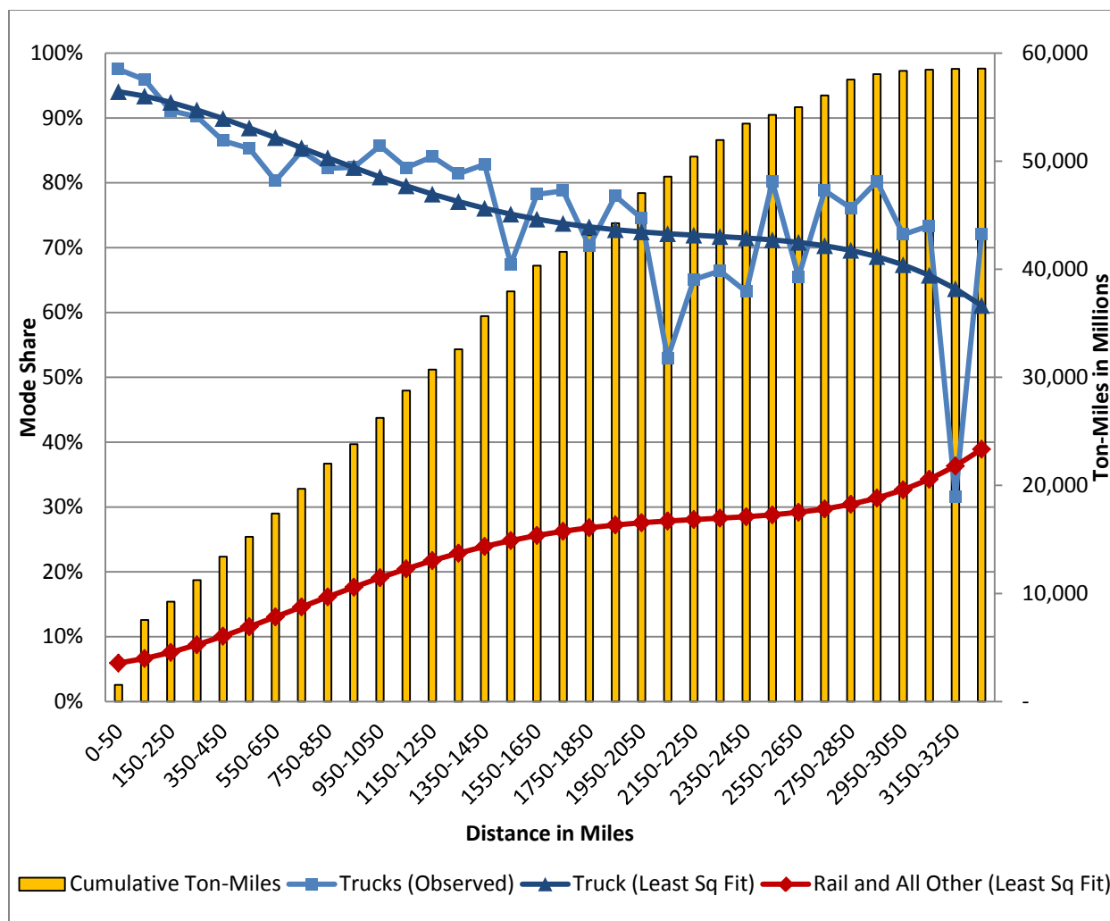
Figure 2.8. Freight modal shares and ton-miles by distance for machinery (commodity group 34), 2007
