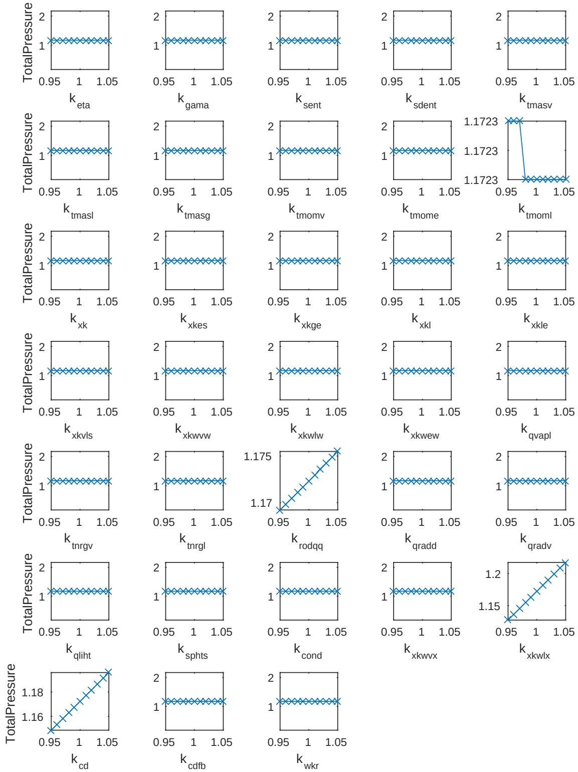
Figure 7.1: Sensitivities of TotalPressure to each of 33 variables varied over \pm 5\% in a centered parameter study. Note that most parameters had identically zero variation and k_{\text{tmoml}} has only very slight variation.
