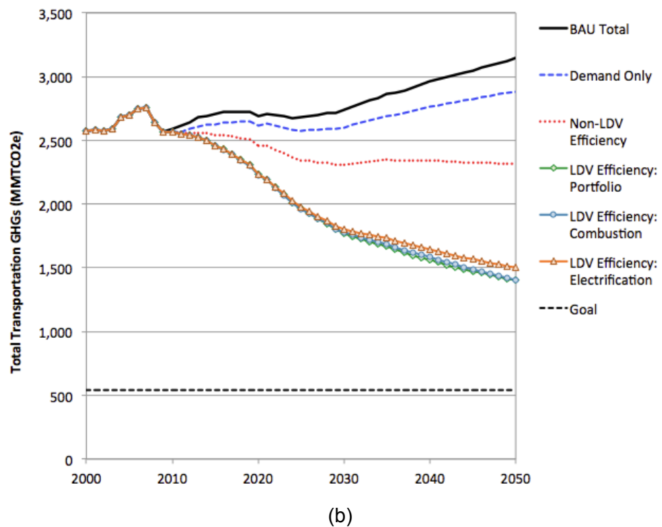
Figure 3.12. Fuel use reductions (a) and GHG reductions (b) due to demand reductions and efficiency improvements, and with carbon intensities of conventional fuels
