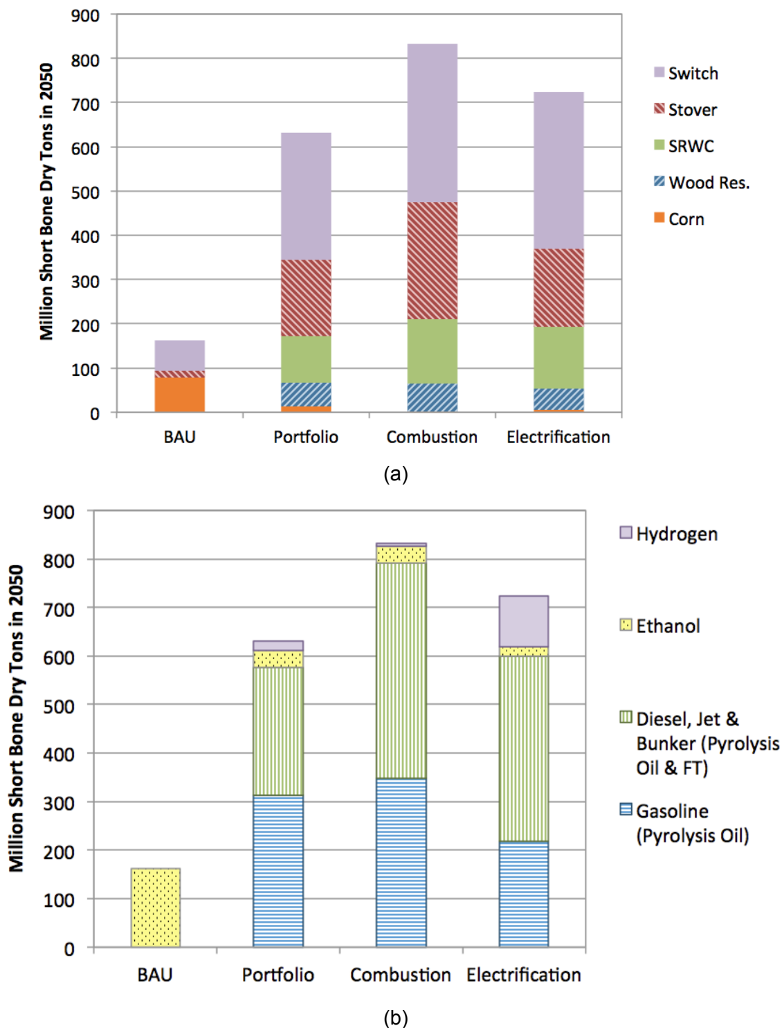
Figure 4.4. Summary of biomass resource use for all scenarios in 2050 by (a) resource type and (b) fuel type
