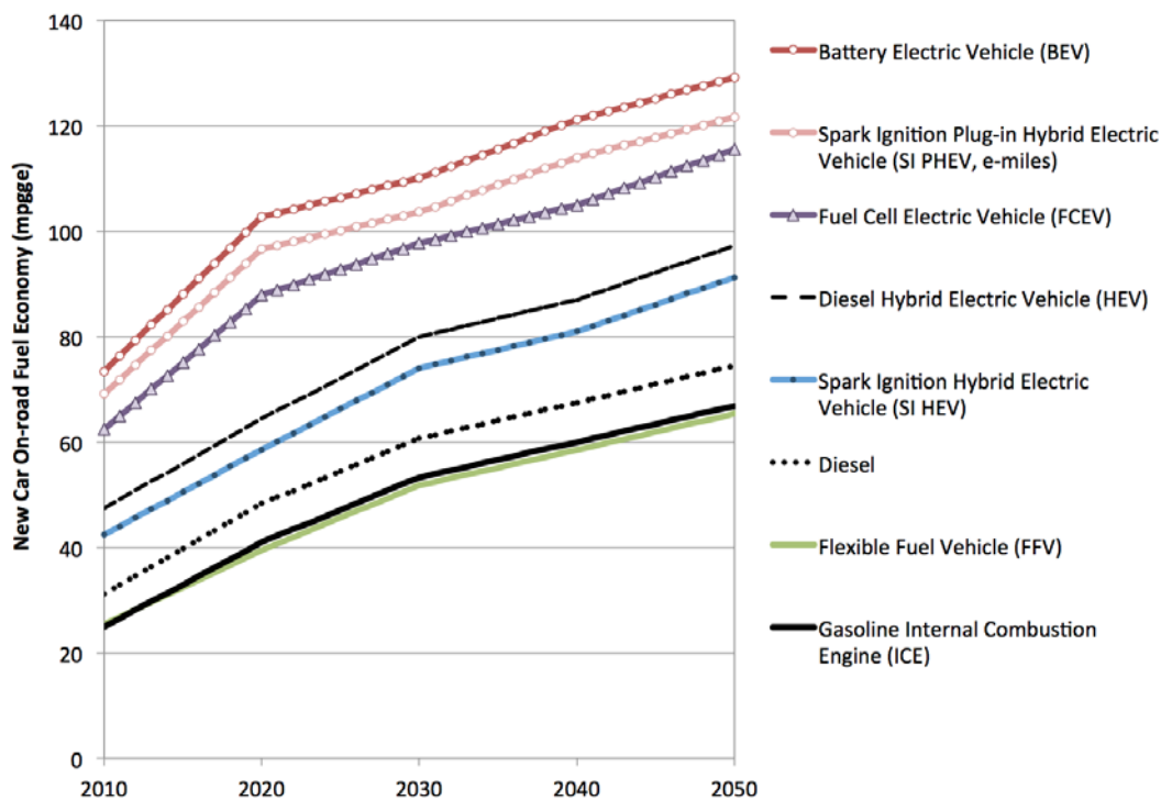
Figure 3.6. New car on-road fuel economy for the low-carbon scenarios
