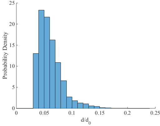
Figure 4. Measured Drop Size Probability Density Functions. Calculated for all secondary droplets detected at We = 784 , \tau = 5.1 .
