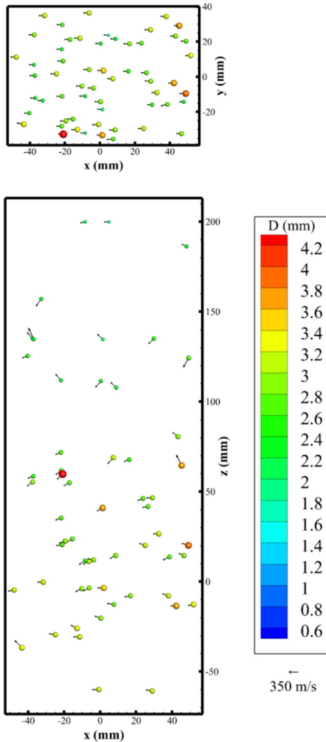
Figure 8. Shotgun Experiment Vector Plot. Front and top views of the same shotgun pellet firing. As expected, the detected pellet size shows a small variation and the motion is primarily in the x direction.
