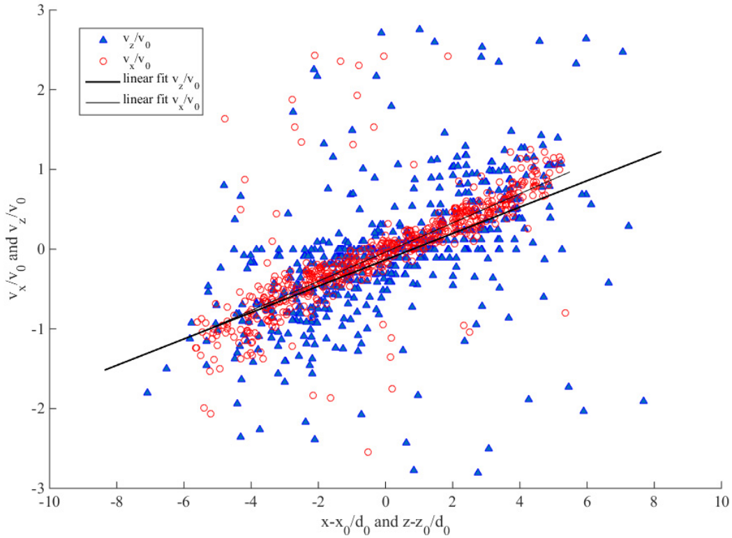
Figure 5. Measured Non-Dimensional Particle Velocities. Measured non-dimensional particles velocities v_x/v_0 and v_z/v_0 plotted as a function of non-dimensional distance from the mean (x-x_0)/d_0 and (z-z_0)/d_0 . Linear fits of v_x/v_0 and v_z/v_0 are overlaid on the plot. For clarity, only 10 percent of the calculated points are plotted.
