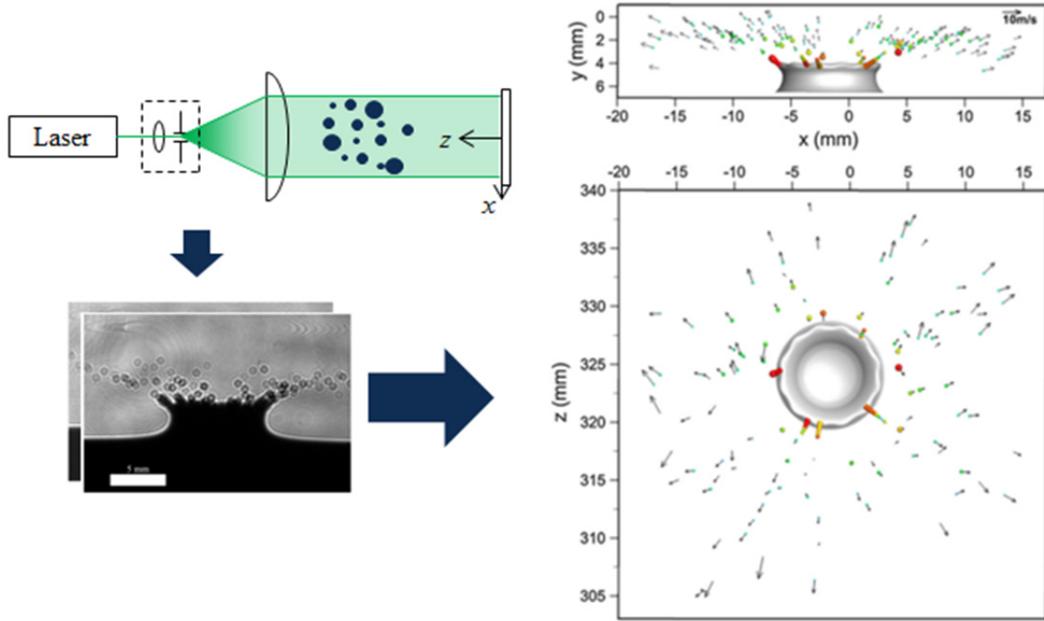
Figure 1. Digital In-line holography (DIH) experimental configuration (top left), example hologram of the splash and secondary fragments when a water drop impacts on a thin film of water (bottom left), and the 3D particle field reconstructed from this hologram (right). 4
