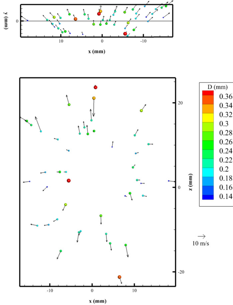
Figure 3. Measured three dimensional droplet sizes and velocities. Front and top views of the same drop impact, displaying the expected symmetry of the secondary droplet motion in all direction. Several erroneous vectors can also be identified.
