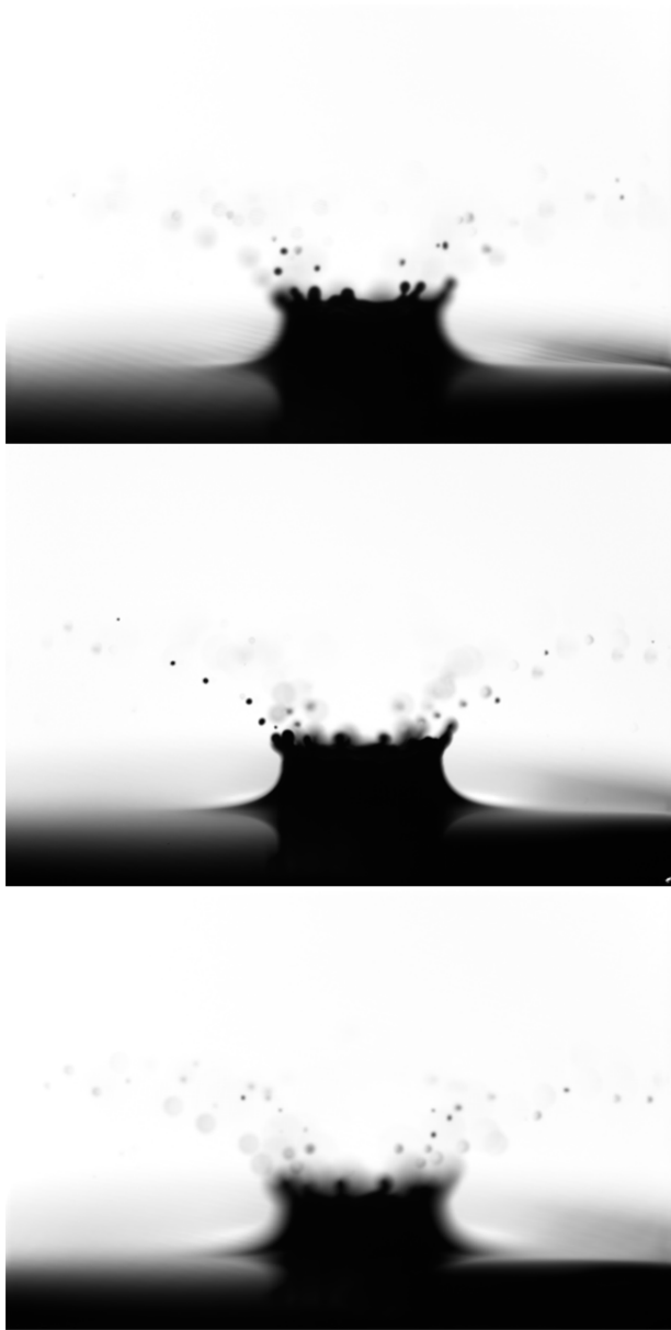
Figure 2. Refocused Drop Impact Images. A single raw plenoptic image refocused to three different planes.
