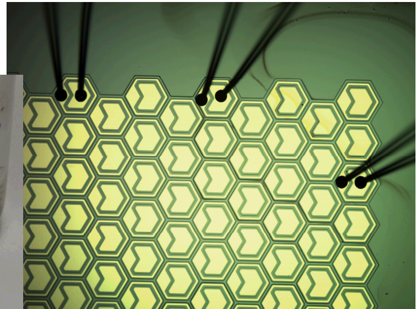
GaAs microscale PV cells on wafer and being tested
