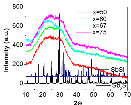
Figure 12. PXRD results of the consolidated product obtained from iodine laden chalcogel with varying weight percentages of \text{Sb}_2\text{S}_3 .
