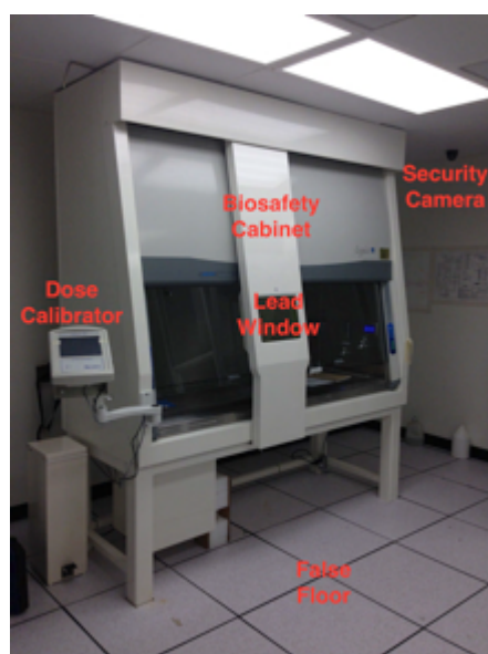
Figure 5. Shielded Class II, B2 Biosafety Cabinet. Protects samples and the environment through HEPA filters and pressure differentials with full exhaust (1100 cfm).
