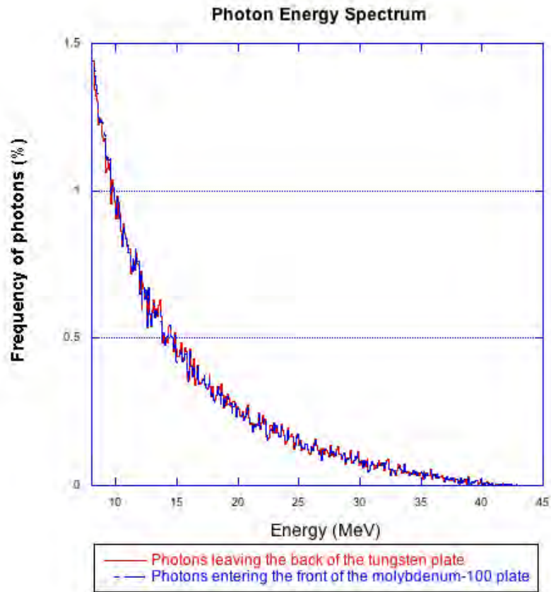
Figure 2.8. Photon energy spectrum for photons leaving the tungsten (red) and entering the molybdenum-100 (blue) for photons above 8 MeV.
