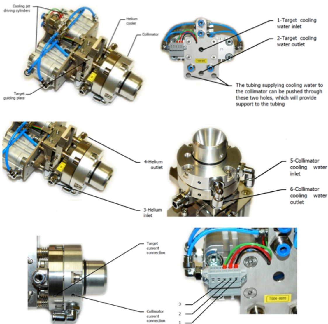
Figure 10. Components of the NIRTA targetry system requiring cooling using a water jet, helium flow and the micro-switch used to load the targets, secure the target, irradiate the target, and drop the target from the system into a pig.
