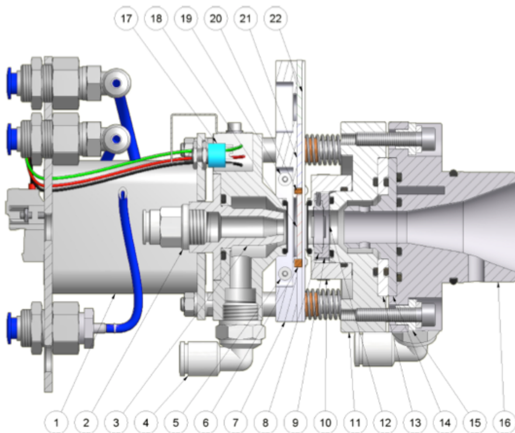
Figure 8. Schematic representation of the NIRTA Targetry system. 1) Pneumatic cylinder driving the cooling jet assembly; 2) Inlet fitting for the cooling water jet; 3) Nozzle for creating the water jet for cooling the back of the target disk; 4) Outlet fitting for the cooling water; 5) Miniature cylinder for driving the locking tongue. 6) Target locking tongue; 7) Target guiding plate; 8) Helium cavity's inner insert. 9) Helium cavity's outer insert. 10) Helium cavity. 11) Connection body. 12) Window foil. 13) PEEK insulator ring. 14) Aluminum extension of the collimator. 15) PEEK insulator insert. 16) Quick connection flange for mounting on cyclotron's extended target ports. 17) Micro-switch. 18) Target disk in irradiation position. 19) Miniature cylinder for driving the intercepting tongue. 20) Intercepting tongue. 21) Second target disk in queue. 22) Third target disk in queue.
