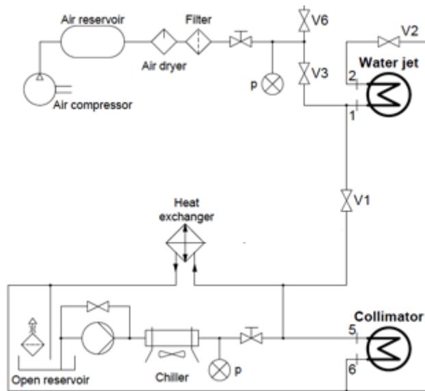
Figure 13. Schematic diagram associated with cooling of the front collimator of the target and the back of the disk using a water jet. The heat exchanger used was again the B3-12A 40 Plate Stainless Steel Heat Exchanger with 1/2" Female NPT Ports Copper Brazed from Dudda Diesel. A chiller was used to cool the water during the whole process. Air was used to purge the system from water in order to clean the back of the target and allow the target disk to drop into the pig.
