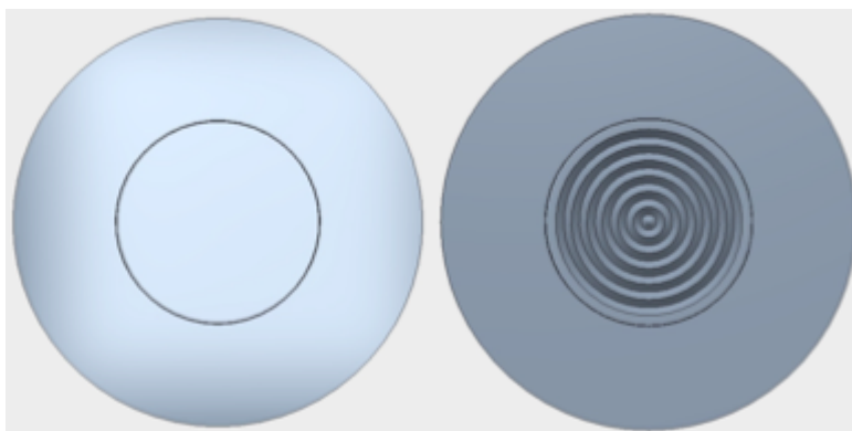
Figure 9. Aluminum target disks used in the NIRTA Solid Targetry System. THE target is the left is used for the production of Zn-62/Cu-62 where a copper disk of 1 cm in diameter is used. The target of the right is used to press TiO 2 or any powder using a high-pressure press. Targets are designed and constructed using a CNC machine using ultra pure aluminum.
