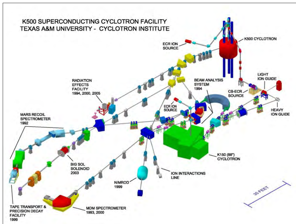
Figure 3. Schematic of K500 superconducting cyclotron facility [40]. The experiments carried out in this research were done at the MDM cave.
