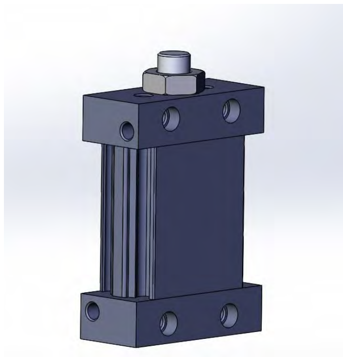
Figure 4.5. Compact actuator MUB series by SMC technologies used to lift the lead shield cover vertically in the transportation shield.
