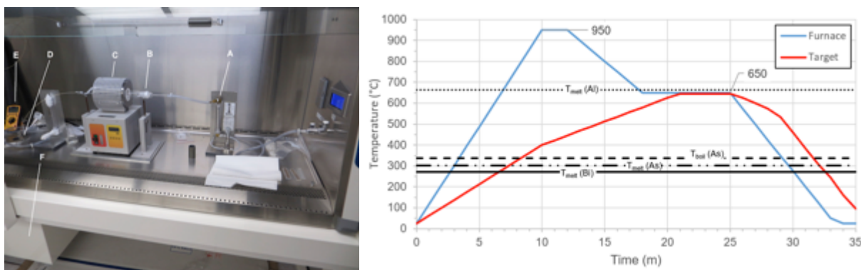
Figure 6. Distillation apparatus for the production of At-211. A) Argon flow meter, b) Quartz tube with crucible. C) Tube furnace. D) Biodex Atom Lab 500 Dose Calibrator to assess the activity of being captured during distillation. E) Temperature monitor. The temperature of the tube furnace and target is given as a function of time showing the corresponding temperature thresholds for melting points for aluminum, bismuth and astatine, and boiling point for astatine. Astatine capture commences immediately after reaching a target temperature of 350 °C and last for approximately 20 min.
