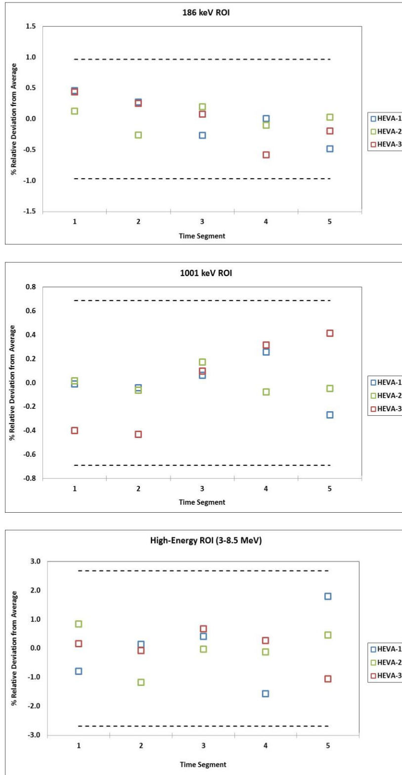
Figure 64. Short-term stability results for a 1.81 wt% cylinder for candidate NDA Fingerprint Signatures for HEVA: HEVA 186 (top), HEVA 1001 (middle) and HEVA NT (bottom). Three-sigma thresholds are shown.
