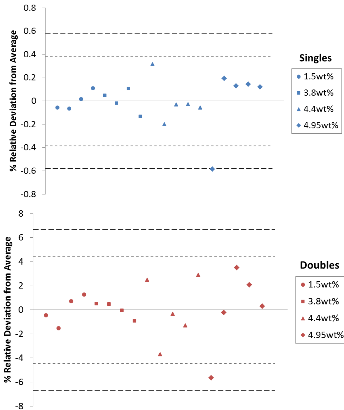
Figure 68. Example NDA Fingerprint results for a series of “inexact replacements” over four cylinders and a total of 18 occupancies for \text{PNEM}_S (top) and \text{PNEM}_D (bottom). Two and three-sigma thresholds are shown.
