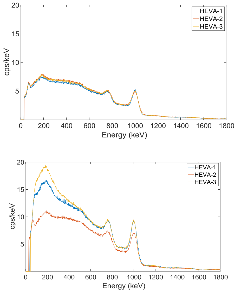
Figure 50. HEVA spectra (from all three modules) for two natural enrichment cylinders producing very different SWC results. Top: cylinder with accurate SWC results for all three HEVA modules. Bottom: cylinder with erroneously high SWC result for HEVA-1 and HEVA-3.
