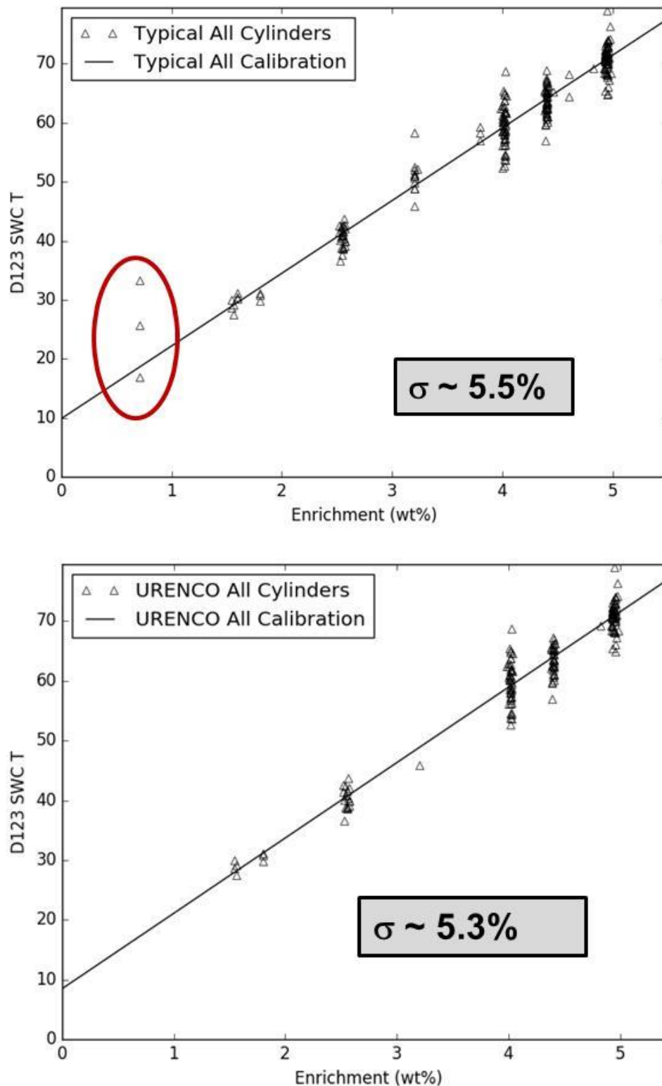
Figure 48. Calibration relationships between the HEVA traditional signature (based on a SWC analysis algorithm) and declared ^{235}\text{U} enrichment for two populations: Typical All (top, 229 cylinders, 226 product) and URENCO All (bottom, 166 cylinders). “D123” is the summed SWC signal from all three HEVA modules.
