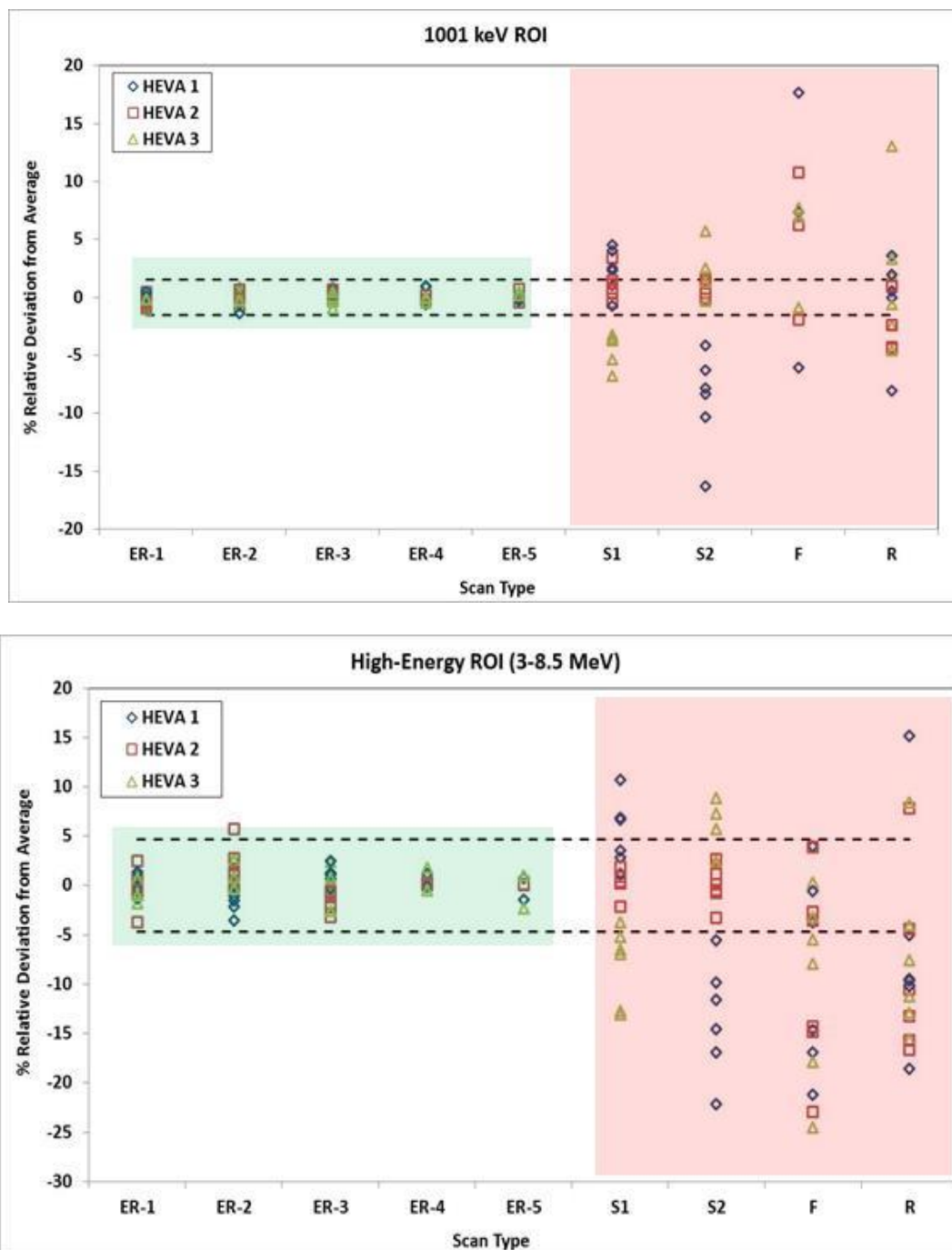
Figure 67. Geometry variation results for candidate NDA Fingerprint Signatures from HEVA, based on five Type 30B cylinders (1.5 wt% to 4.95 wt%): HEVA 1001 (top) and HEVA NT (bottom). Three-sigma thresholds are shown. Some HEVA 1001 data points with very high relative differences are off scale.
