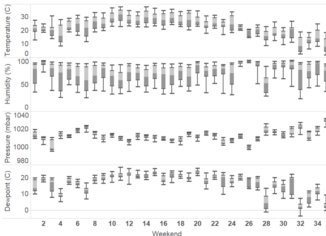
Figure 71. Box-and-whisker plots showing the environmental sensor data over 35 weekends from April to December 2015, based on 30-second measurement intervals.
