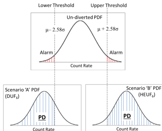
Figure 80. Method of determining PD for diversion of a fixed amount of \text{UF}_6 and false alarm rate for scenarios A and B.
