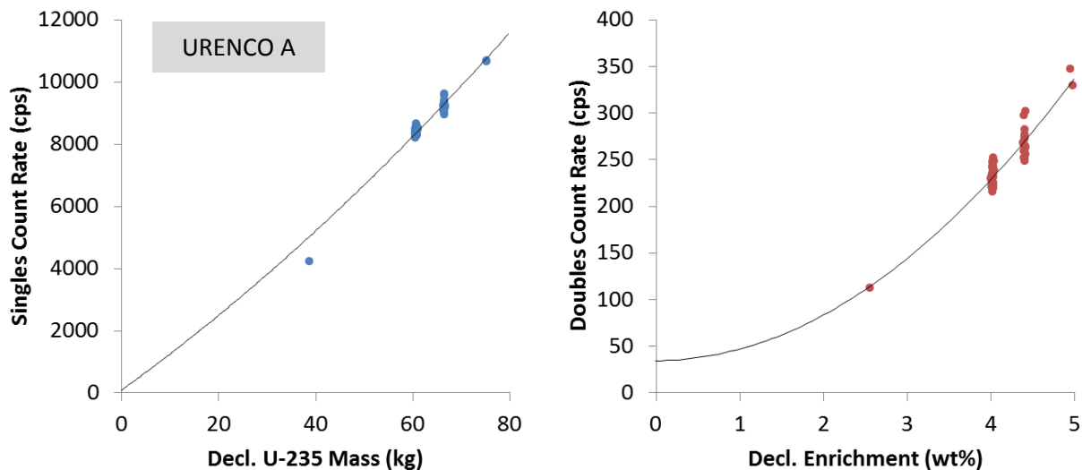
Figure 59. PNEM results showing results for ^{235}\text{U} mass based on the singles count rate (left) and enrichment based on the doubles count rate (right) for the URENCO A population.
