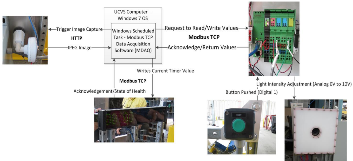
Figure 31. MDAQ Software Interaction Diagram.
