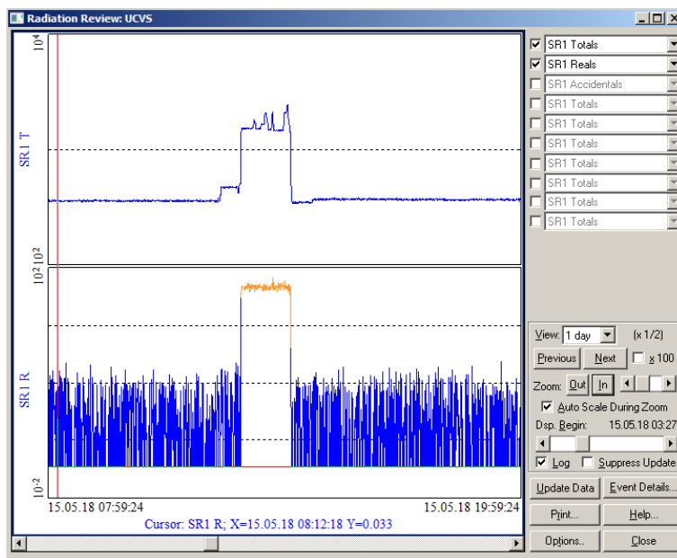
Figure 43. Example of a perturbed occupancy for PNEM identified using the Radiation Review graphical interface.
