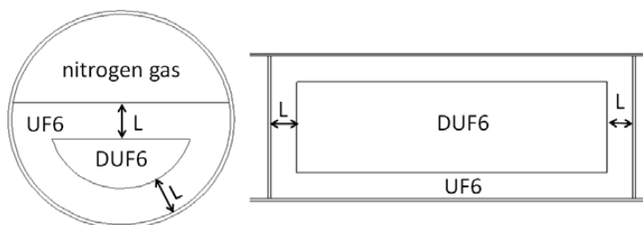
Figure ES. 9. Schematic of diversion scenario in which declared \text{UF}_6 in the center of the cylinder is substituted, in this case with depleted \text{UF}_6 .
