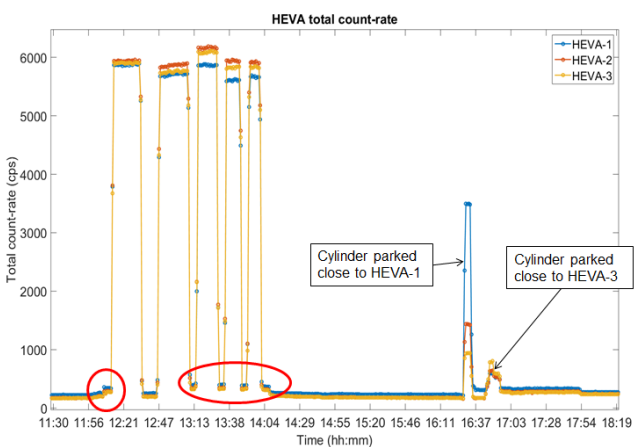
Figure 42. Examples of the HEVA raw data (left) and NGSS imagery used to identify perturbed occupancies. Red circles on the left indicate the effects of a cylinder on the accountancy scale during the UCVS assay.
