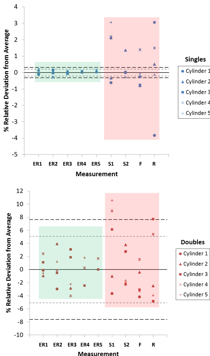
Figure 66. Geometry variation results for candidate NDA Fingerprint Signatures from PNEM, based on five Type 30B cylinders (1.5 wt% to 4.95 wt%): PNEM S (top) and PNEM D (bottom). Two and three-sigma thresholds are shown.
