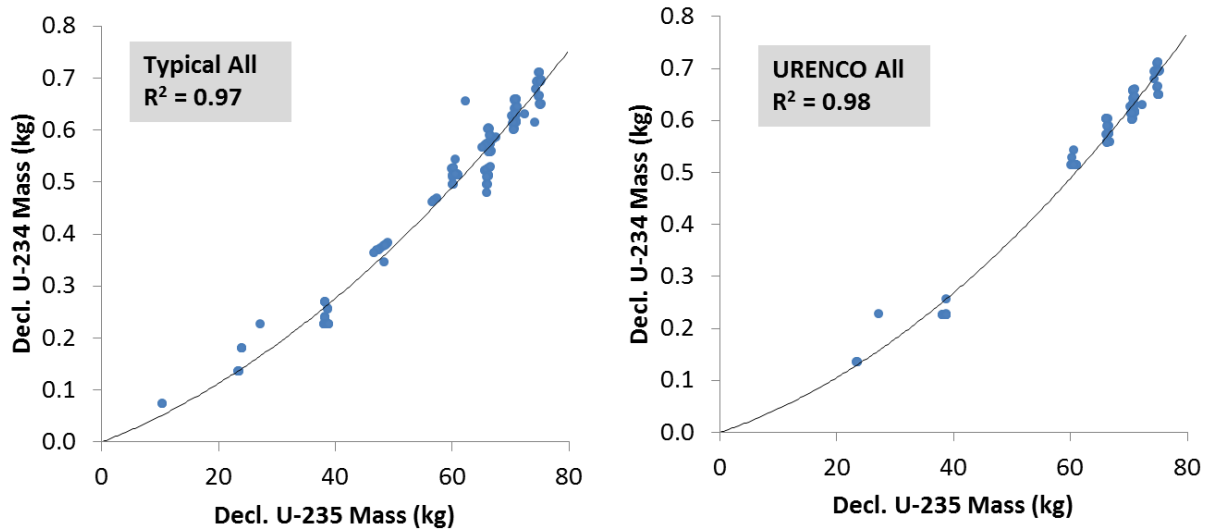
Figure 45. Declared ^{234}\text{U} vs. ^{235}\text{U} values for a subset of the Typical All (left) and URENCO All (right) cylinder populations, and a quadratic fit to those data.
