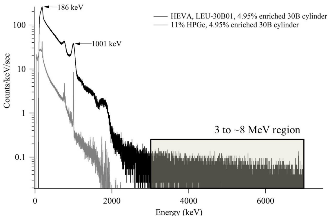
Figure 8. Illustration of the traditional (186-keV and nontraditional (3-8 MeV region corresponding to neutron-induced gamma rays) gamma-ray signatures used by the HEVA method. For comparison, the spectrum from a high-purity germanium (HPGe) spectrometer similar to that used by Euratom and IAEA during inspections, is shown. Note that the high-energy signature is not viable with that smaller, germanium instrument.
