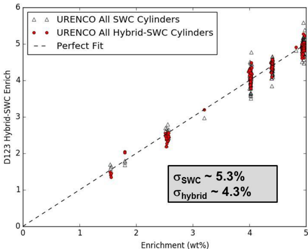
Figure 53. Comparison of hybrid and SWC-based values for ^{235}\text{U} enrichment for the URENCO All population (166 cylinders).
