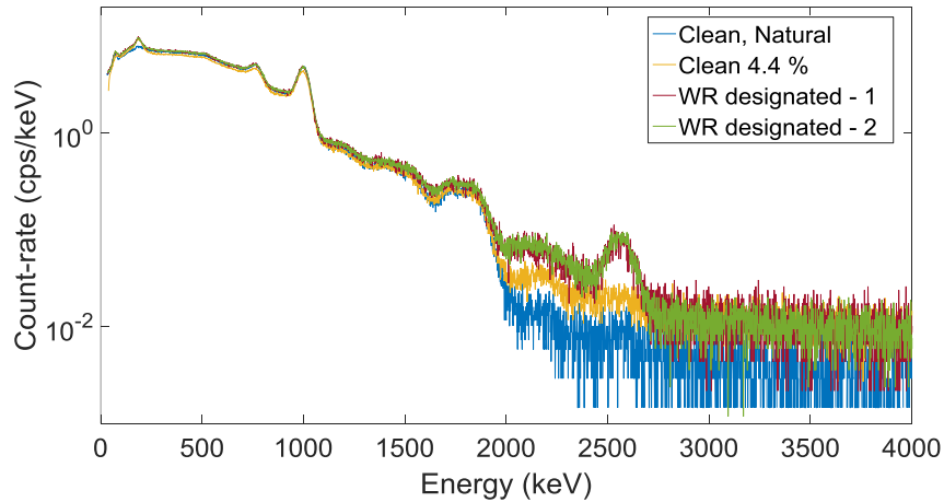
Figure 14. Illustration of variation in 2614-keV signal for cylinders of varying characteristics. WR refers to weapons-recycle material that is expected to contain elevated levels of ^{232}\text{U} .
