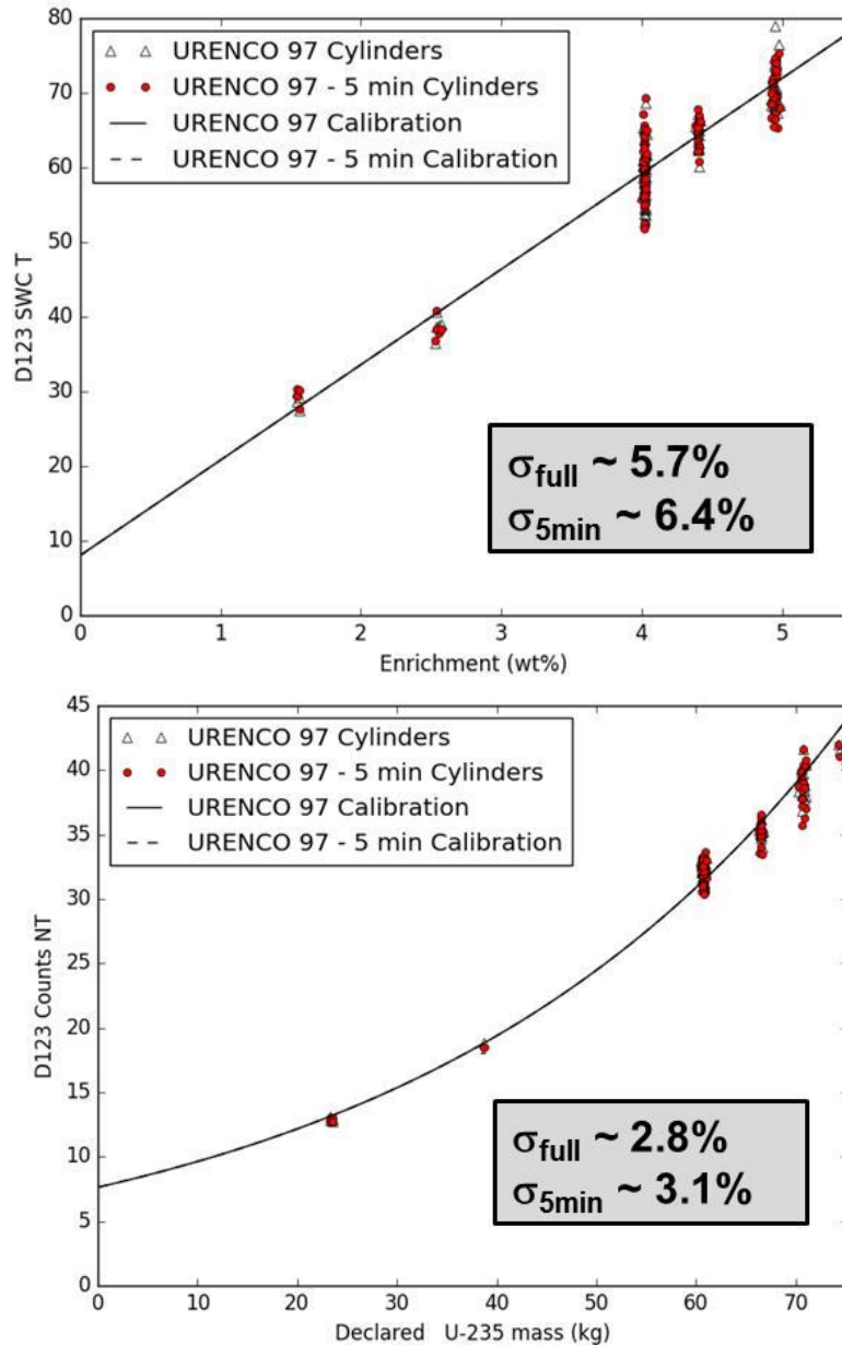
Figure 54. Comparison of HEVA results for full (i.e., variable) and 5-minute occupancy durations for the URENCO 97 (97 cylinders) population. Top: SWC-based values for ^{235}\text{U} enrichment. Bottom: HEVA non-traditional signature for ^{235}\text{U} mass.
