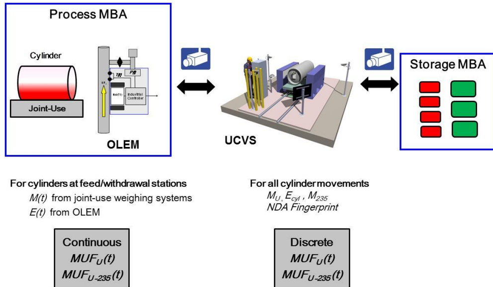
Figure 4. Schematic overview of candidate unattended instrumentation in action including joint-use weighing systems on feed/withdrawal stations, OLEM, and UCVS. Cameras and unattended ID readers provide monitoring of cylinder movements and authenticable cylinder identification.
