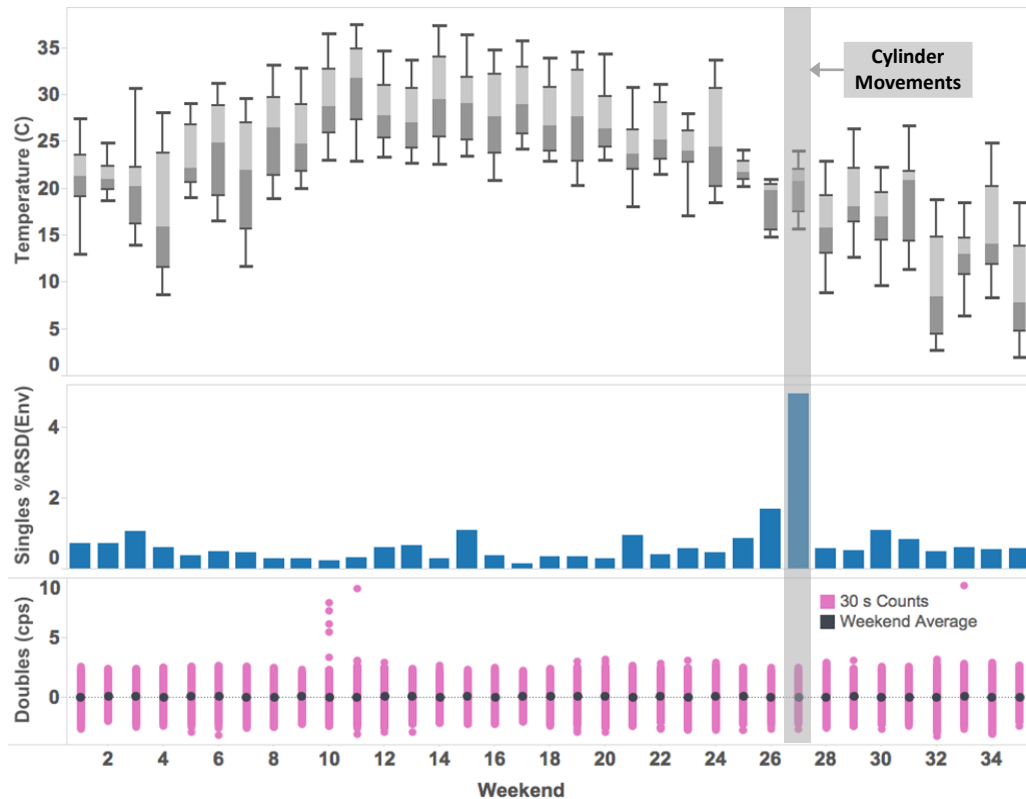
Figure 72. Long-term environmental stability analysis of the PNEM data.
