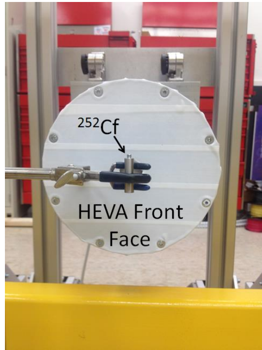
Figure A.1. Experimental configuration for laboratory characterization of a HEVA module in terms of intrinsic neutron efficiency and neutron activation.
