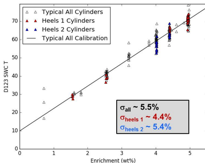
Figure 56. Comparison of SWC-based values for ^{235}\text{U} enrichment for cylinders assayed during the multi-day loading processes for two different trailers loaded with empty cylinders containing heels. The RSD values for the cylinders assayed with heels cylinders nearby are compared to the Typical All value.
