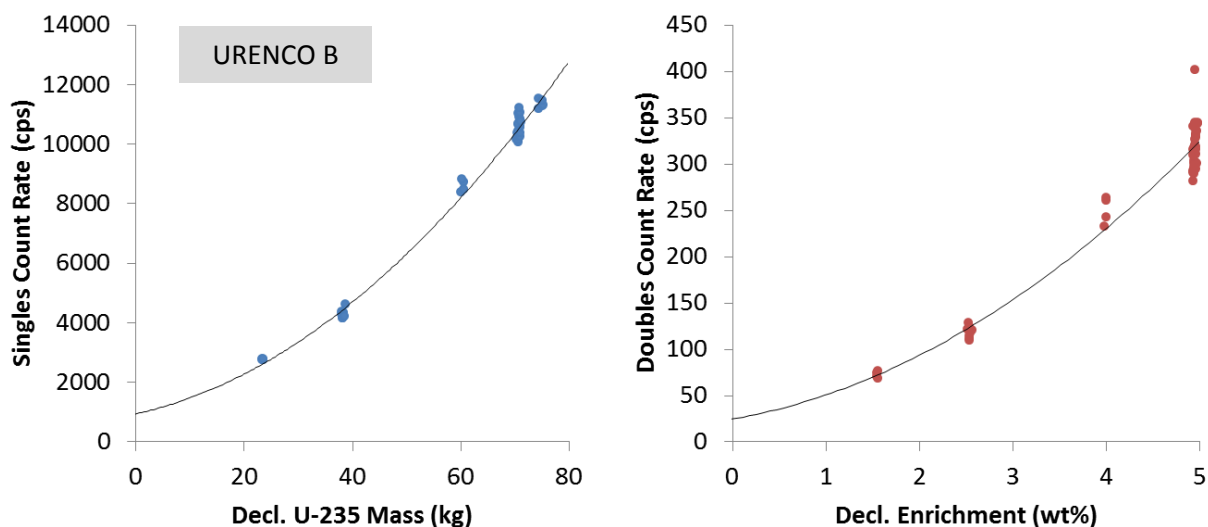
Figure 60. PNEM results showing results for ^{235}\text{U} mass based on the singles count rate (left) and enrichment based on the doubles count rate (right) for the URENCO B population.
