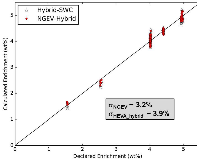
Figure 86. Comparison of NGEV and HEVA hybrid results for the URENCO 97 population.
