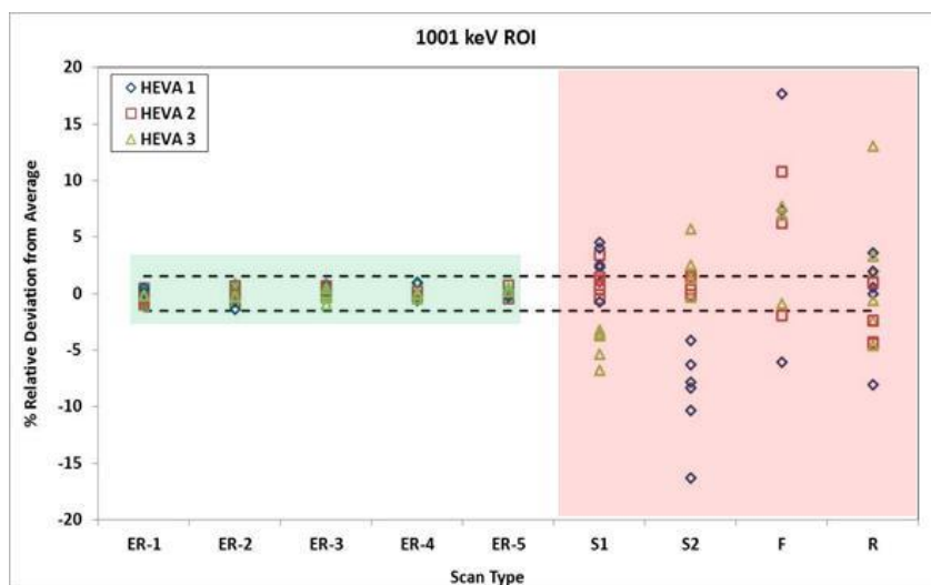
Figure ES. 7. Geometry-sensitivity results for candidate NDA Fingerprint signatures, aggregated over five cylinders for HEVA 1001 . The green box indicates occupancies where the cylinder was consistently positioned on the platform. The red box indicates deliberate geometry changes beyond those expected in routine cylinder handling.
