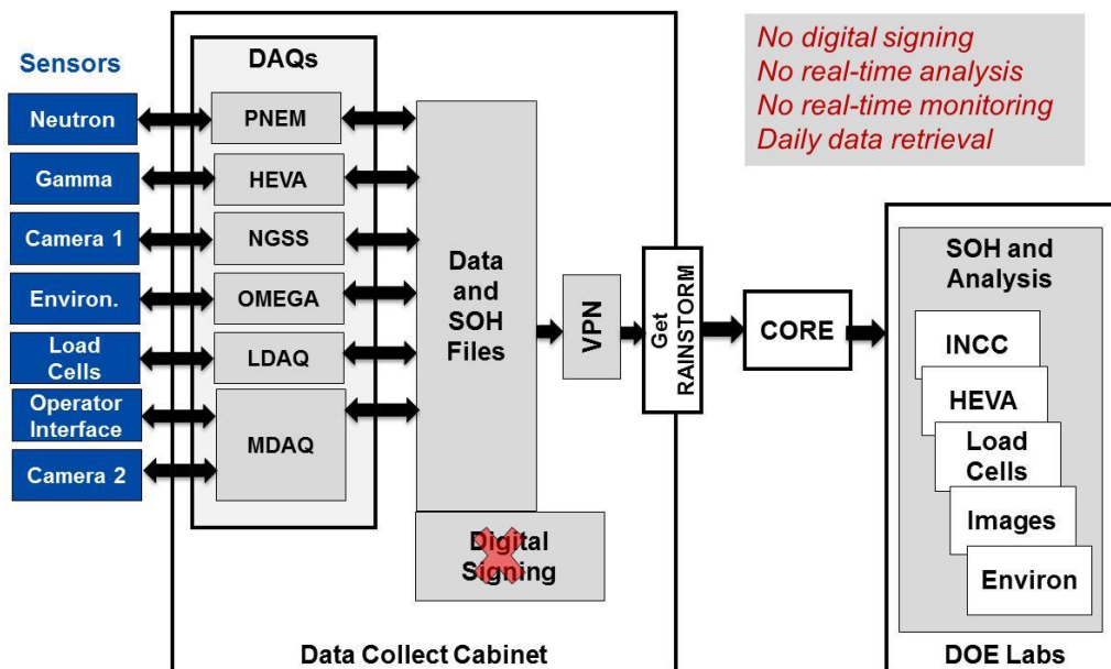
Figure 29. Conceptual schematic of the UCVS software architecture.
