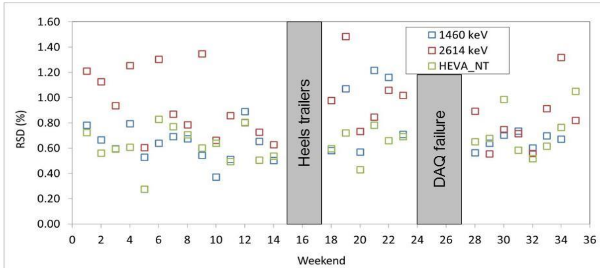
Figure 73. Long-term environmental stability analysis of the HEVA data.
