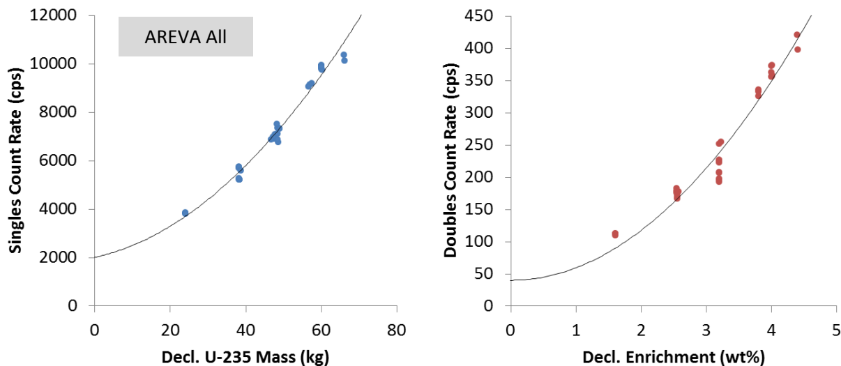
Figure 61. PNEM results showing results for ^{235}\text{U} mass based on the singles count rate (left) and enrichment based on the doubles count rate (right) for the AREVA All population.
