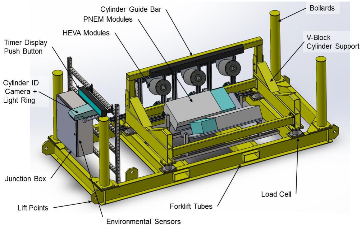
Figure 18. Schematic of the UCVS field prototype hardware design.
