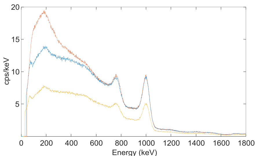
Figure 12. Illustration of the high variability in continuum under the 186-keV peak due to varying levels of wall deposit. All three spectra are from cylinders with enrichment of 0.71 wt%.
