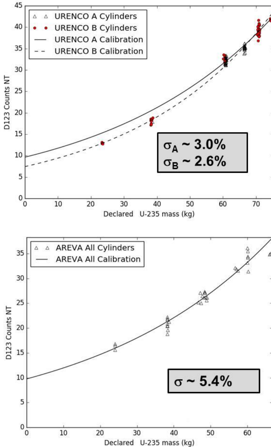
Figure 52. Calibration relationship between the HEVA non-traditional signature (count rate in 3-8 MeV region of interest) and declared ^{235}\text{U} mass for three populations: URENCO A, URENCO USA B (top, 66 and 50 cylinders, respectively), and AREVA All (34 cylinders). “D123” is the sum over all three HEVA modules.
