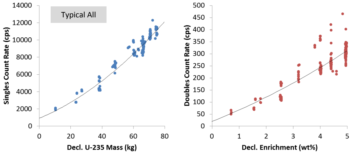
Figure 57. PNEM results showing results for ^{235}\text{U} mass based on the singles count rate (left) and enrichment based on the doubles count rate (right) for the Typical All population.
