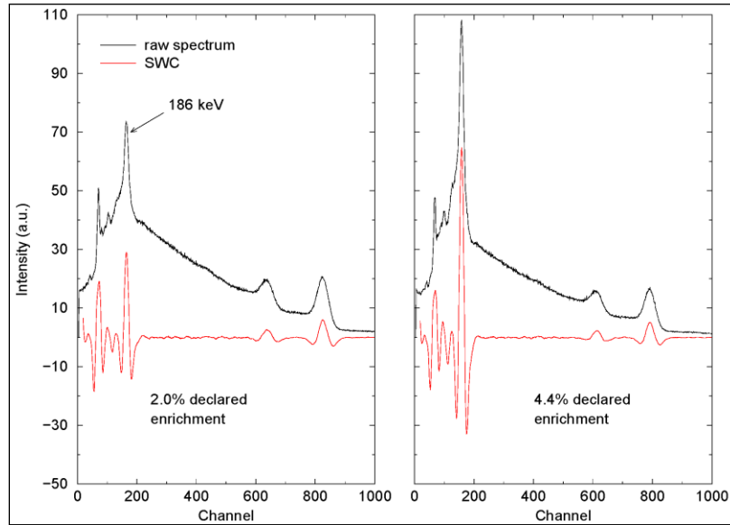
Figure 13. Illustration of the square-wave convolute method on two \text{UF}_6 spectra recorded from Type 30B cylinders with an NaI(Tl) spectrometer.
