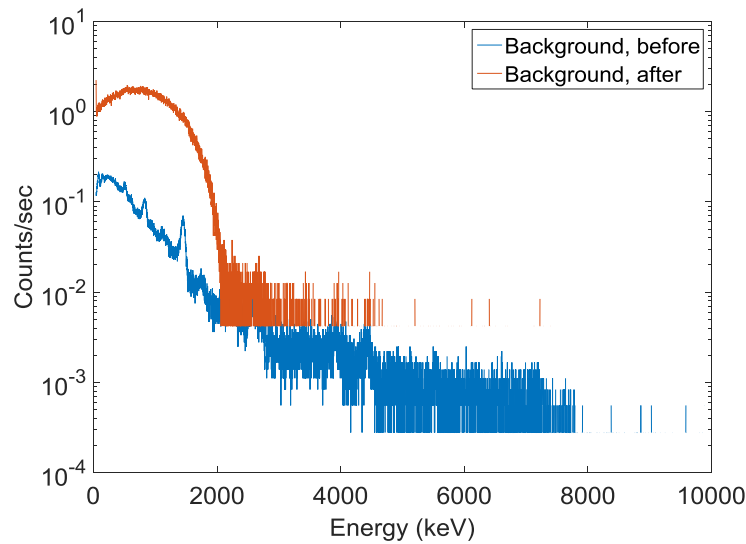
Figure A.3. Background spectra before and after neutron irradiation.
