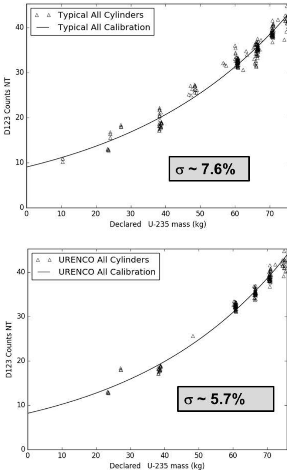
Figure 51. Calibration relationship between the HEVA non-traditional signature (count rate in 3-8 MeV region of interest) and declared ^{235}\text{U} mass for two populations: Typical All (top, 229 cylinders, 226 product) and URENCO All (bottom, 166 cylinders). “D123” is the sum over all three HEVA modules.
