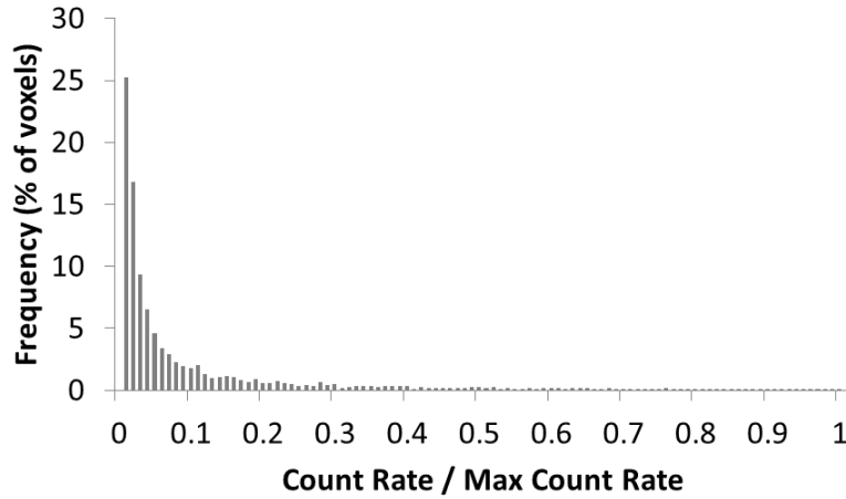
Figure 77. Histogram depicting total neutron signal efficiency map for PNEM 5 .
