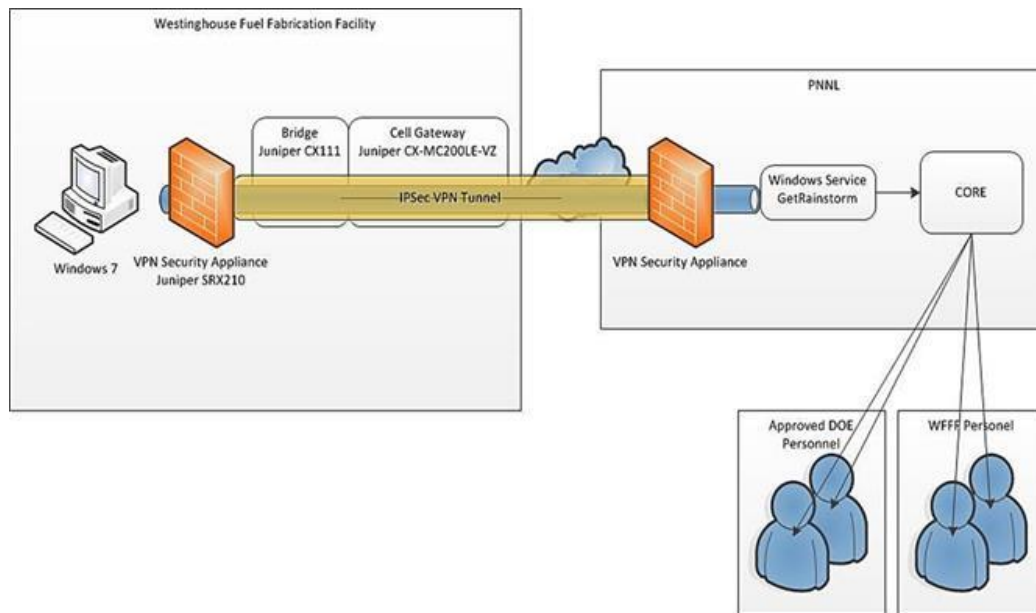
Figure 28. Off-site communication was enabled using a Juniper SRX210 with CX111 bridge and CX-MC200LE-VZ cellular modem.
