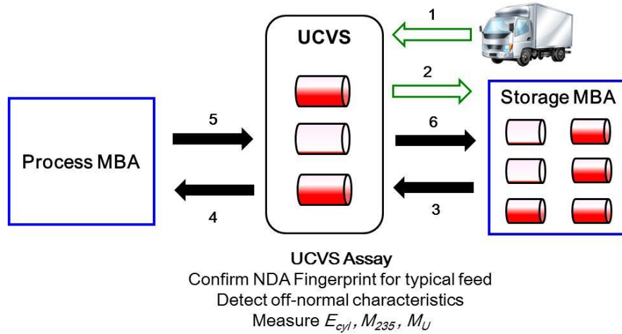
Figure 7. Conceptual overview of how a feed cylinder could be verified using the UCVS, beginning with the receipt of the cylinder from off-site. The six cylinder movements describe, notionally, the life cycle of the cylinder from its acceptance onsite as a full feed cylinder through its entry into the storage MBA as an empty.
