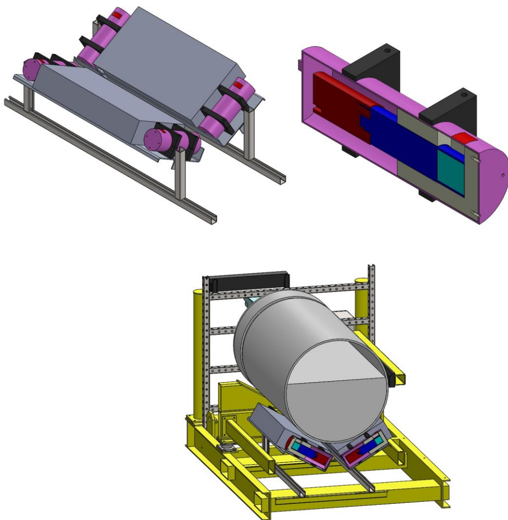
Figure 85. Notional illustration of an NDA method that merges the strengths of PNEM and HEVA to create a new method called Neutron-Gamma Enrichment Verification (NGEV). Top left: ^3\text{He} modules flanked by “side-looking” collimated LaBr spectrometers, with NGEV panels in a clamshell configuration. Top right: Cross-section of the LaBr module showing collimator (grey) and LaBr crystal (light blue). Bottom: Depiction of a UCVS prototype with NGEV modules.
