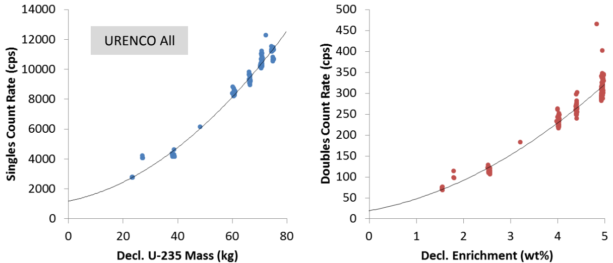
Figure 58. PNEM results showing results for ^{235}\text{U} mass based on the singles count rate (left) and enrichment based on the doubles count rate (right) for the URENCO All population.
