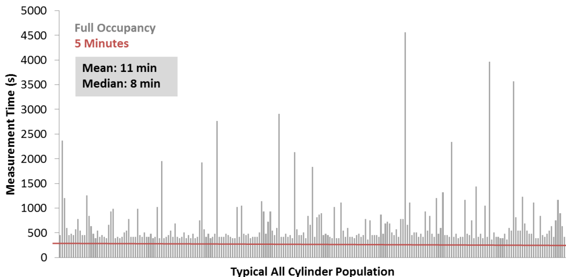
Figure 44. Duration of the 229 occupancies in the Typical All cylinder population, and the associated mean and median values. The UCVS prototype timer was set to 7 minutes; UCVS User Requirements from the IAEA indicate a 5-minute occupancy in a future production-version UCVS.
