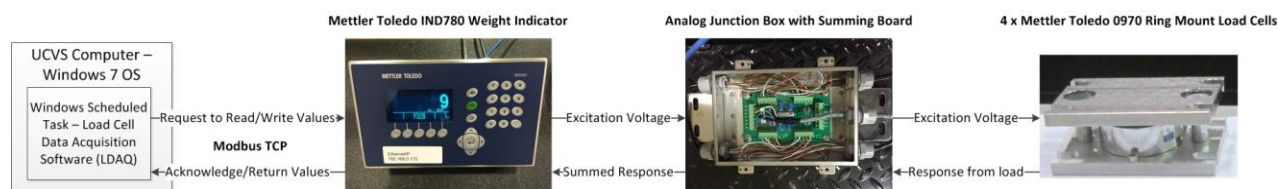
Figure 32. LDAQ Software Application Interaction Diagram.
