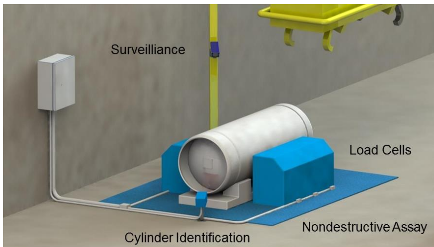
Figure ES. 1. Conceptual design of an integrated UCVS that includes unattended NDA instrumentation (blue panels), camera surveillance, and cylinder identification technology.
