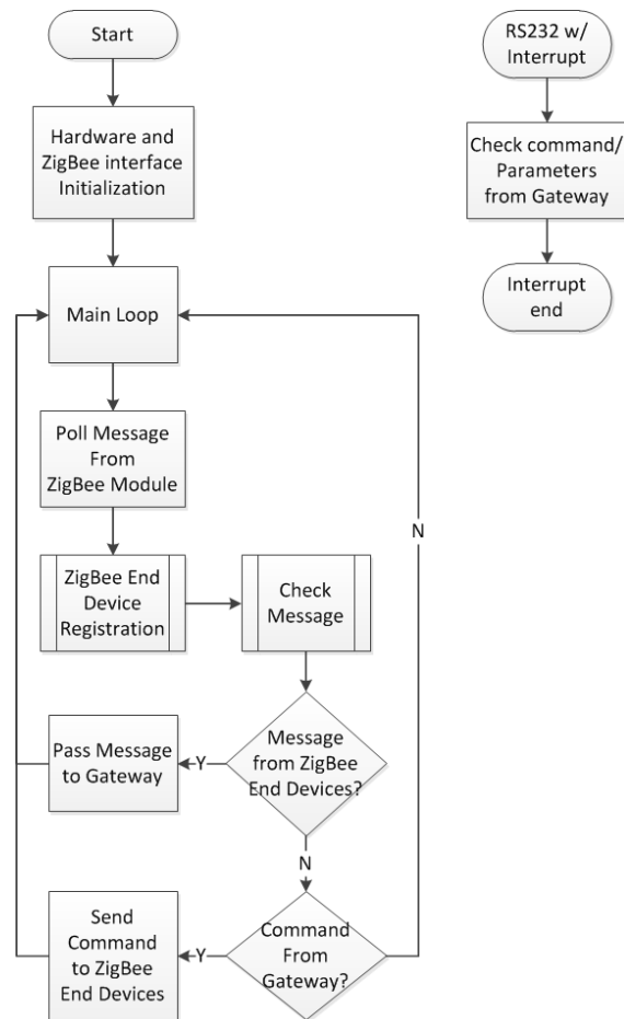
Fig. 13: ZigBee coordinator firmware flow
