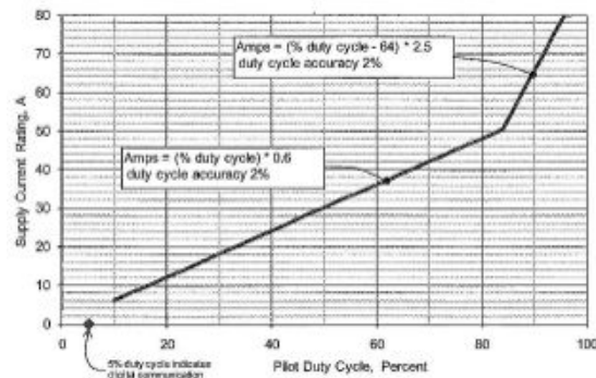
Fig. 5: Supply current v.s. pilot duty cycle[12]
