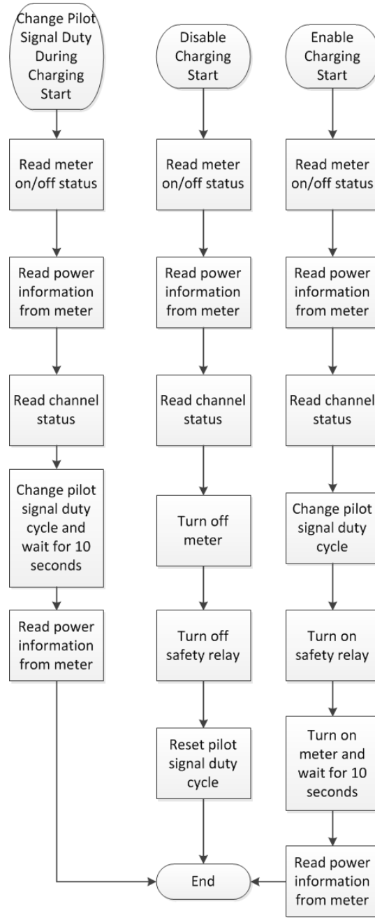
Fig. 14: Server operation flow
