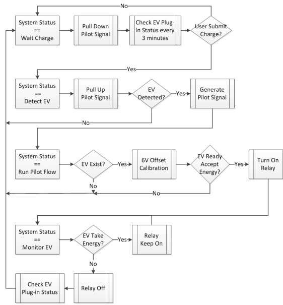
Fig. 9: State machine flow chart
