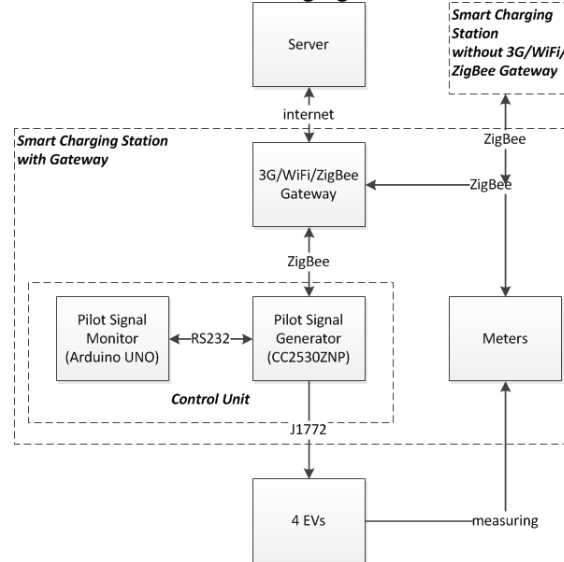
Fig. 2: Details of smart charging station
