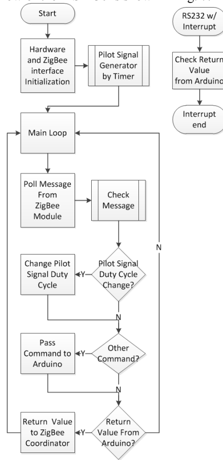
Fig. 7: Firmware flow of MSP430 of CC2530ZNP as the ZigBee end device (pilot signal generator)
