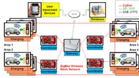
Fig. 1: Smart charging infrastructure
