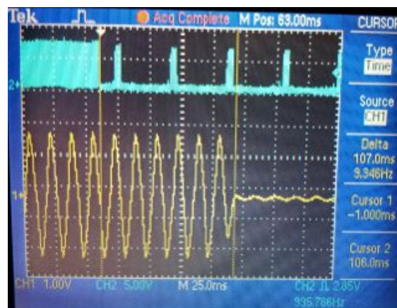
Fig. 19 From 12A to 0A
