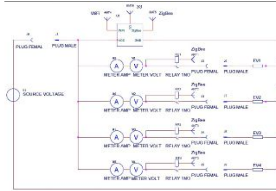
Fig. 3: Schematics of metering system
