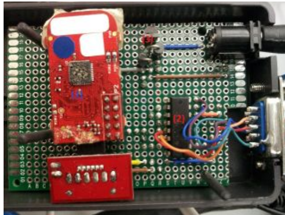
Fig. 12: ZigBee coordinator implementation: (1) ZigBee CC2530ZNP (2) MAX3232
