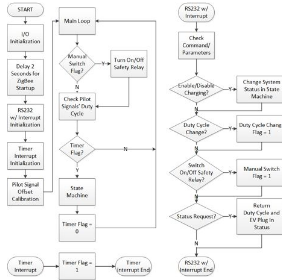
Fig. 8 Pilot signal monitor firmware flow chart
