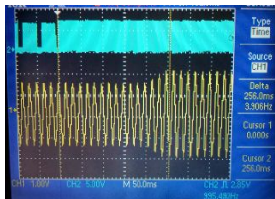
Fig. 20 From 8A to 12A
