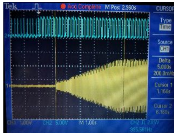
Fig. 18: From 0A to 12A
