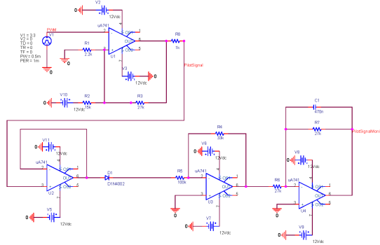
Fig. 10: Peripheral circuit simulation schematics
