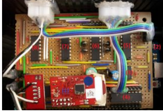
Fig. 6: Realization of the control unit: (1)pilot signal generator (2)pilot signal monitor (3)555 counter (4)relay driver (5)Schmitt trigger (6)unit gain buffer (7)inverting amplifier (8)inverting LPF
