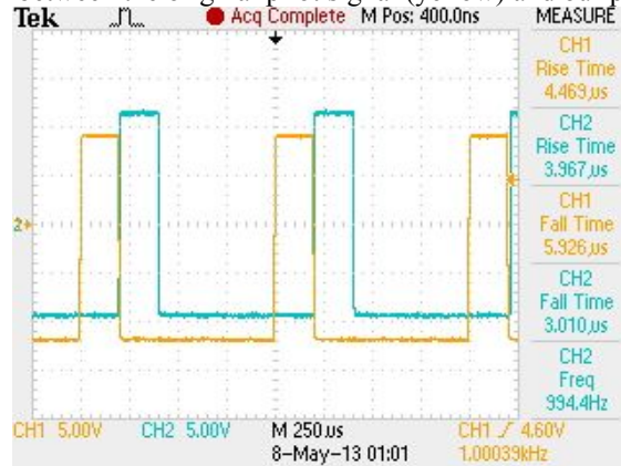
Fig. 17: Comparison between our pilot signal and original pilot signal
