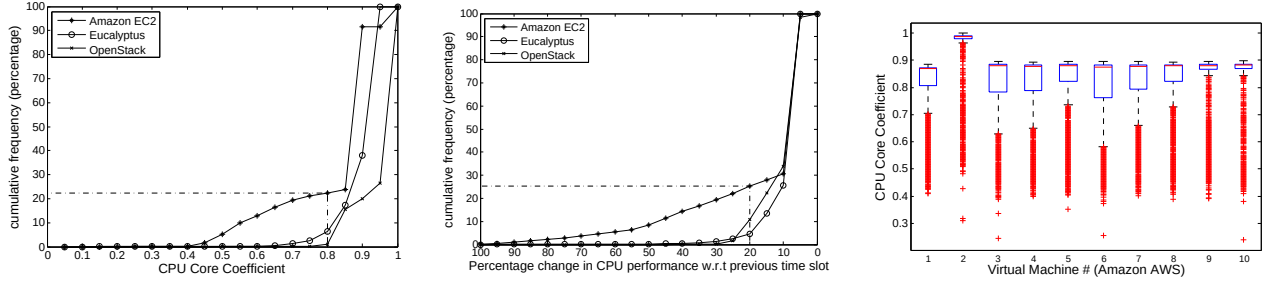
(a) Cumulative Distribution Function (CDF) of normalized CPU Core performance, across VMs previous measurement time-slot and over time. (b) CDF of performance variation relative to normalized CPU Core performance, across VMs previous measurement time-slot and over time. (c) Box-and-Whiskers plot of normalized performance distribution over time (Y axis) and for different Amazon AWS VMs (X axis).
