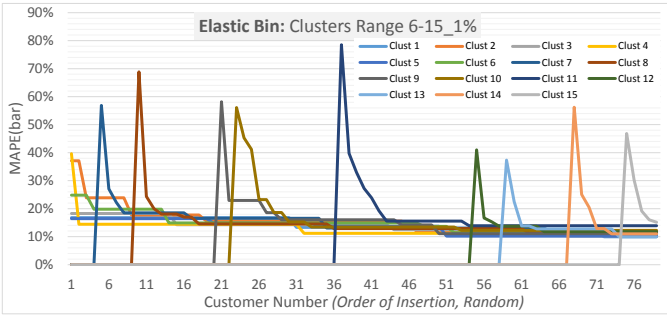
(a) Incremental reduction in MAPE as each new customer is from among 6 clusters, initially, and among 15 cluster finally. Spikes indicate a new cluster is created.
