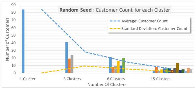
(c) # of customers in each cluster (bar). Experiments run with different numbers of clusters: 1, 3, 6 and 15. Average and Std. Deviation of # of customers per cluster (line) is also shown.
