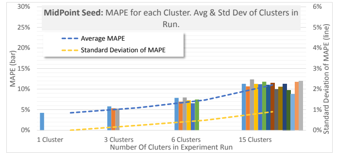
(b) MAPE for each cluster (bar) when using customer's KWh as the ordering for midpoint selection. Results for different numbers of clusters, and their Average and Std. Deviation of MAPE (line) are shown.
