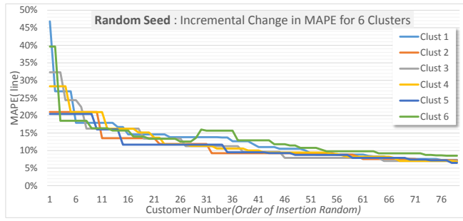
(a) Incremental reduction in MAPE as each new customer is added across 6 clusters
