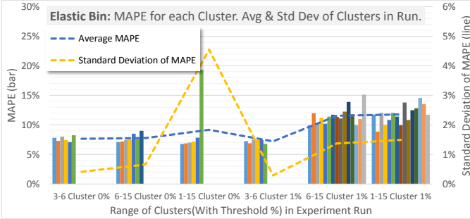
(b) MAPE for each cluster (bar) for elastic numbers of clusters. Results for different numbers of cluster upper and lower bounds, along with thresholds, as well as their Average and Std. Deviation of MAPE (line) are shown.
