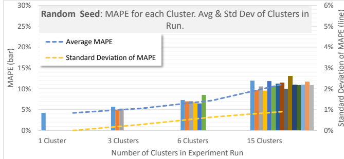
(b) MAPE for each cluster (bar). Experiment is run with different numbers of clusters: 1, 3, 6 & 15. Average and Std. Deviation of MAPE (line) for each clusters is also shown.
