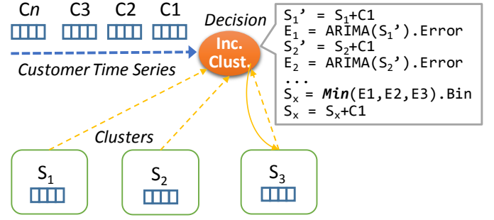
Figure 2. Incremental Clustering Approach for Energy Consumption Time Series Data. The Min function calculates the affinity score.
