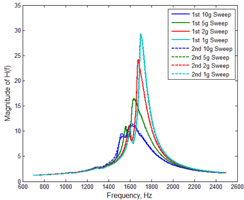
Fig. 4 Transfer functions for a specimen preloaded to 3110 N through foam and cylinder, assembly 3
