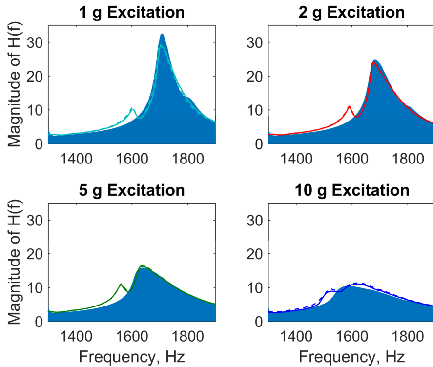
Fig. 10 Comparison of experimental transfer functions and simulated sine sweeps from 10g to 1g
