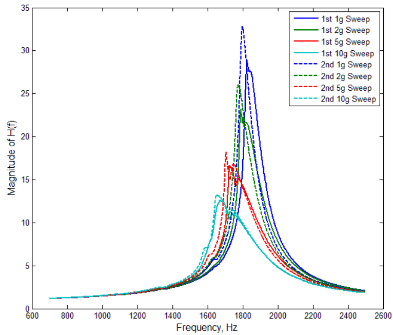
Fig. 2 Transfer functions for a specimen preloaded to 3110 N through foam and cylinder, assembly 1
