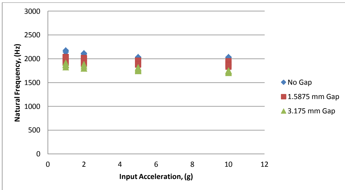
Fig. 6 Distribution of natural frequency per gap size with a 3110 N preload through the cylinder only
