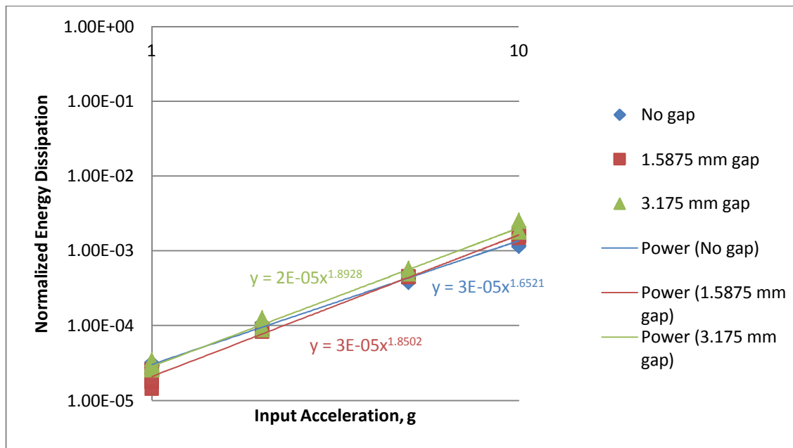
Fig. 7 Distribution of normalized energy dissipation per gap size with a 3110 N preload through the foam and cylinder
