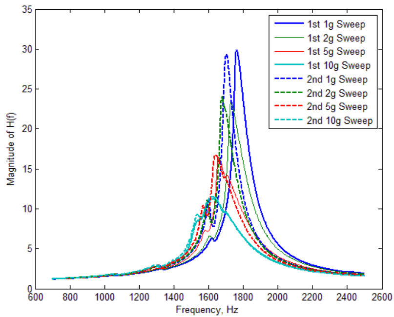
Fig. 3 Transfer functions for a specimen preloaded to 3110 N through foam and cylinder, assembly 2
