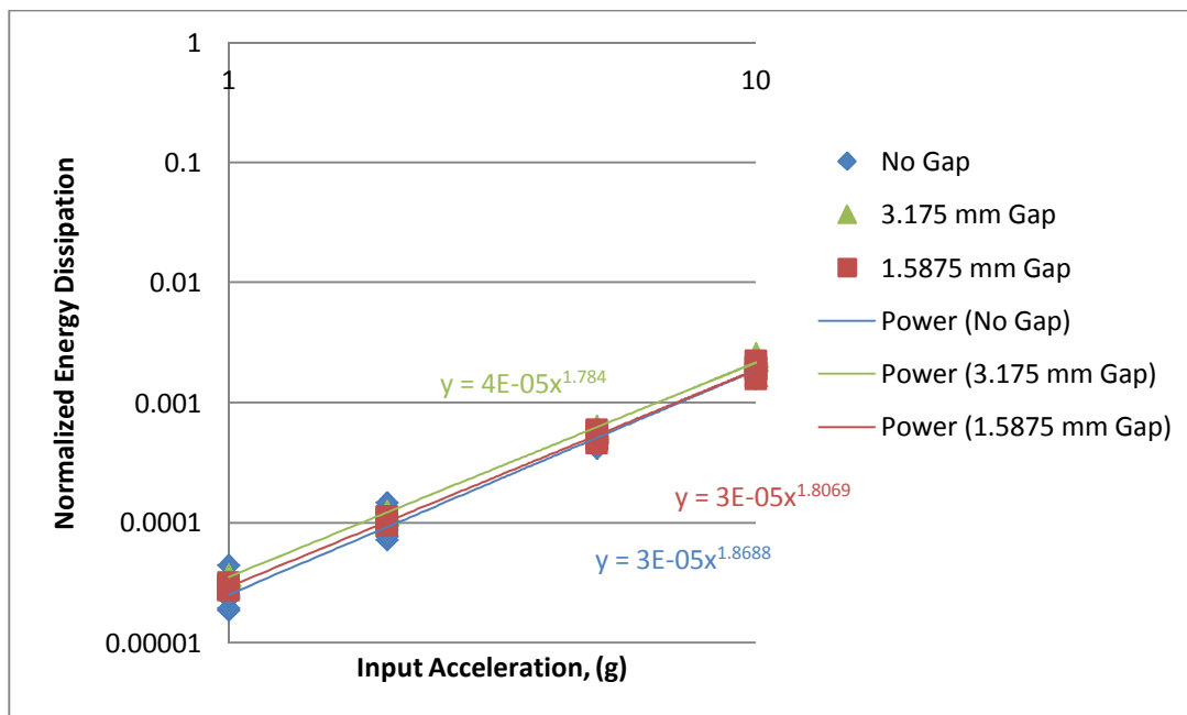
Fig. 8 Distribution of normalized energy dissipation per gap size with a 3110 N preload through the cylinder only
