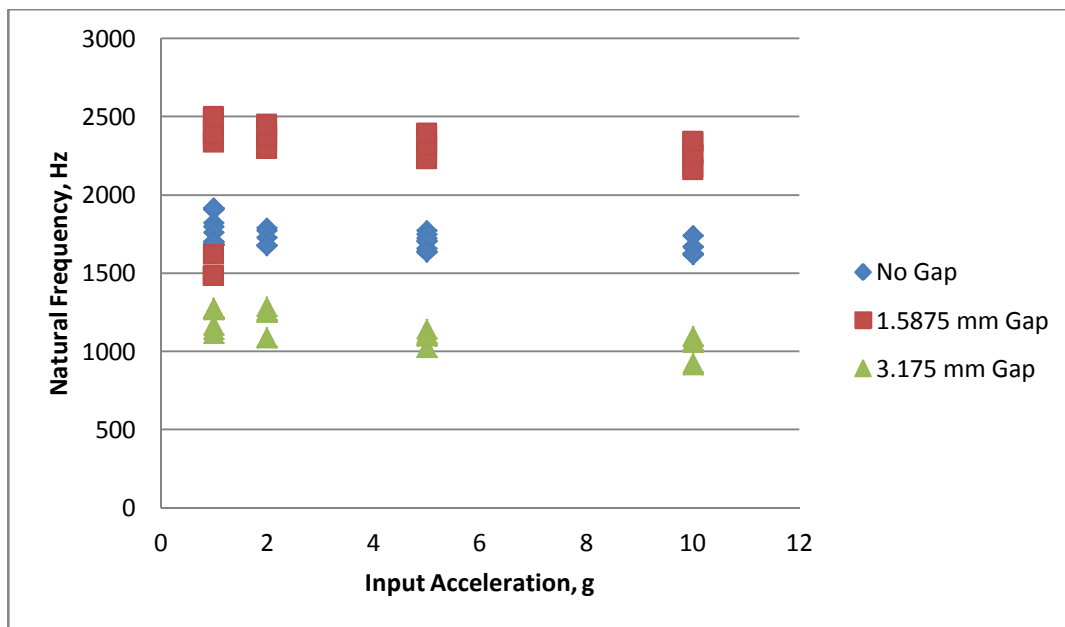
Fig. 5 Distribution of natural frequency per gap size with a 3110 N preload through the foam and cylinder
