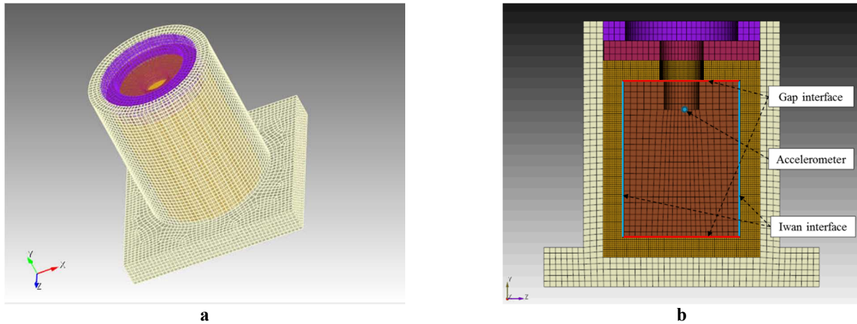
Fig. 9 (a) Finite element model of Ministack, (b) solid mass to foam interface
