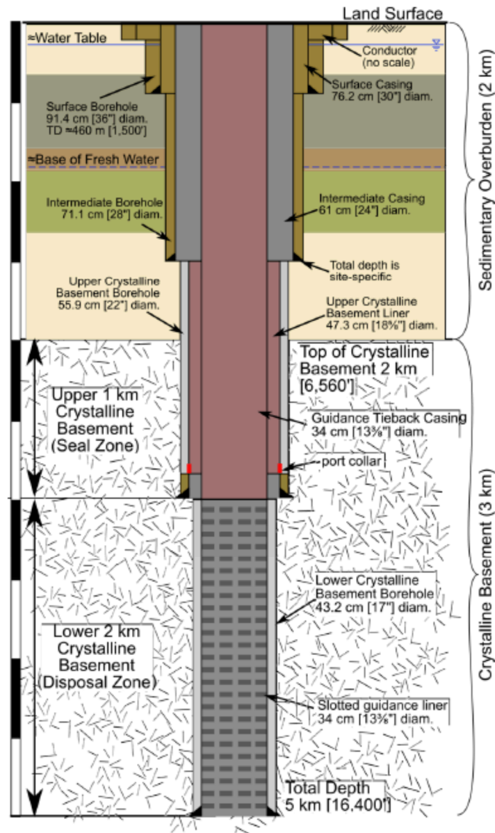
Figure 2 DBFT Conceptual Design (Kuhlman, K.L., et al, 2015)
