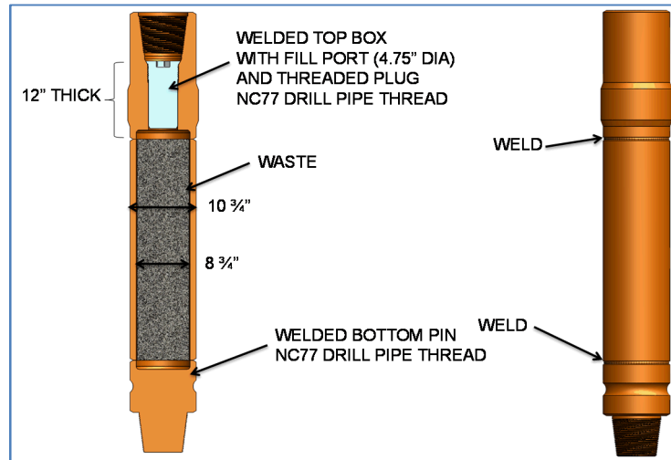
Figure 3. 27.3-cm (10.75-inch) OD flask-type design, aspect ratio shortened for illustration (Su and Hardin 2015)
