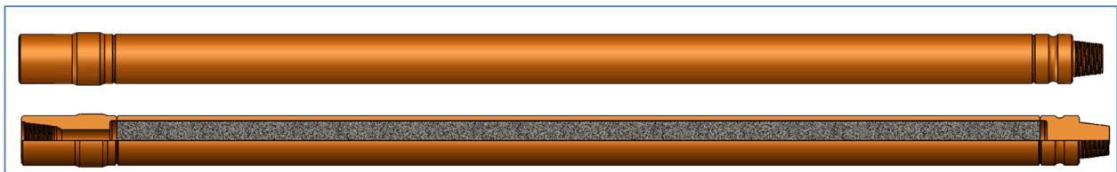
Figure 4. 27.3-inch OD flask-type design, shown at true aspect ratio (Su and Hardin 2015)
