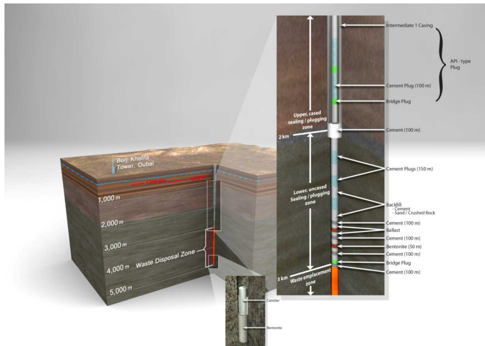
Figure 1. Conceptual design of DBD of radioactive waste. The dashed blue line indicates typical lower extent of useable fresh groundwater resources (from Hardin, 2015)
