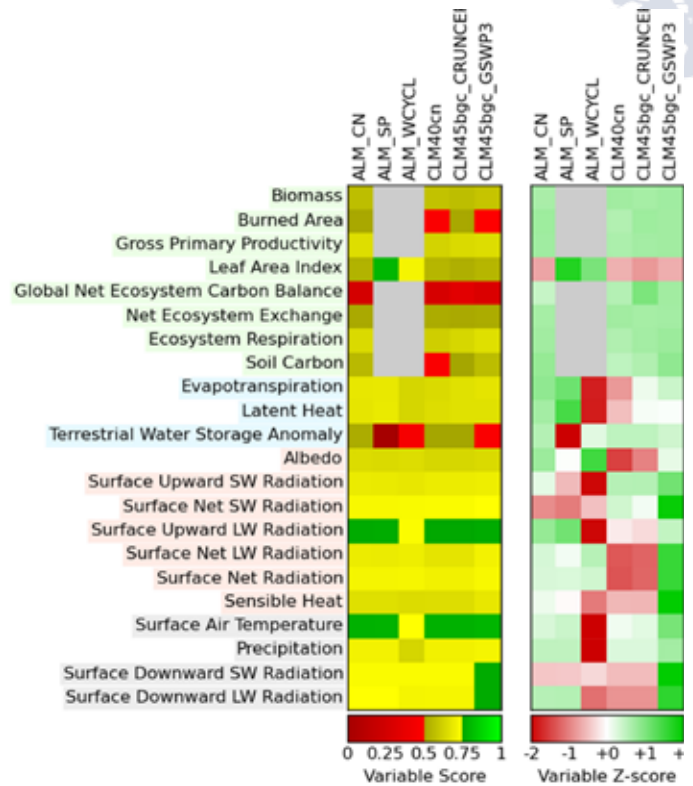
Figure 2.1. The ILAMBv2 package produces a summary graphic depicting model performance across a wide variety of variables, emphasizing absolute performance (left) as well as relative performance (right) with respect to comparisons with observations. This figure compares results from the ACME Land Model (ALM) run offline with carbon–nitrogen (CN) biogeochemistry (ALM_CN), run offline in satellite phenology (SP) mode (ALM_SP), and fully coupled in SP mode (ALM_WCYCL) with the Community Land Model (CLM) run offline for CLM-4.0 (CLM40cn), for CLM-4.5-BGC (CLM45bgc_CRUNCEP) and for CLM-4.5-BGC with Global Soil Wetness Project version 3 (GSWP3) forcing (CLM45bgc_GSWP3). (image to the right)
