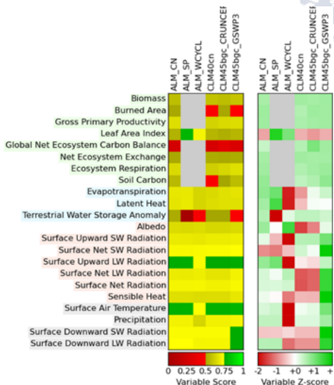
Figure 3.3. The ILAMBv2 package produces a summary graphic depicting model performance across a wide variety of variables, emphasizing absolute performance (left) as well as relative performance (right) with respect to comparisons with observations. This figure compares results from the ACME Land Model (ALM) run offline with carbon–nitrogen (CN) biogeochemistry (ALM_CN), run offline in satellite phenology (SP) mode (ALM_SP), and fully coupled in SP mode (ALM_WCYCL) with the Community Land Model (CLM) run offline for CLM-4.0 (CLM40cn), for CLM-4.5-BGC (CLM45bgc_CRUNCEP) and for CLM-4.5-BGC with Global Soil Wetness Project version 3 (GSWP3) forcing (CLM45bgc_GSWP3).
