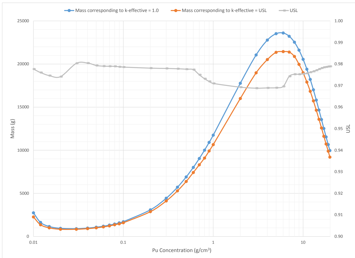
Figure 1. Pu critical mass and USL-mass for water-moderated plutonium bare spheres
